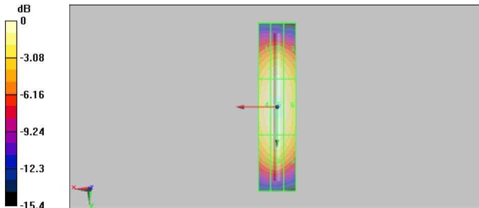
0 dB = 0.499A/m
