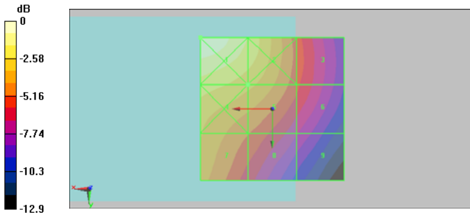
0 dB = 0.277A/m
