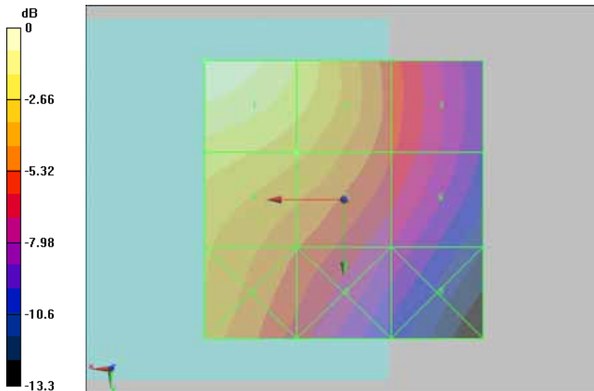
0 dB = 0.283A/m
