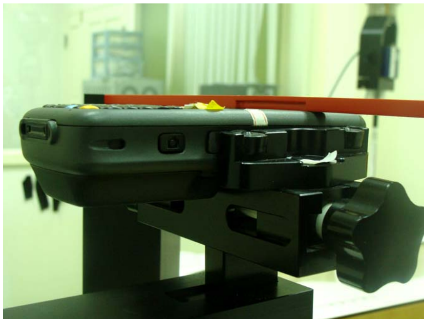
DUT with Battery 2 - Left Side View
