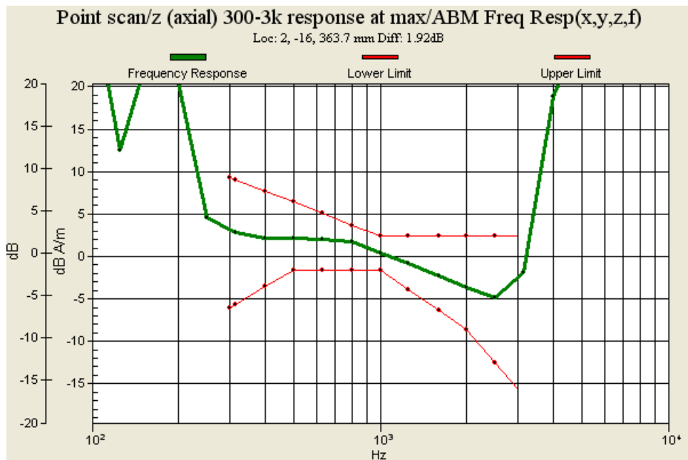
Fig. 9.6: Frequency Response of GSM1900 Ch810
