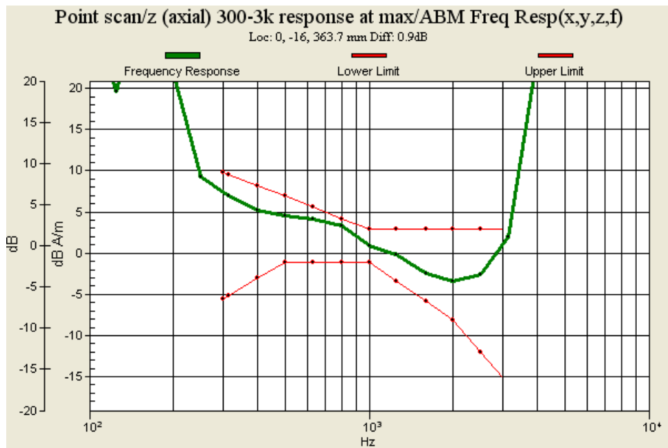
Fig. 9.12: Frequency Response of WCDMA Band II Ch9538
