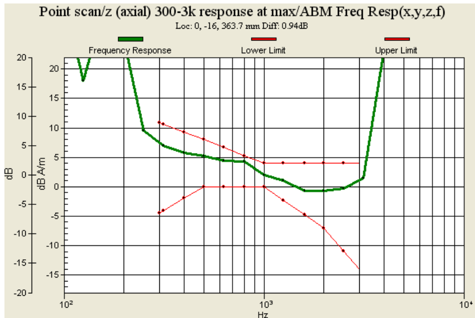
Fig. 9.2: Frequency Response of GSM850 Ch189
