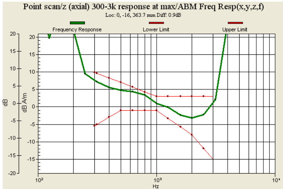
Fig. 9.11: Frequency Response of WCDMA Band II Ch9400
