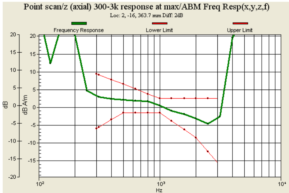
Fig. 9.5: Frequency Response of GSM1900 Ch661
