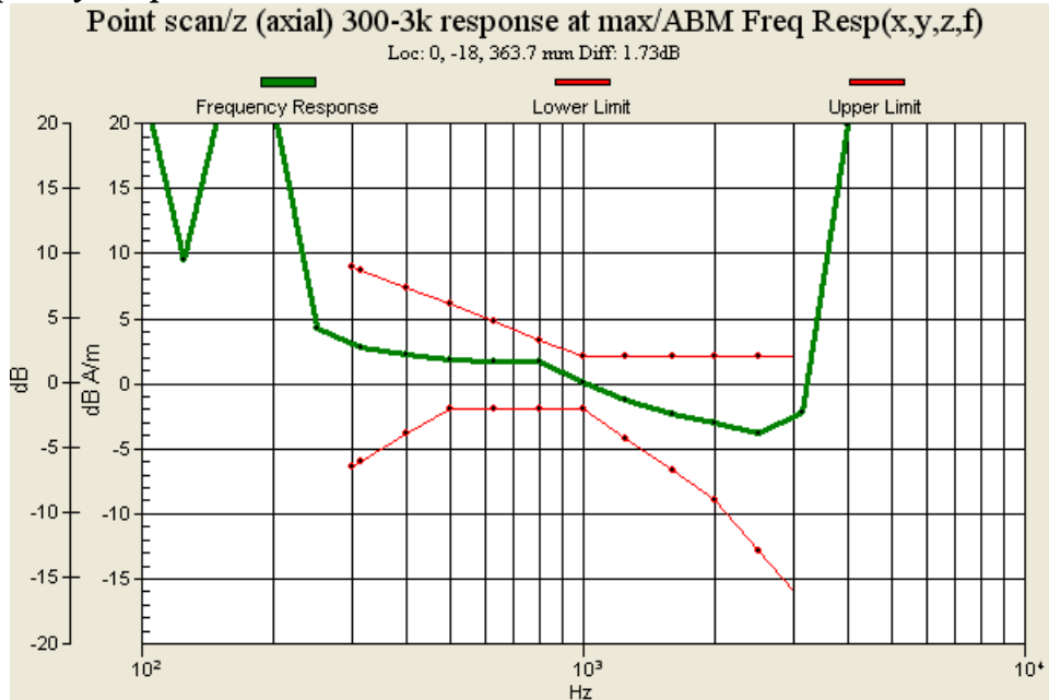
Fig. 9.1: Frequency Response of GSM850 Ch128
