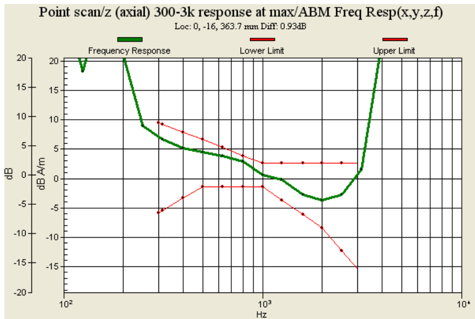
Fig. 9.8: Frequency Response of WCDMA Band V Ch4182
