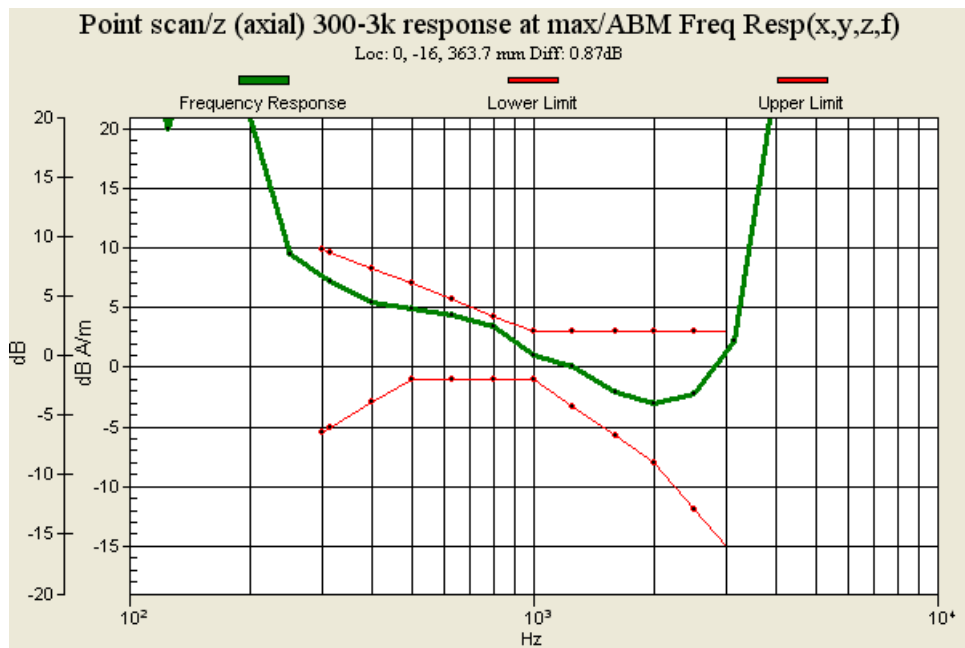
Fig. 9.10: Frequency Response of WCDMA Band II Ch9262
