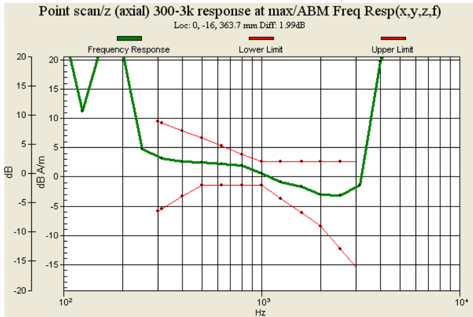
Fig. 9.3: Frequency Response of GSM850 Ch251
