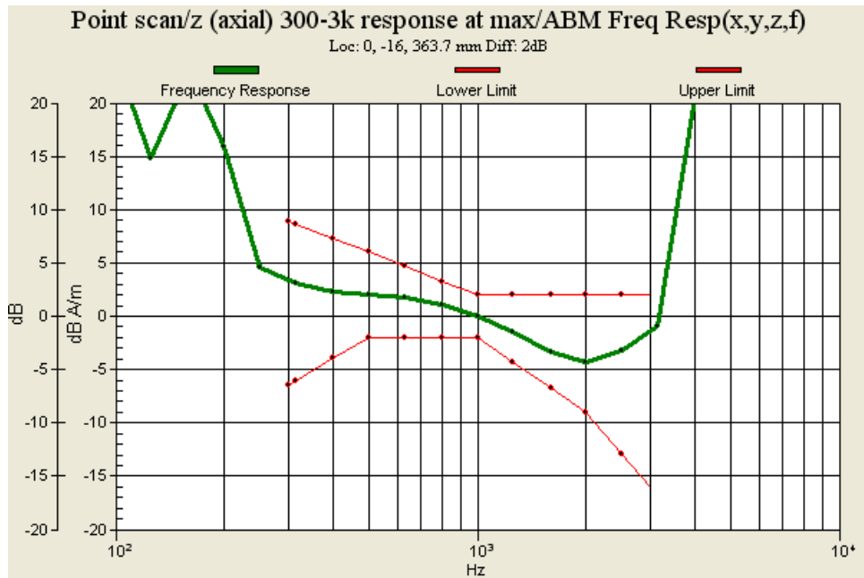
Fig. 9.7: Frequency Response of WCDMA Band V Ch4132
