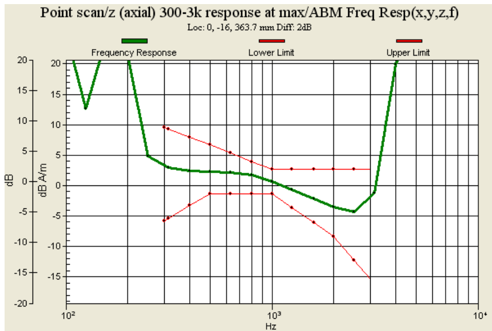
Fig. 9.4: Frequency Response of GSM1900 Ch512
