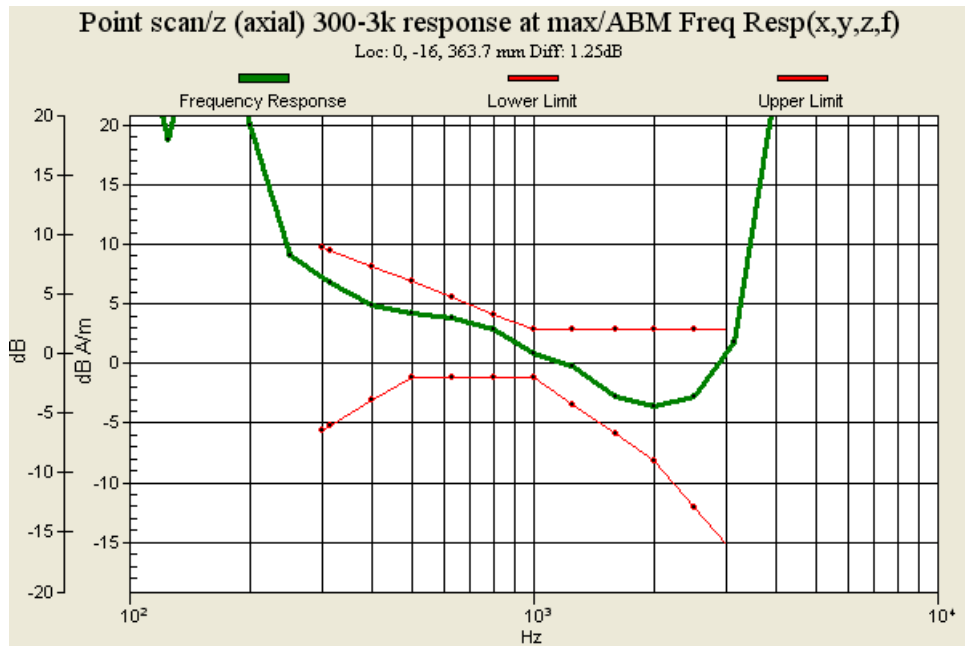
Fig. 9.9: Frequency Response of WCDMA Band V Ch4233
