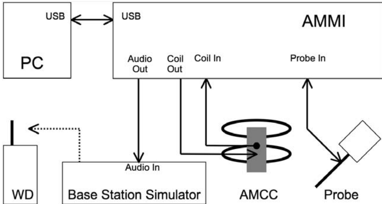
Fig. 5.6: T-Coil setup cabling
