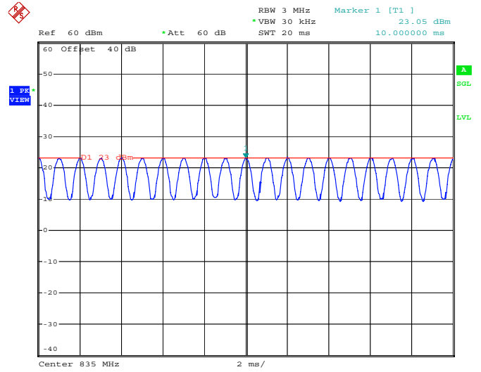
835MHz - 80% AM
