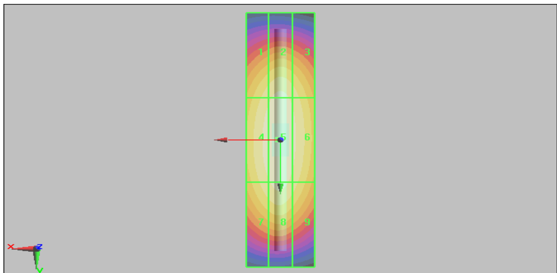
0 dB = 0.546A/m
