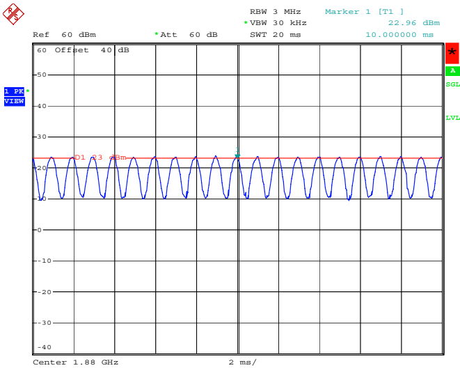
1880MHz - 80% AM
