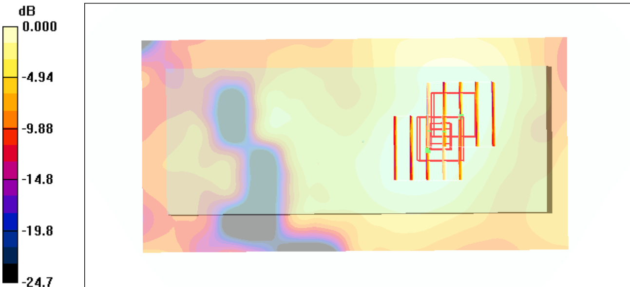
0 dB = 0.019mW/g
