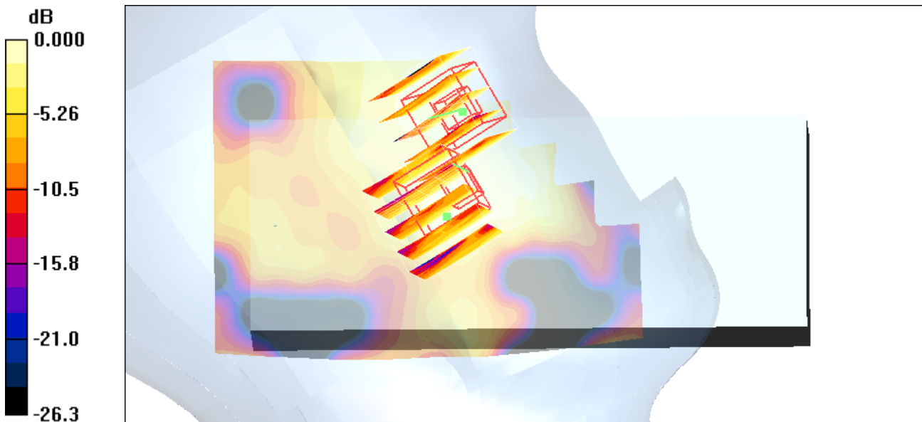
0 dB = 0.012mW/g
