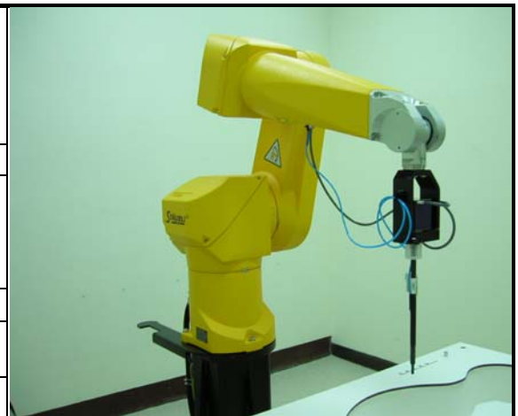
Fig. 5.2 Probe Setup on Robot
