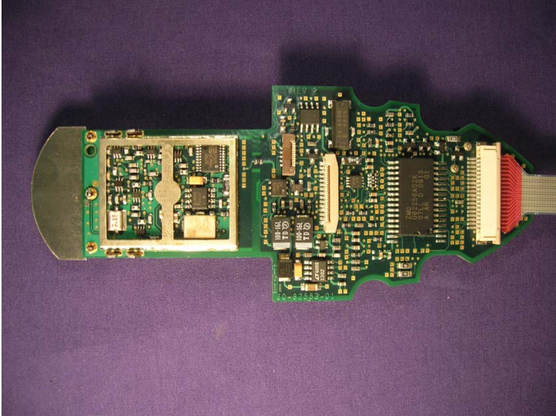
Top w/ RF Shield Removed
