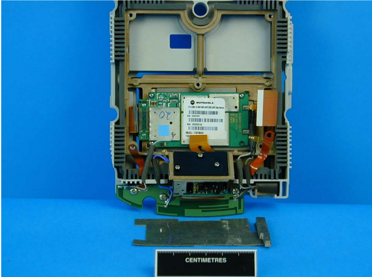
Internal View 11
