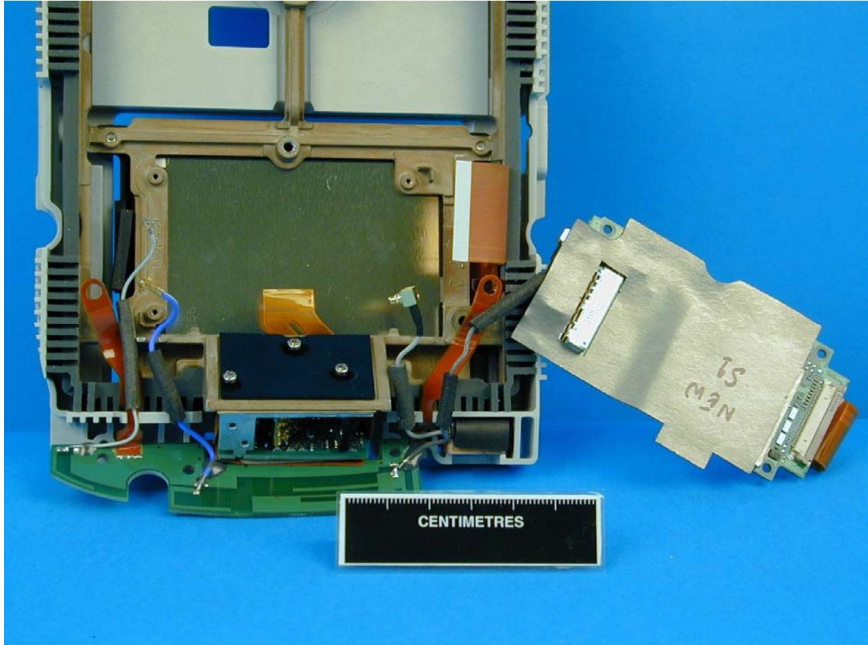
Internal View 12
