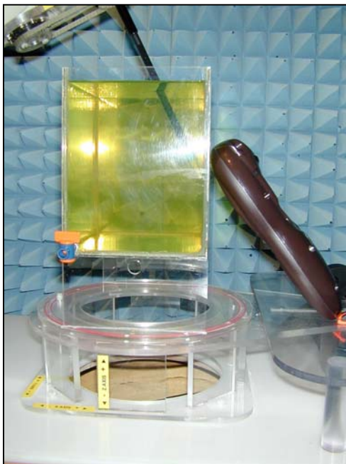
Figure 35. Positional photograph 4111-CDMA Touch Front Top Facing
