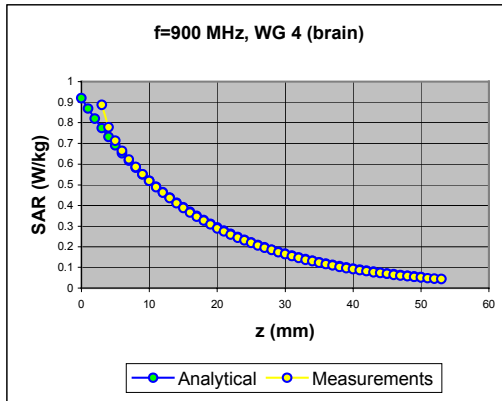
Figure 7. The measured SAR decay function along the centreline of the WG4 waveguide with conversion factors adjusted to fit to the theoretical function for the particular dimension, frequency, power and liquid properties employed.
