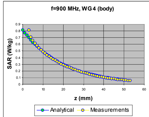
Figure 7. The measured SAR decay function along the centreline of the WG4 waveguide with conversion factors adjusted to fit to the theoretical function for the particular dimension, frequency, power and liquid properties employed.
