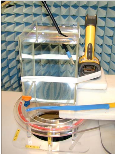
Figure 24. Positional photograph of the LS3478 LHS facing to Phantom side
