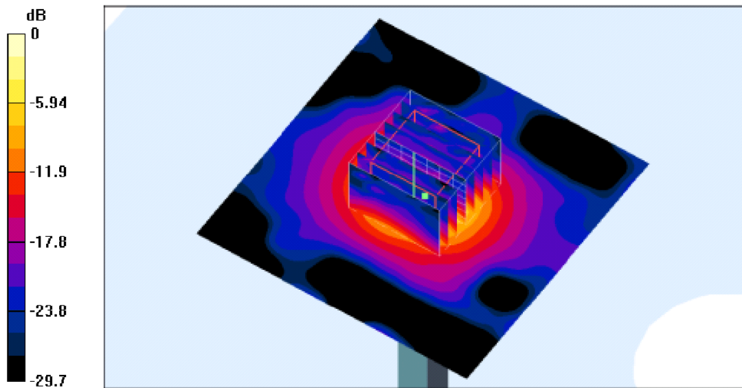
0 dB = 15.2mW/g
