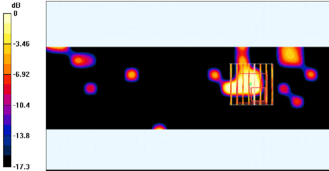
0 dB = 0.175mW/g
