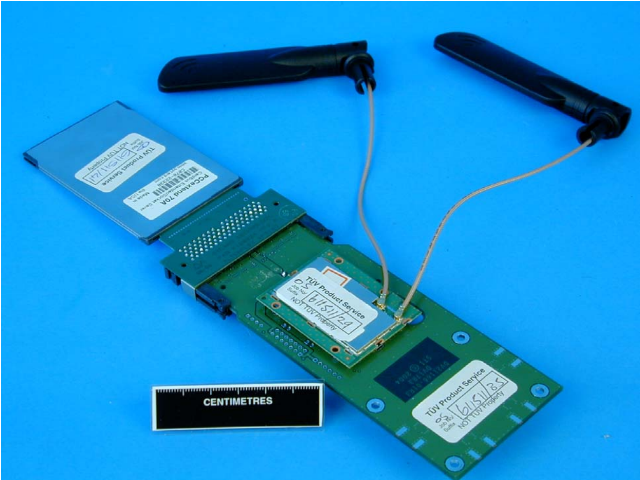
System Set Up Showing Antennas
