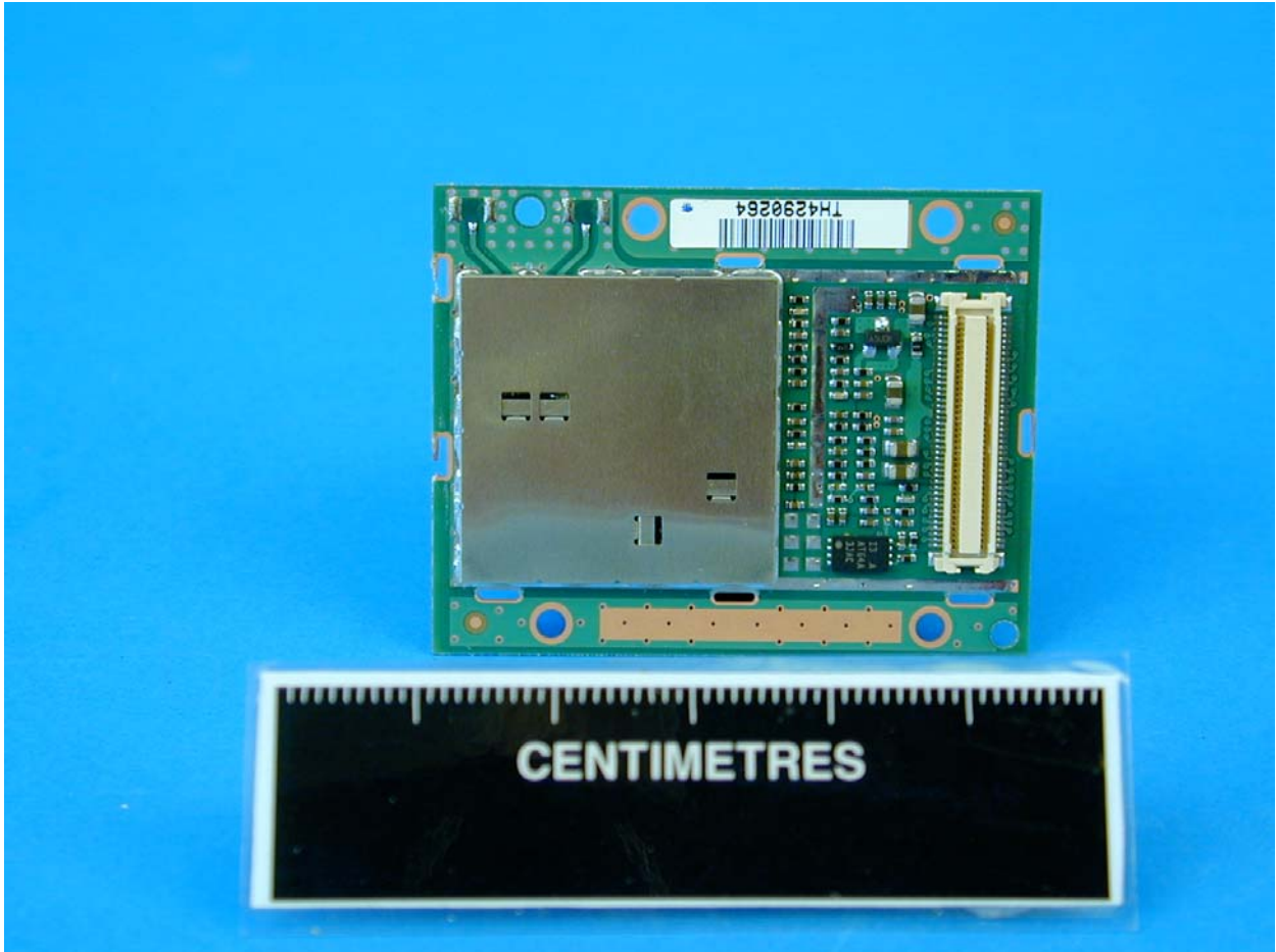
Front View 21-21160-01
