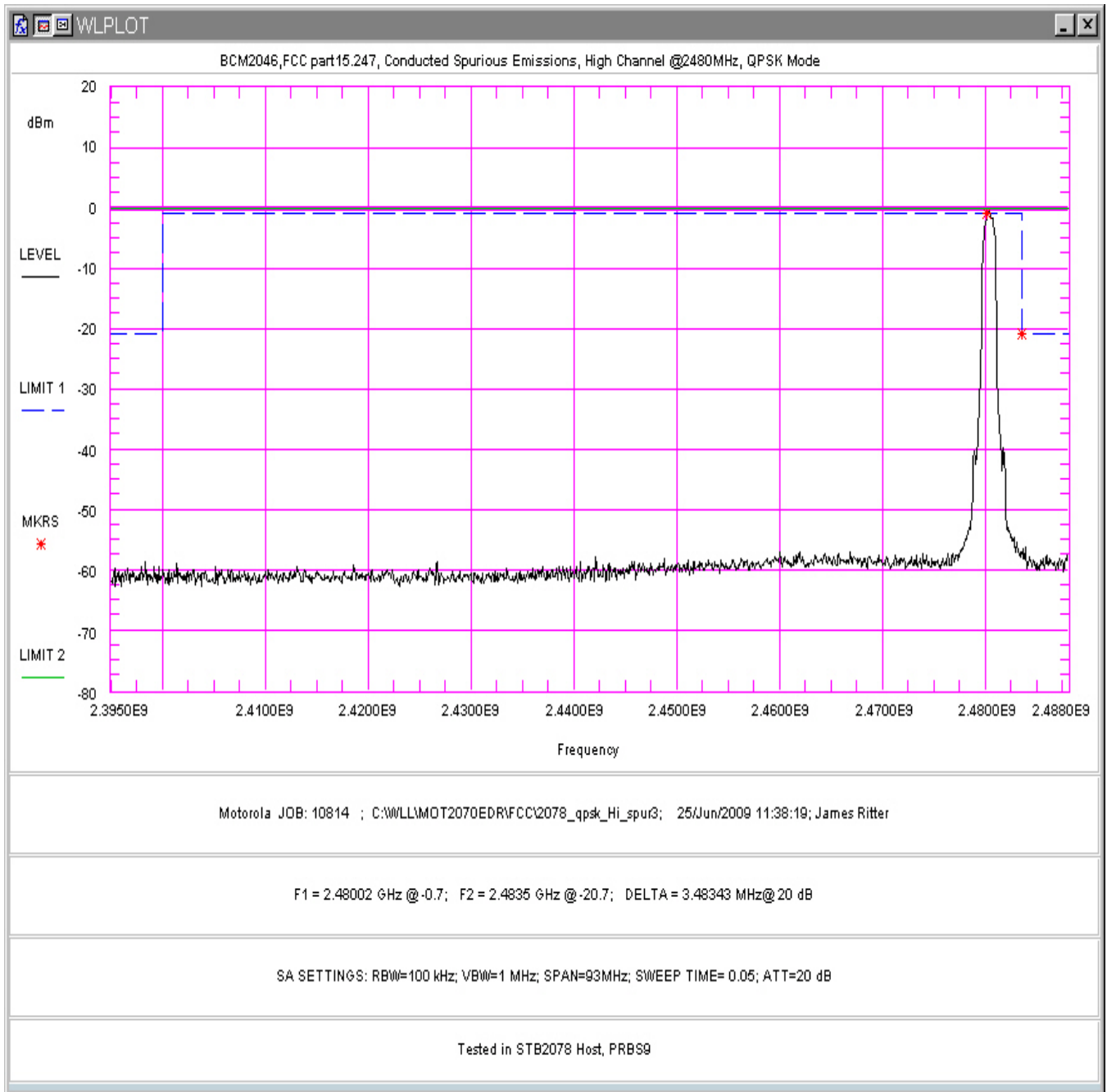
Figure 113. Conducted Spurious Emissions, QPSK Mode, High Channel 2.395- 2.488GHz (in STB2078 Host)
