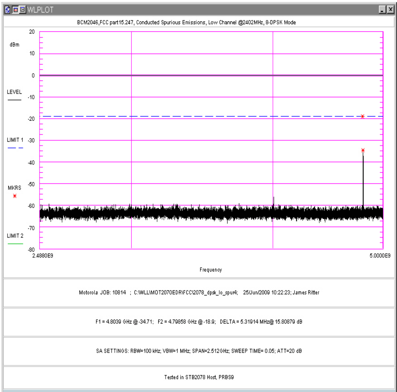
Figure 126. Conducted Spurious Emissions, 8-DPSK Mode, Low Channel 2.488 – 5 GHz (in STB2078 Host)
