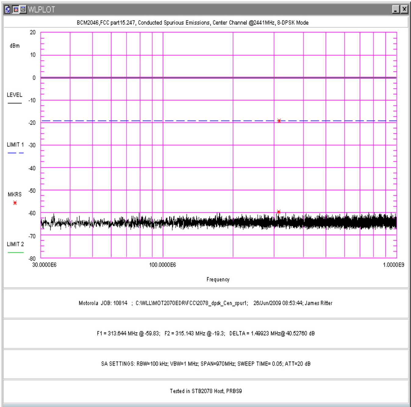
Figure 131 Conducted Spurious Emissions, 8-DPSK Mode, Center Channel 30 - 1000MHz (in STB2078 Host)
