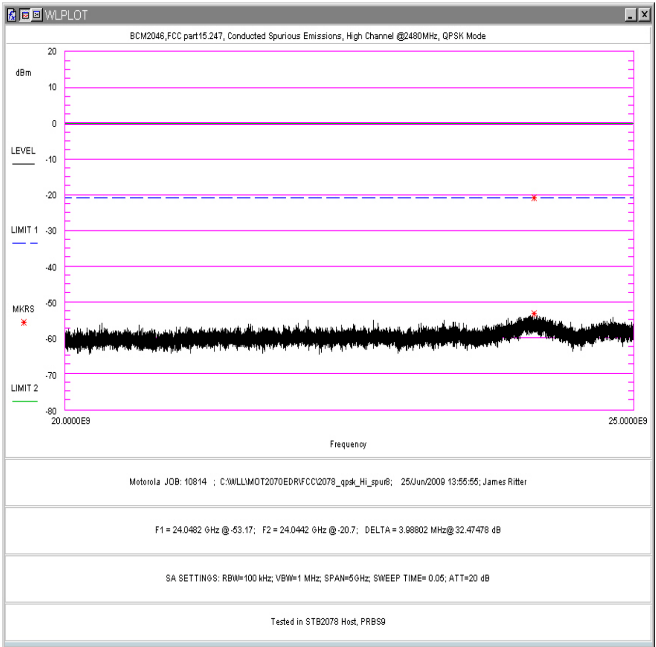
Figure 118. Conducted Spurious Emissions, QPSK Mode, High Channel 20-25GHz (in STB2078 Host)
