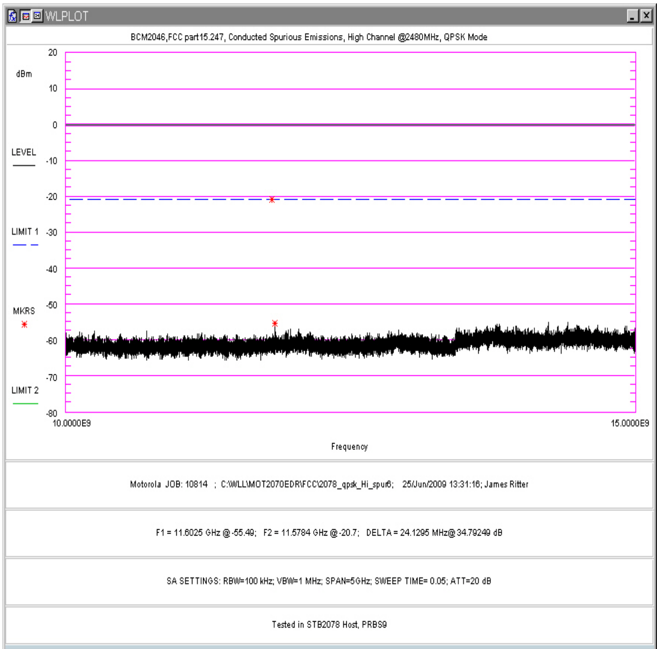
Figure 116. Conducted Spurious Emissions, QPSK Mode, High Channel 10- 15GHz (in STB2078 Host)
