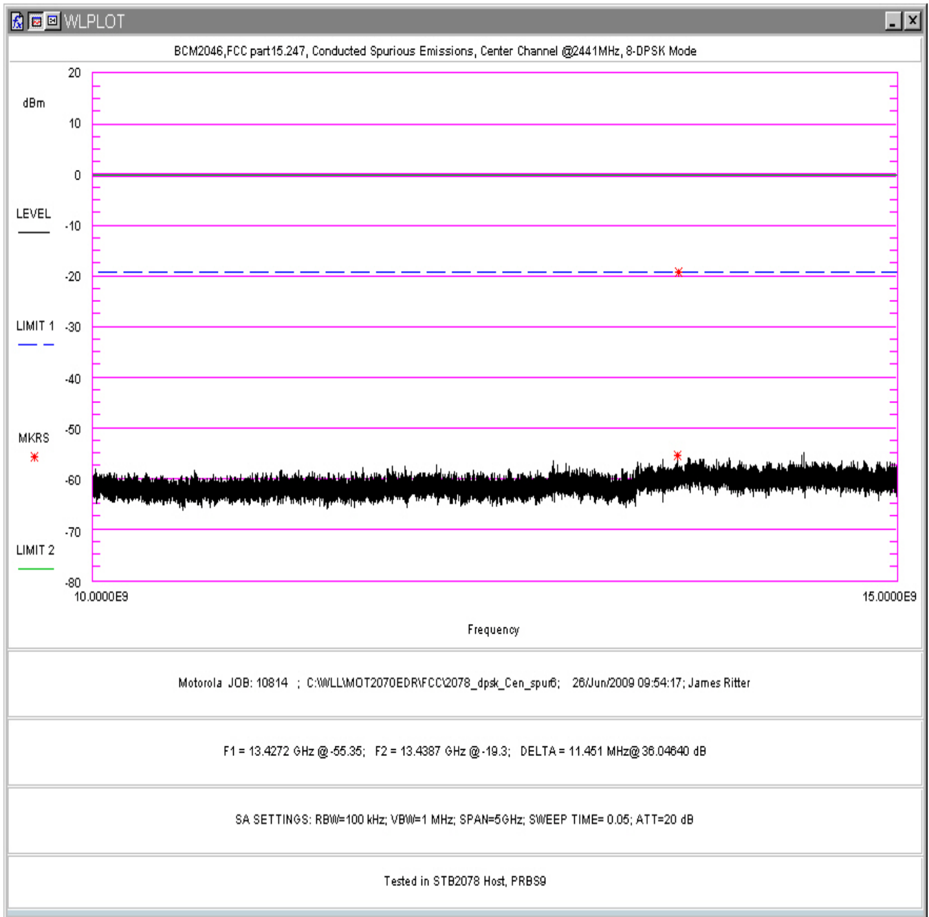
Figure 136. Conducted Spurious Emissions, 8-DPSK Mode, Center Channel 10- 15GHz (in STB2078 Host)
