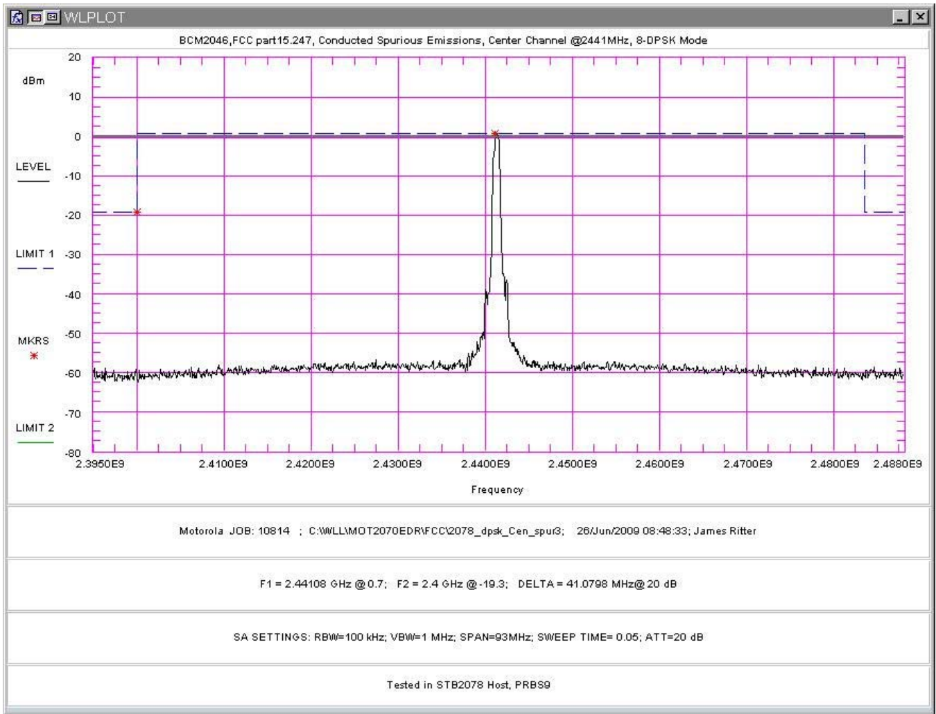
Figure 133. Conducted Spurious Emissions, 8-DPSK Mode, Center Channel 2.395- 2.488GHz (in STB2078 Host)
