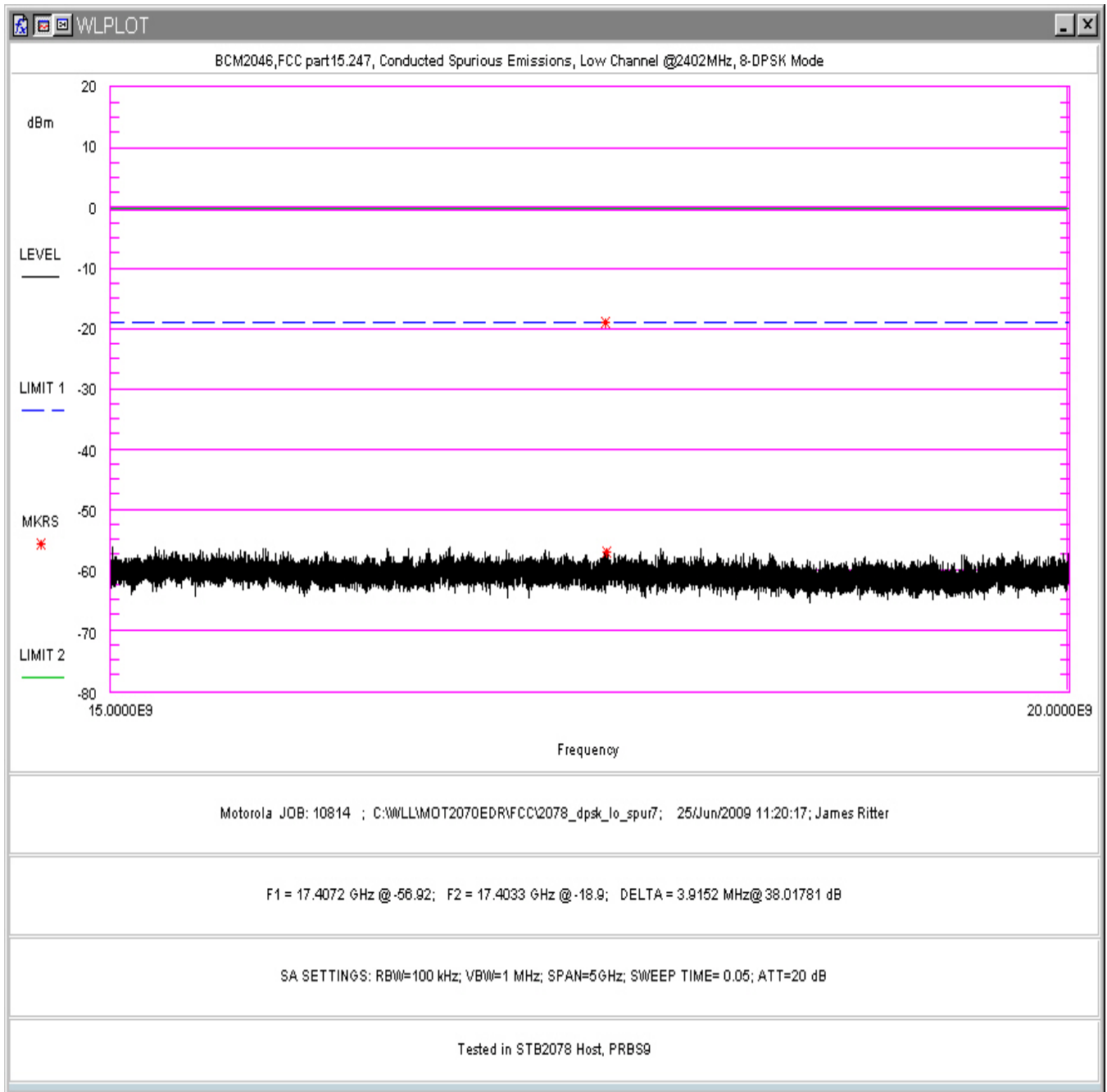
Figure 129. Conducted Spurious Emissions, 8-DPSK Mode, Low Channel 15- 20GHz (in STB2078 Host)
