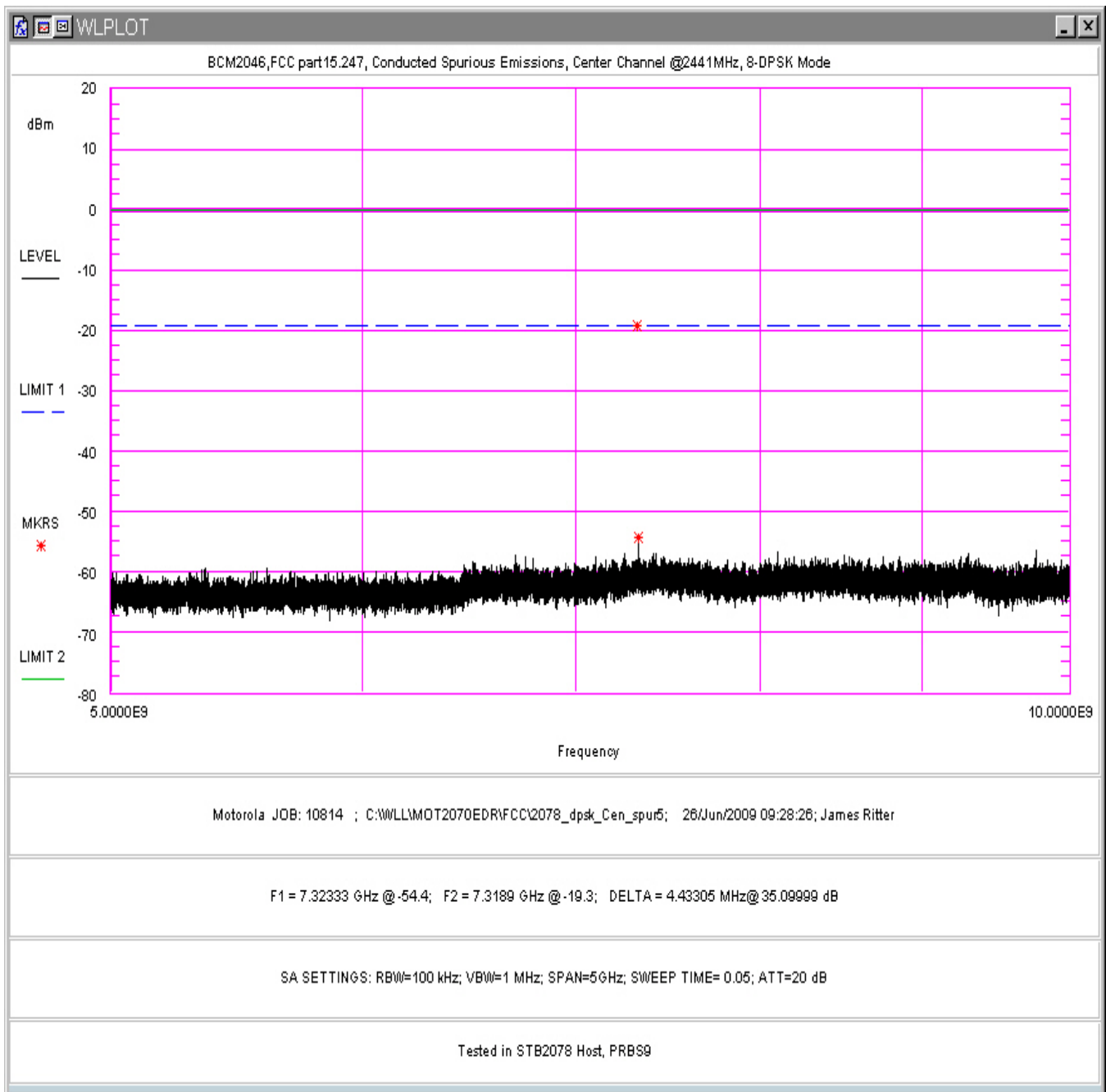
Figure 135. Conducted Spurious Emissions, 8-DPSK Mode, Center Channel 5-10GHz (in STB2078 Host)
