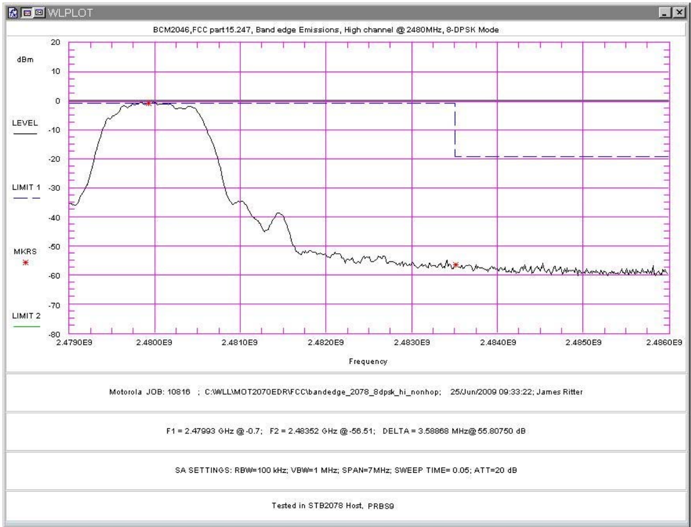
Figure 121. Upper Band Edge Plot, 8-DPSK Mode, High Channel (in STB2078 Host)
