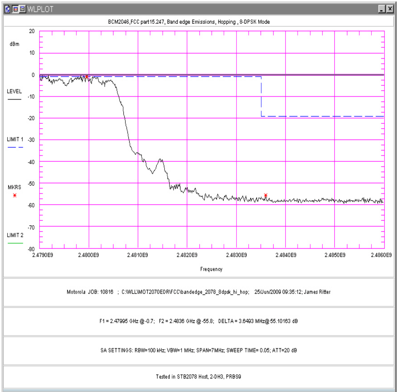
Figure 122. Upper Band Edge Plot, 8-DPSK Mode, Hopping Mode (in STB2078 Host)
