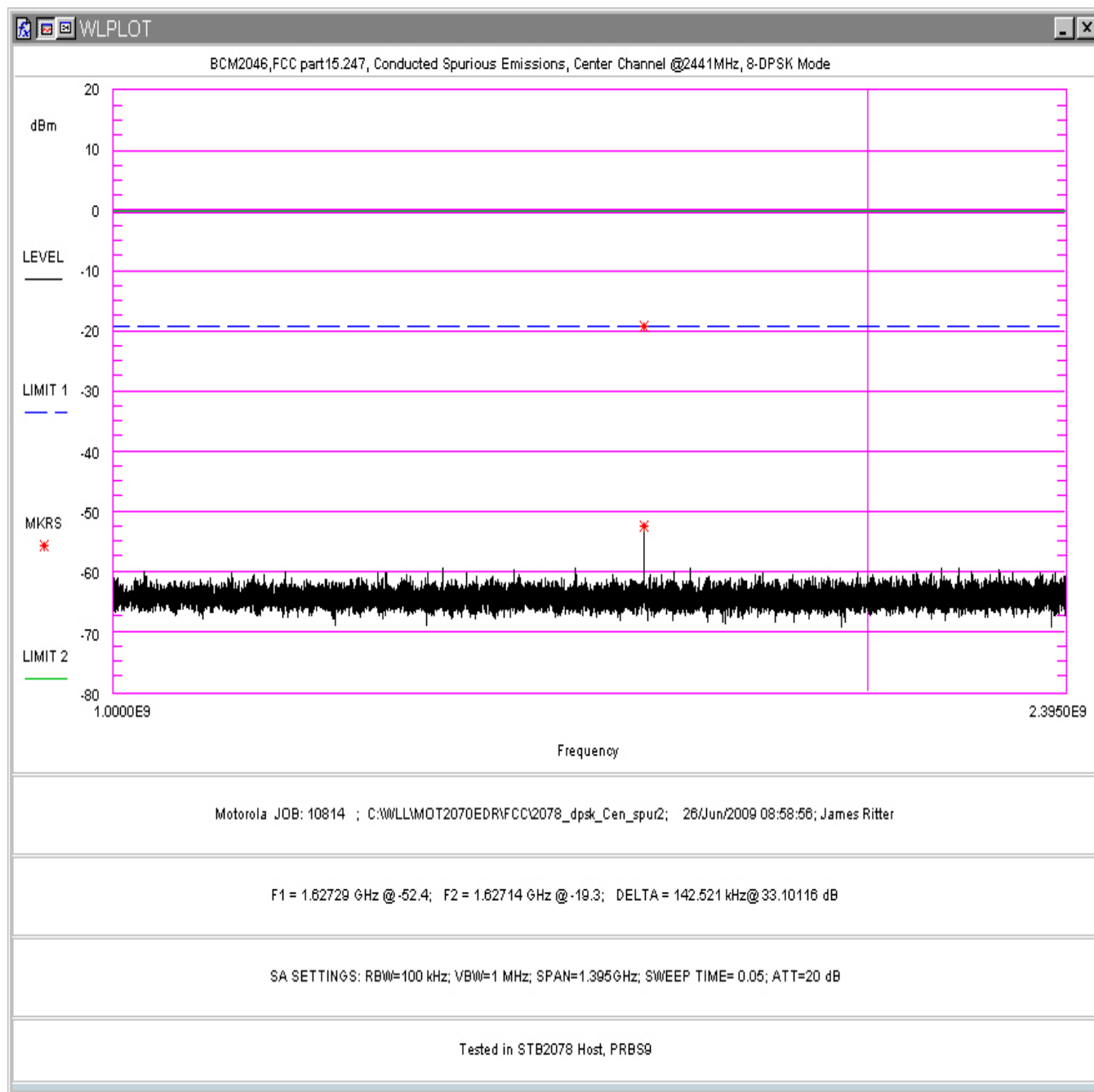
Figure 132. Conducted Spurious Emissions, 8-DPSK Mode, Center Channel 1 – 2.395GHz (in STB2078 Host)
