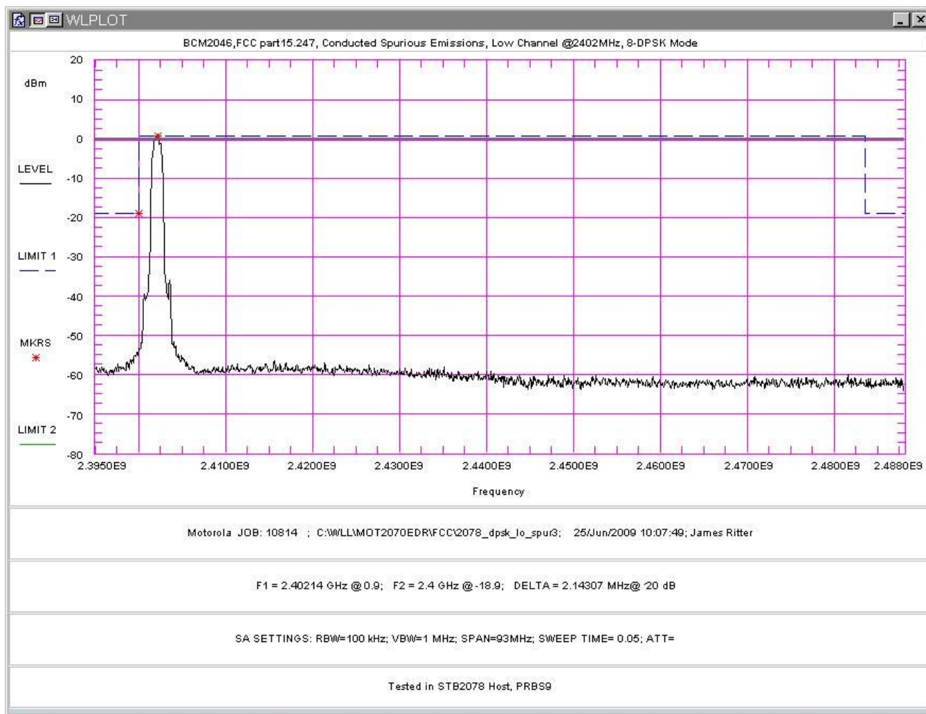
Figure 125. Conducted Spurious Emissions, 8-DPSK Mode, Low Channel 2.395- 2.488GHz (in STB2078 Host)
