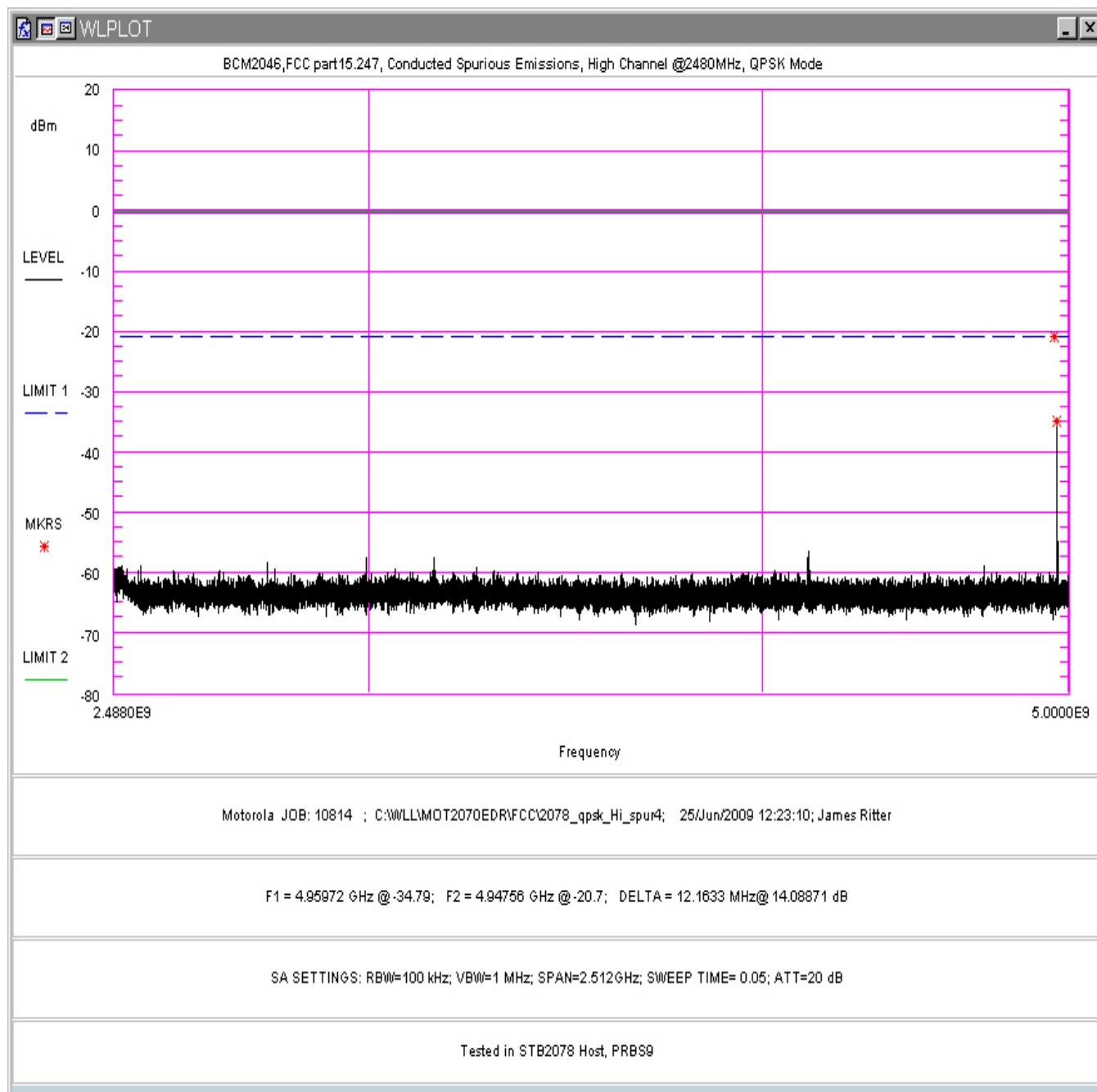
Figure 114. Conducted Spurious Emissions, QPSK Mode, High Channel 2.488 – 5 GHz (in STB2078 Host)
