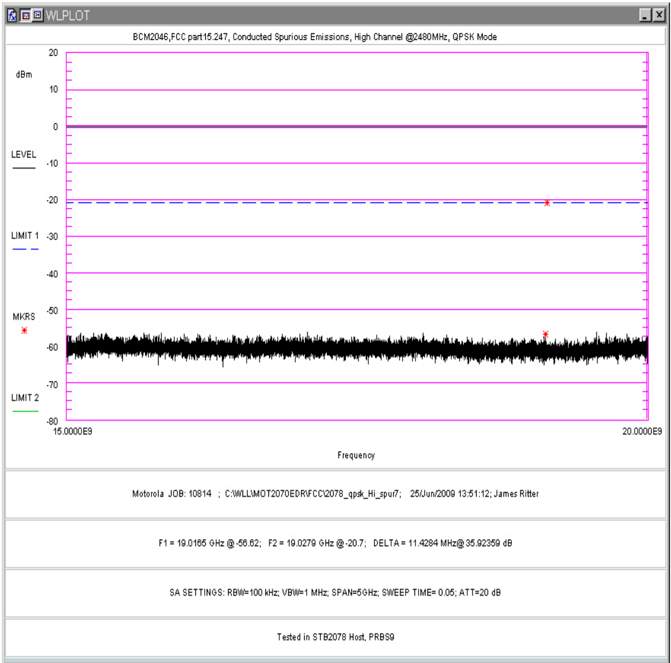
Figure 117. Conducted Spurious Emissions, QPSK Mode, High Channel 15- 20GHz (in STB2078 Host)
