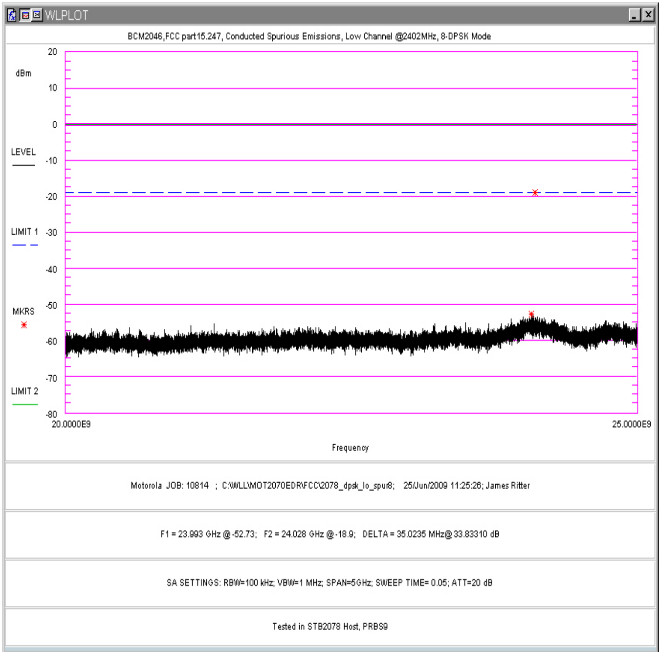
Figure 130. Conducted Spurious Emissions, 8-DPSK Mode, Low Channel 20-25GHz (in STB2078 Host)
