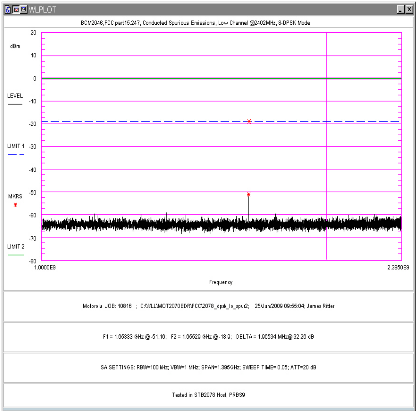
Figure 124. Conducted Spurious Emissions, 8-DPSK Mode, Low Channel 1 – 2.395GHz (in STB2078 Host)
