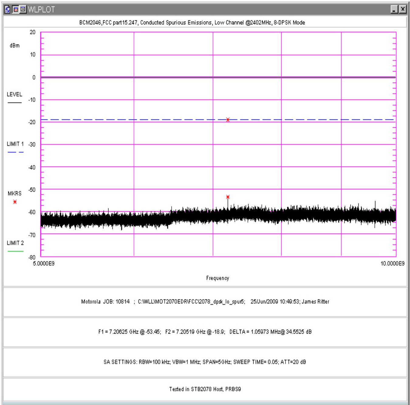
Figure 127. Conducted Spurious Emissions, 8-DPSK Mode, Low Channel 5-10GHz (in STB2078 Host)
