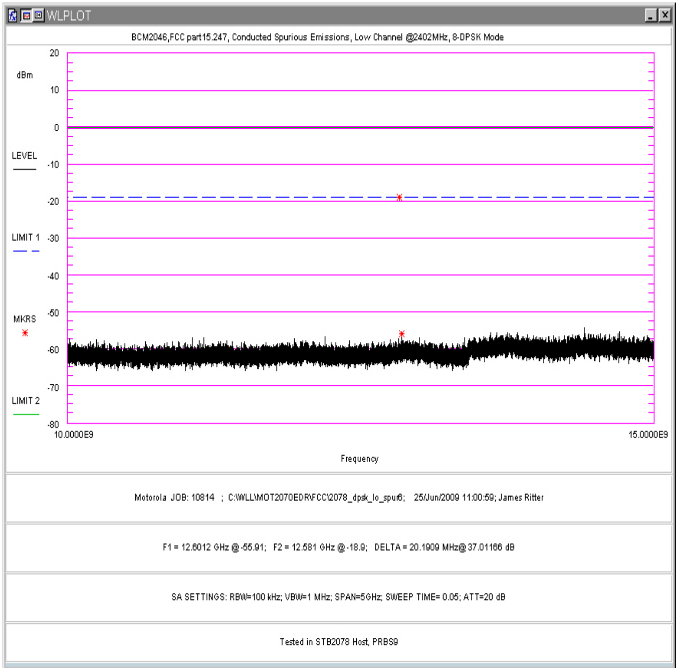
Figure 128. Conducted Spurious Emissions, 8-DPSK Mode, Low Channel 10- 15GHz (in STB2078 Host)
