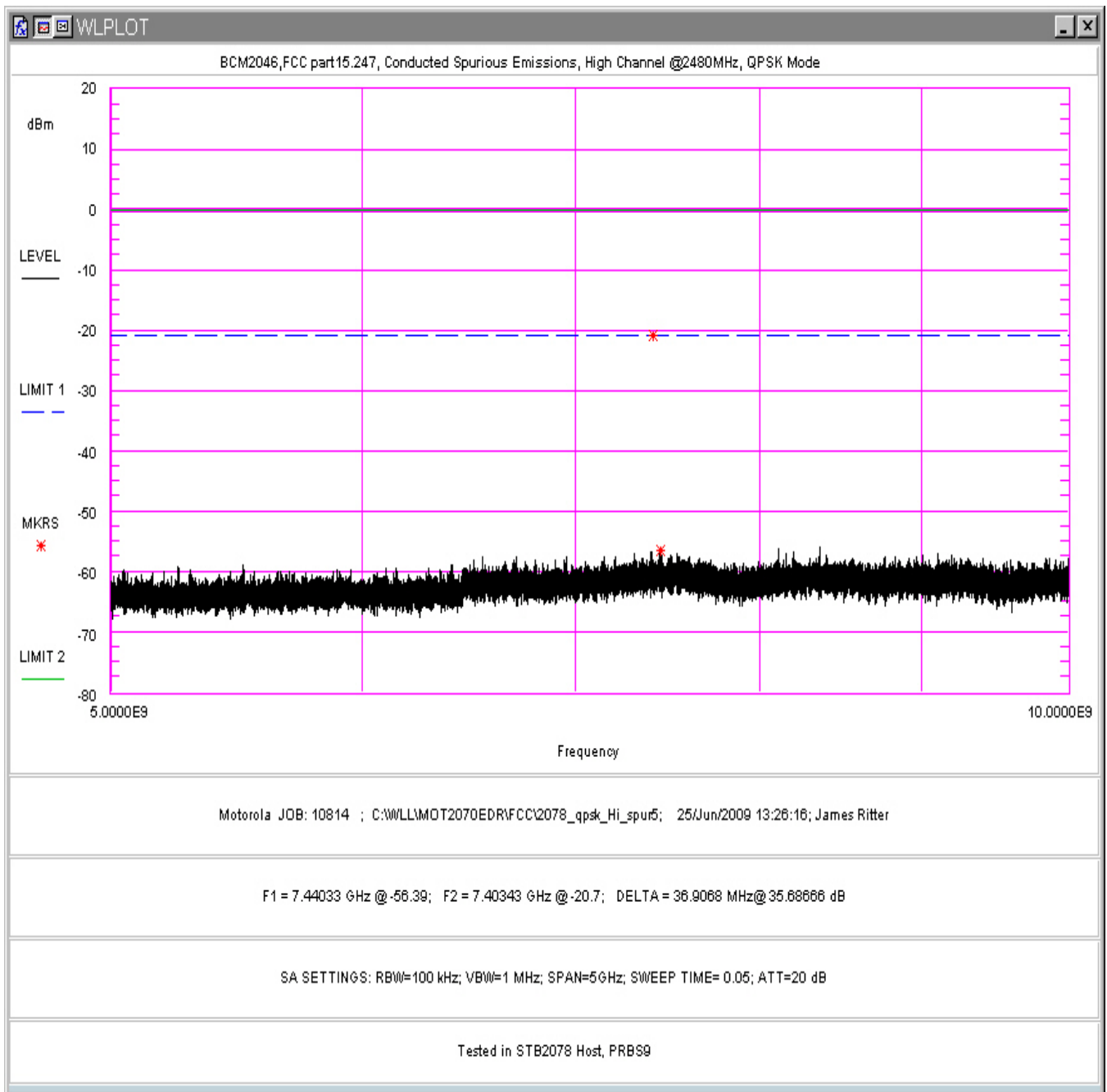
Figure 115. Conducted Spurious Emissions, QPSK Mode, High Channel 5-10GHz (in STB2078 Host)
