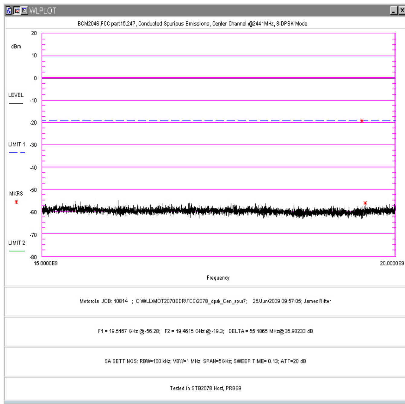
Figure 137. Conducted Spurious Emissions, 8-DPSK Mode, Center Channel 15- 20GHz (in STB2078 Host)
