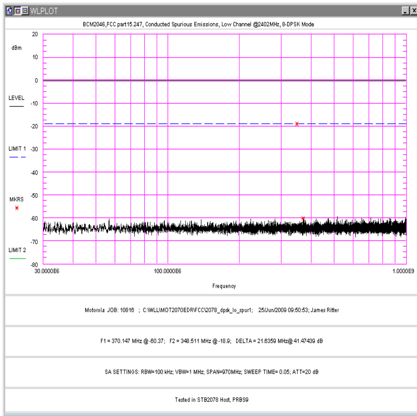
Figure 123. Conducted Spurious Emissions, 8-DPSK Mode, Low Channel 30 - 1000MHz (in STB2078 Host)
