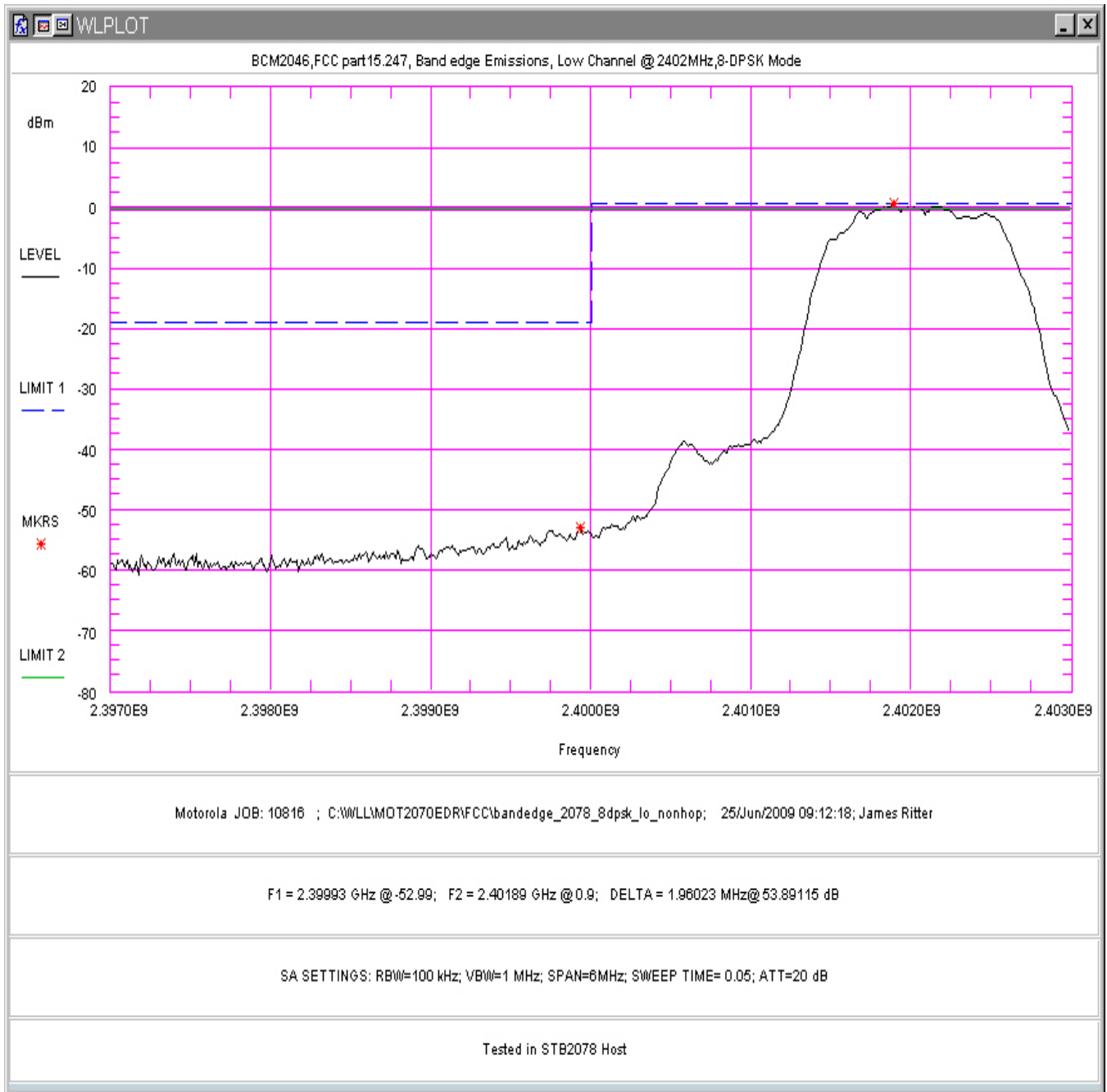
Figure 119. Lower Band Edge Plot, 8-DPSK Mode, Low Channel (in STB2078 Host)
