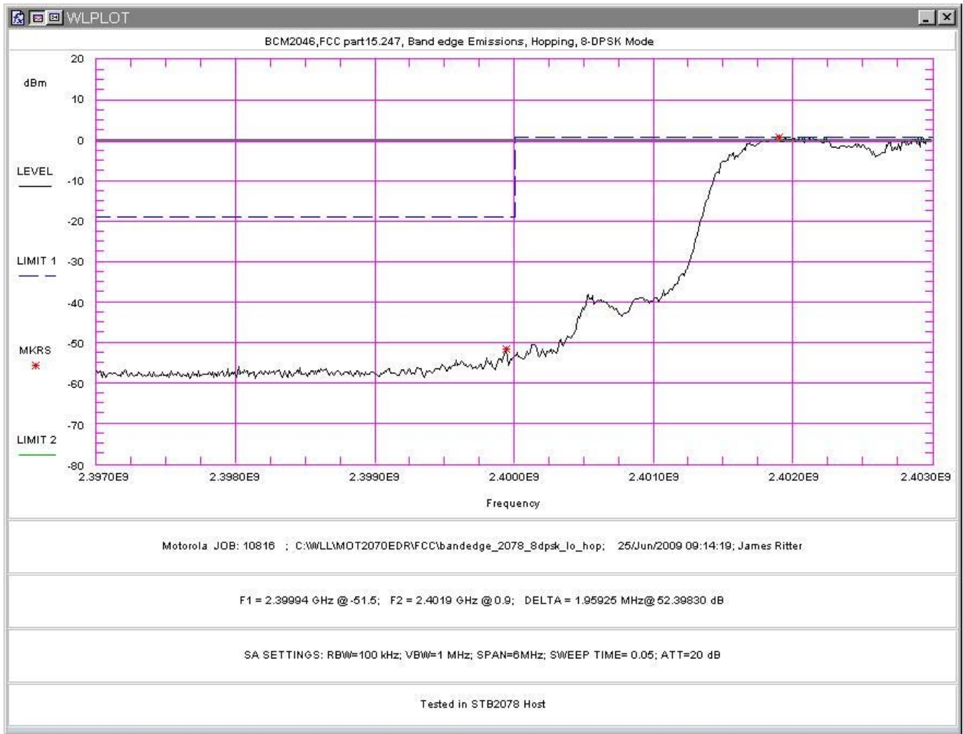
Figure 120. Lower Band Edge Plot, 8-DPSK Mode, Hopping Mode (in STB2078 Host)
