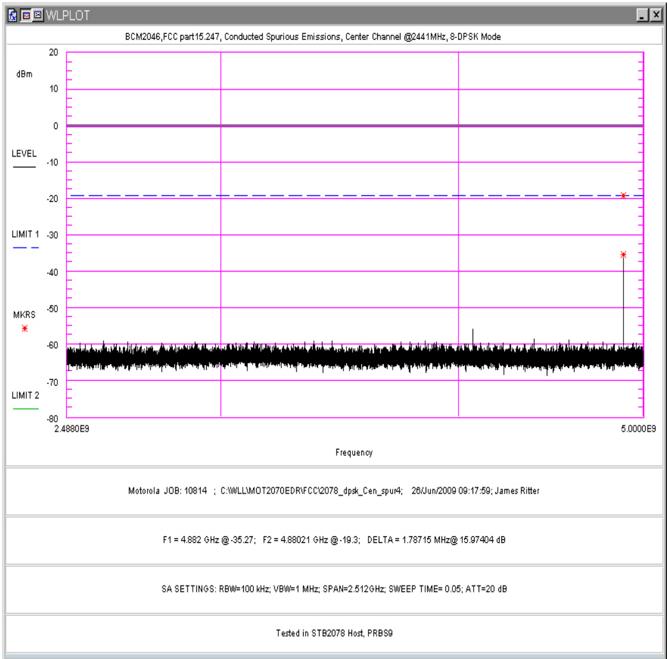
Figure 134. Conducted Spurious Emissions, 8-DPSK Mode, Center Channel 2.488 – 5 GHz (in STB2078 Host)
