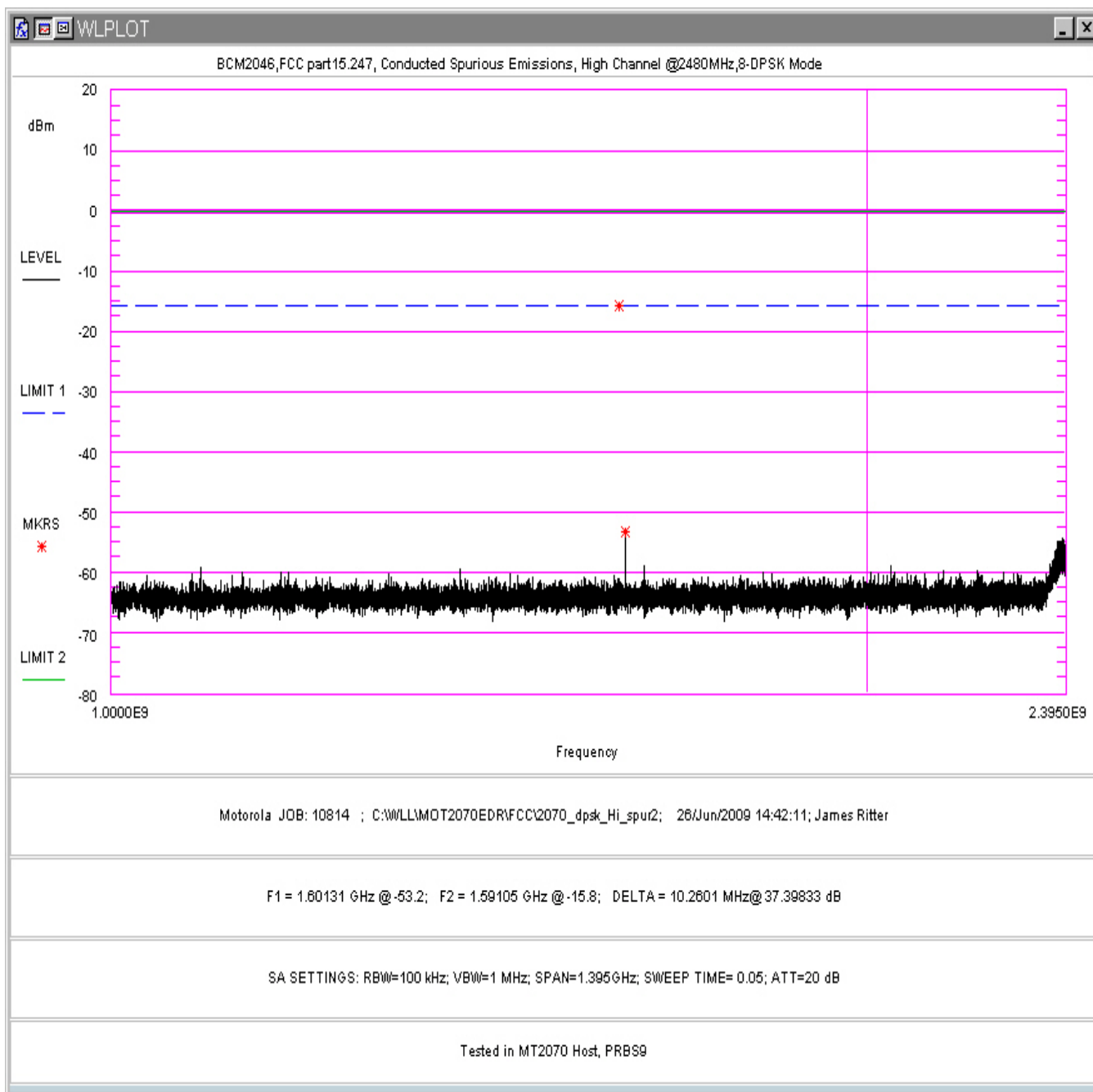
Figure 84. Conducted Spurious Emissions, 8-DPSK Mode, High Channel 1 – 2.395GHz (in MT2070 Host)
