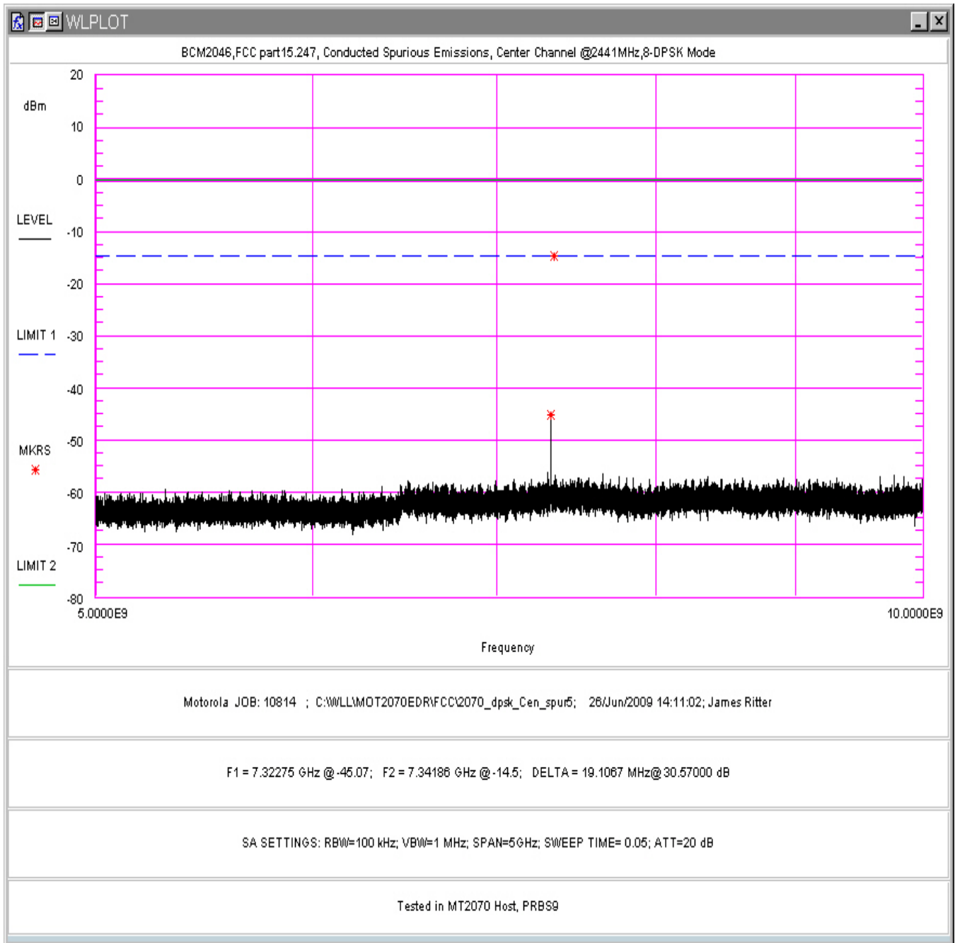
Figure 79. Conducted Spurious Emissions, 8-DPSK Mode, Center Channel 5 - 10GHz (in MT2070 Host)
