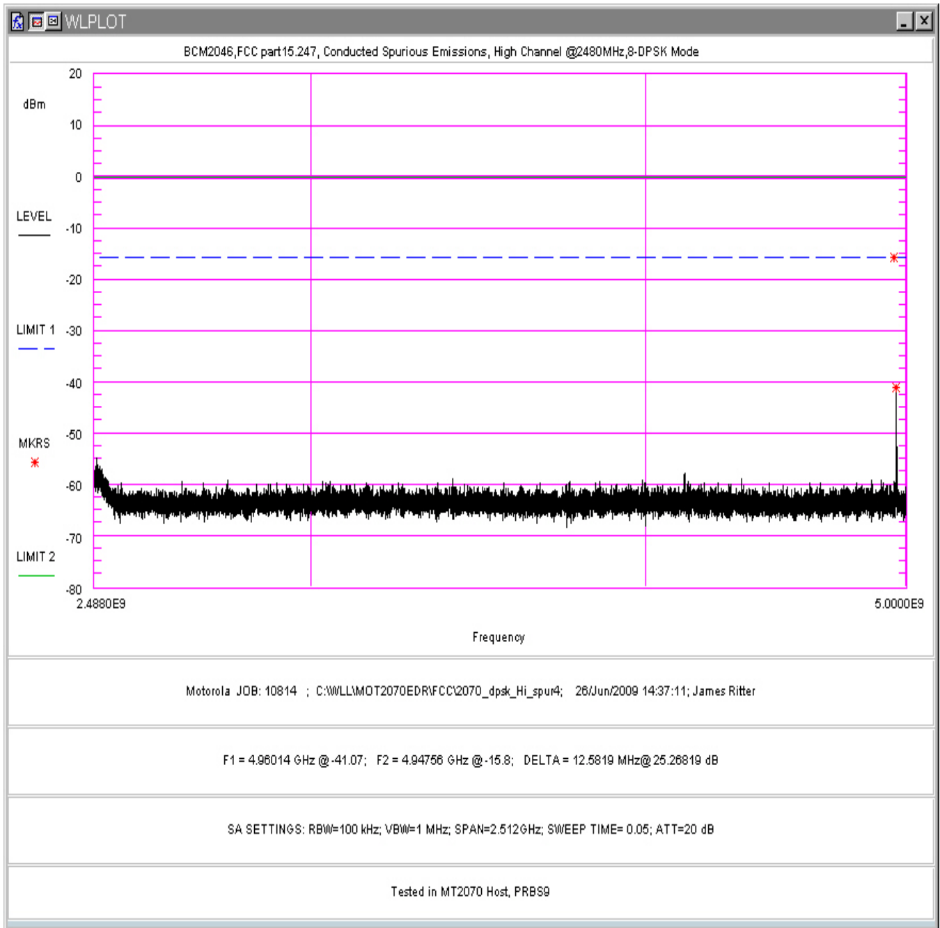
Figure 86. Conducted Spurious Emissions, 8-DPSK Mode, High Channel 2.488 - 5GHz (in MT2070 Host)
