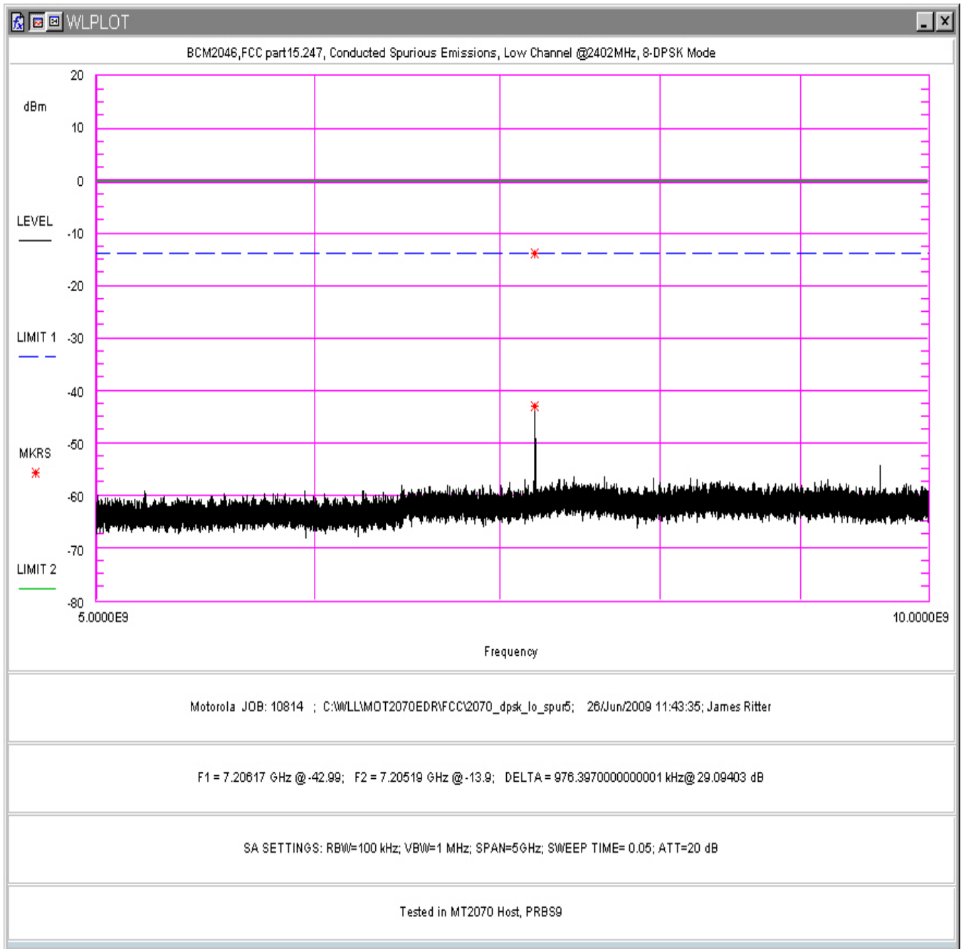
Figure 71. Conducted Spurious Emissions, 8-DPSK Mode, Low Channel 5-10GHz (in MT2070 Host)
