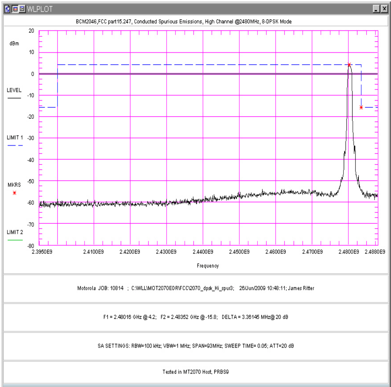
Figure 85. Conducted Spurious Emissions, 8-DPSK Mode, High Channel 2.395 – 2.488GHz (in MT2070 Host)
