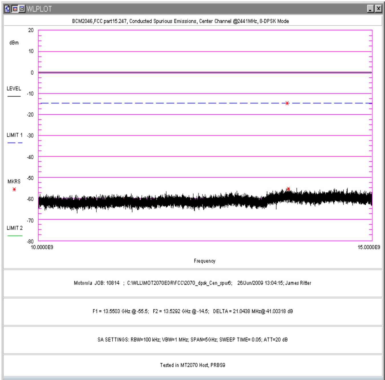
Figure 80. Conducted Spurious Emissions, 8-DPSK Mode, Center Channel 10-15GHz (in MT2070 Host)
