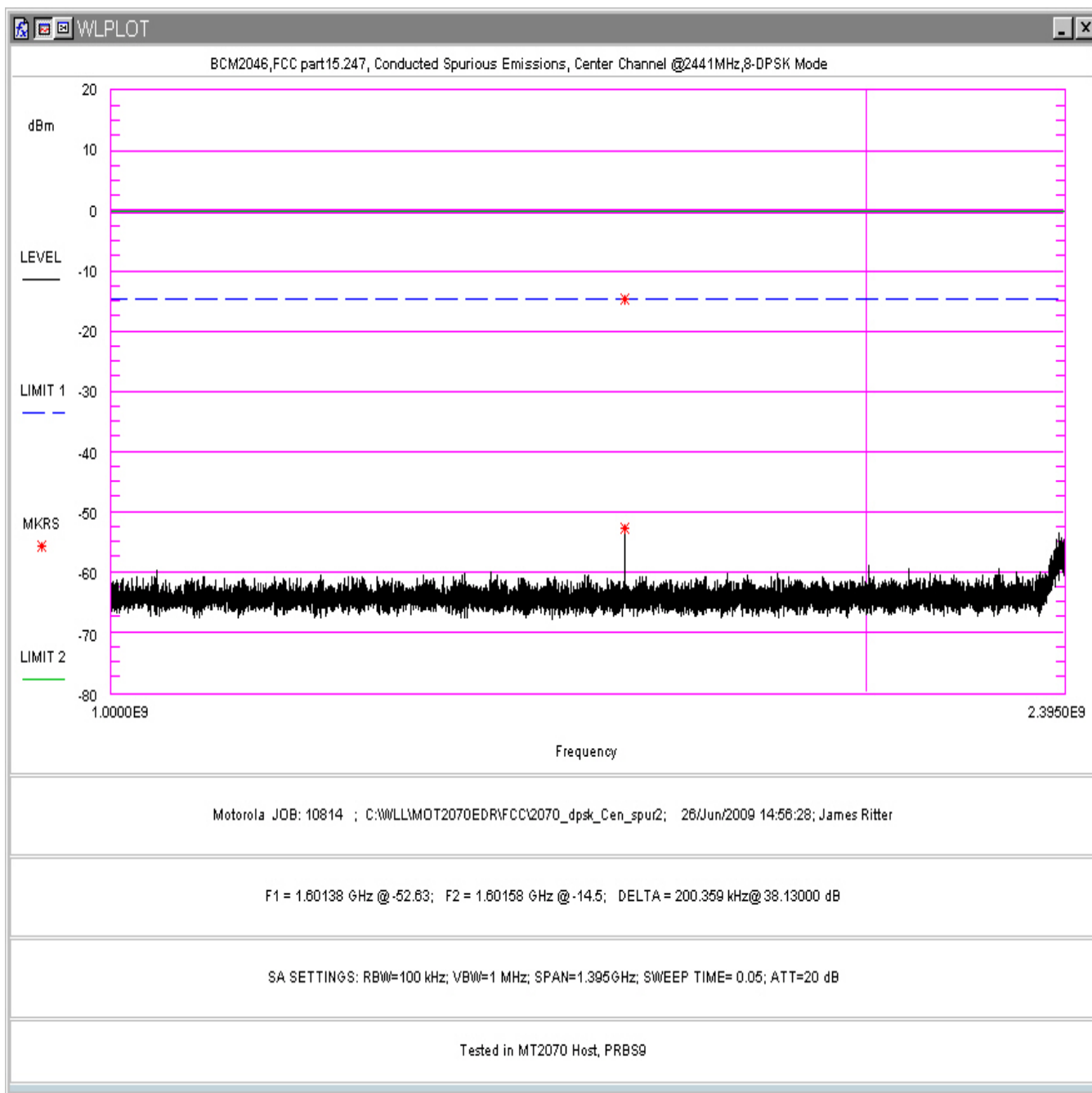
Figure 76. Conducted Spurious Emissions, 8-DPSK Mode, Center Channel 1 – 2.395GHz (in MT2070 Host)
