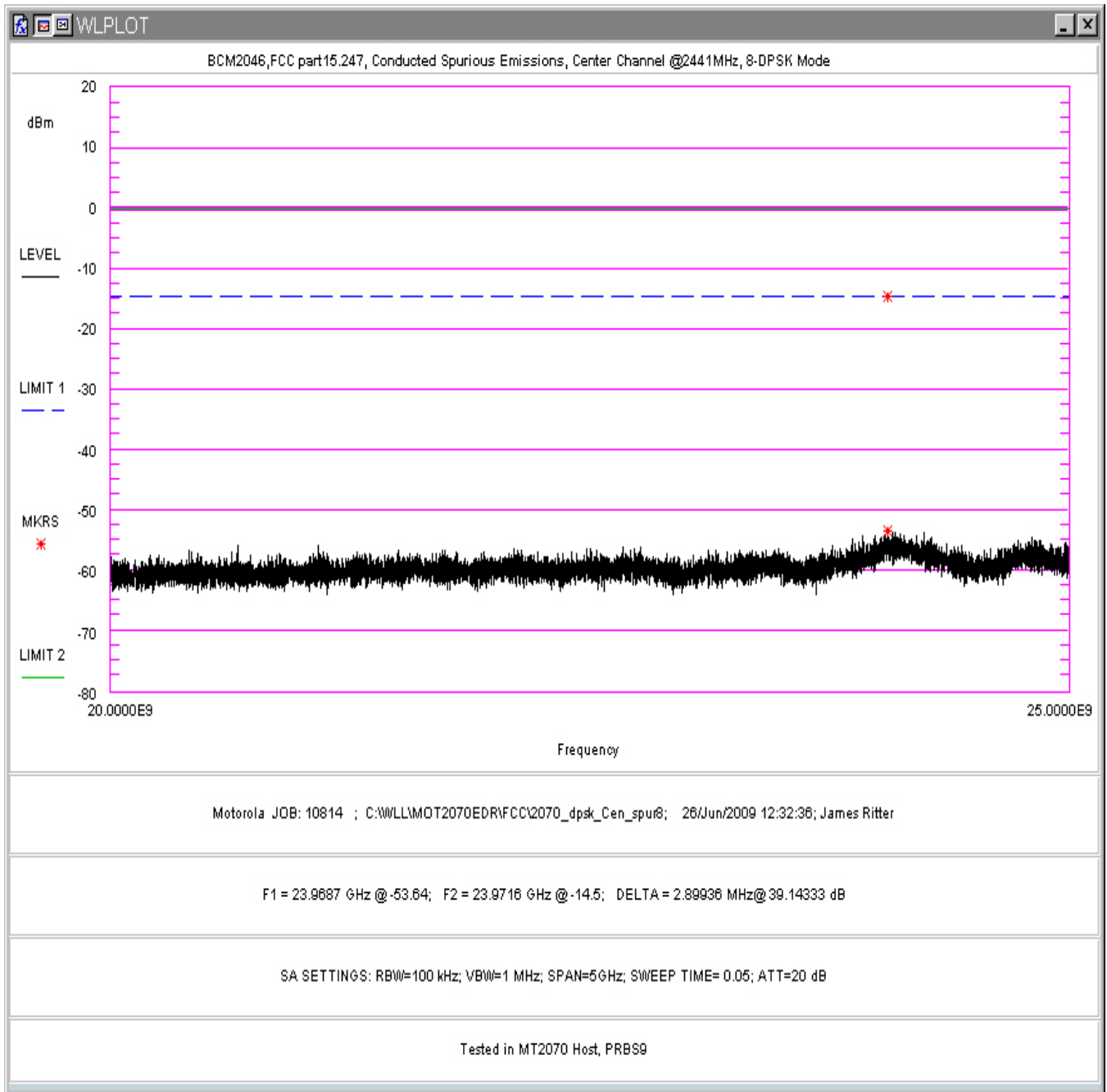
Figure 82. Conducted Spurious Emissions, 8-DPSK Mode, Center Channel 20-25GHz (in MT2070 Host)
