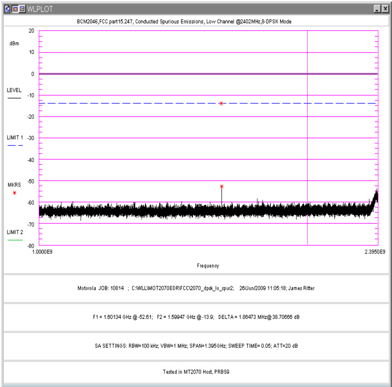
Figure 68. Conducted Spurious Emissions, 8-DPSK Mode, Low Channel 1 – 2.395GHz (in MT2070 Host)
