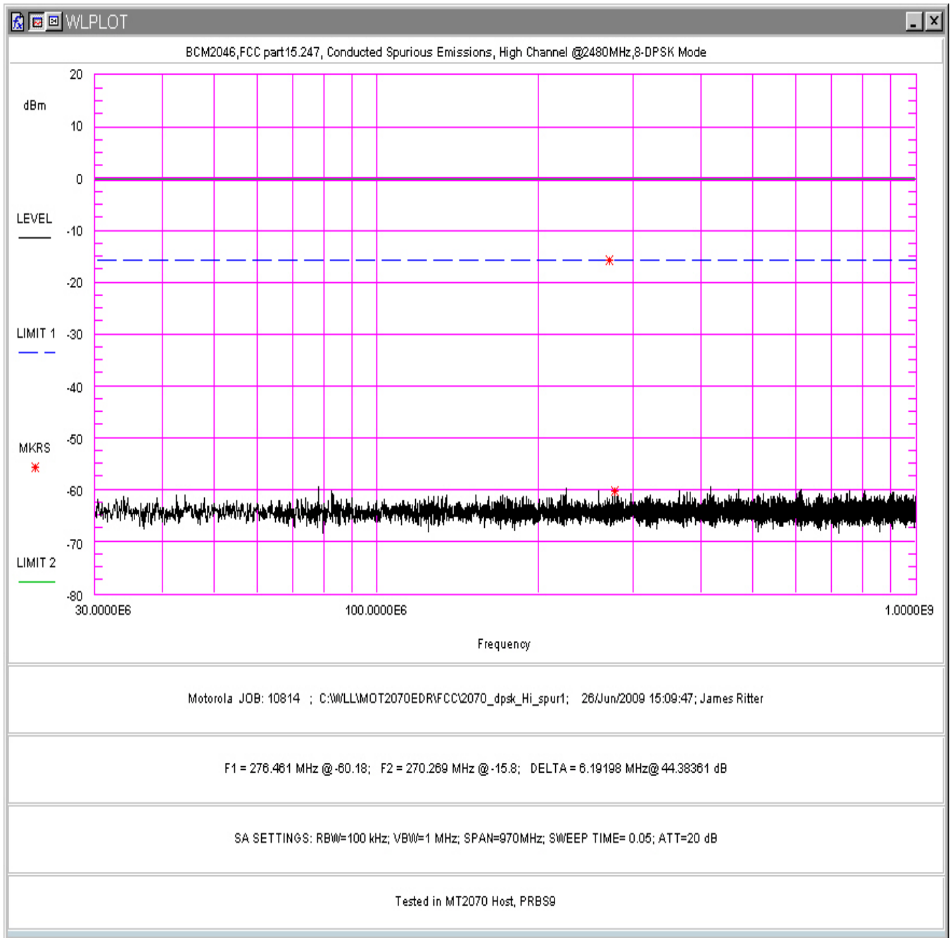
Figure 83. Conducted Spurious Emissions, 8-DPSK Mode, High Channel 30 - 1000MHz (in MT2070 Host)
