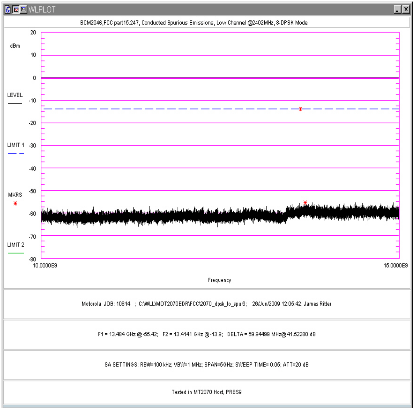
Figure 72. Conducted Spurious Emissions, 8-DPSK Mode, Low Channel 10-15GHz (in MT2070 Host)
