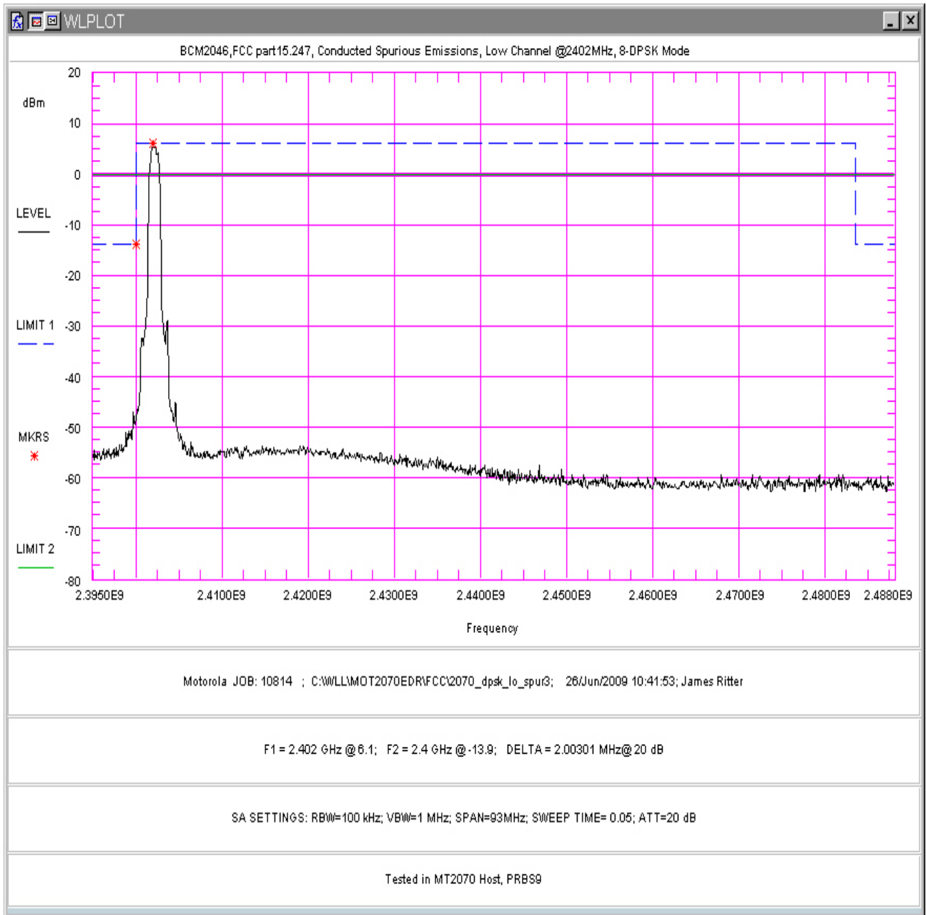
Figure 69. Conducted Spurious Emissions, 8-DPSK Mode, Low Channel 2.395 – 2.488GHz (in MT2070 Host)
