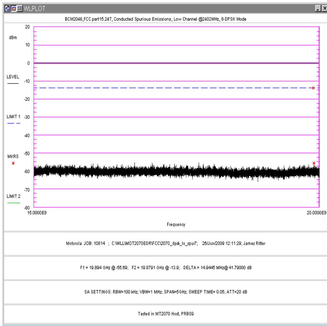
Figure 73. Conducted Spurious Emissions, 8-DPSK Mode, Low Channel 15-20GHz (in MT2070 Host)
