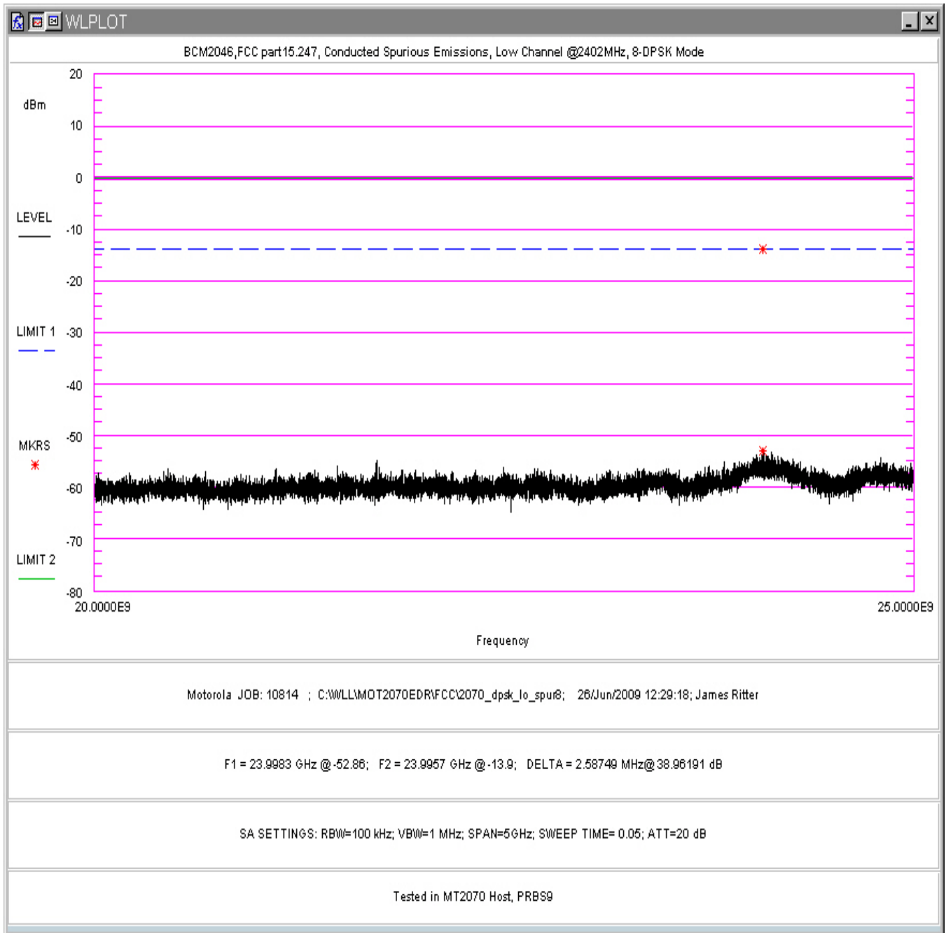
Figure 74. Conducted Spurious Emissions, 8-DPSK Mode, Low Channel 20-25GHz (in MT2070 Host)
