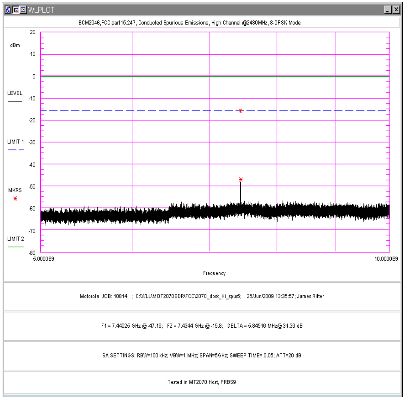
Figure 87. Conducted Spurious Emissions, 8-DPSK Mode, High Channel 5 - 10GHz (in MT2070 Host)
