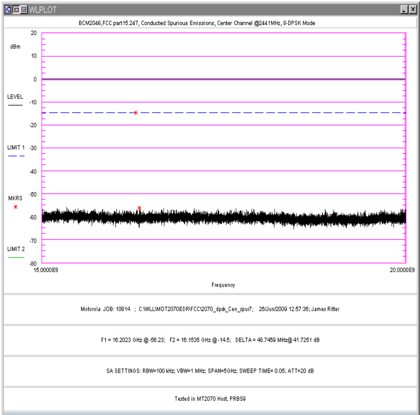
Figure 81. Conducted Spurious Emissions, 8-DPSK Mode, Center Channel 15-20GHz (in MT2070 Host)
