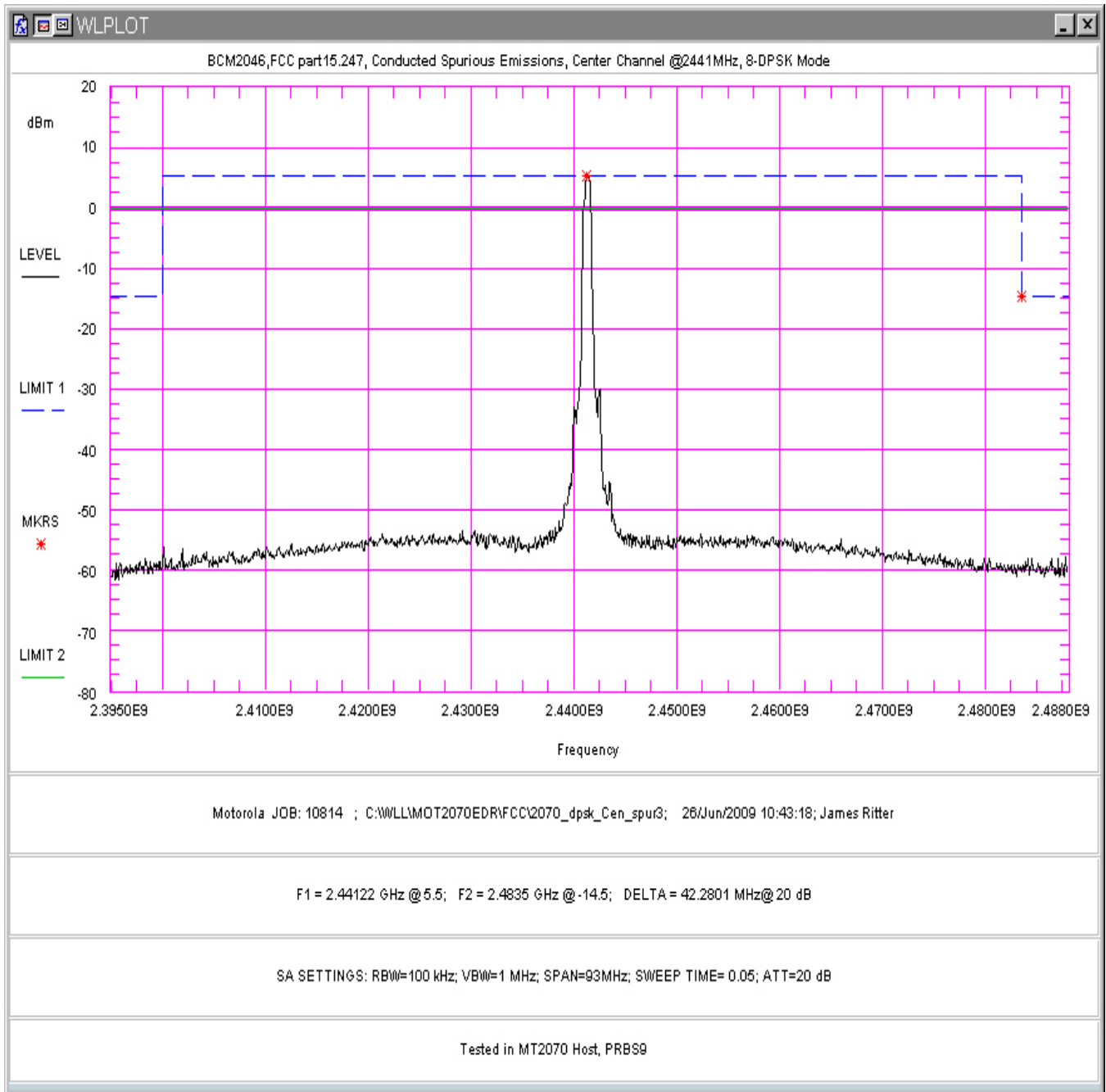
Figure 77. Conducted Spurious Emissions, 8-DPSK Mode, Center Channel 2.395 – 2.488GHz (in MT2070 Host)
