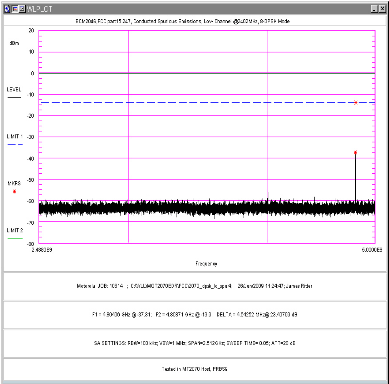
Figure 70. Conducted Spurious Emissions, 8-DPSK Mode, Low Channel 2.488 - 5GHz (in MT2070 Host)
