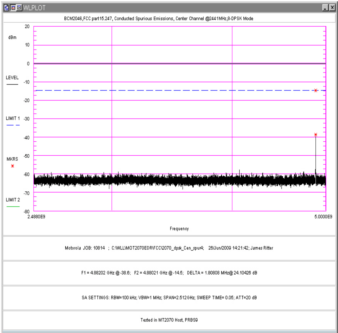
Figure 78. Conducted Spurious Emissions, 8-DPSK Mode, Center Channel 2.488 - 5GHz (in MT2070 Host)
