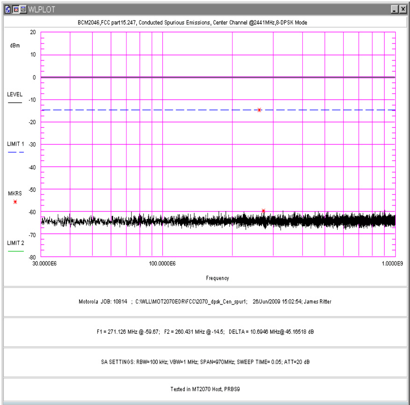
Figure 75. Conducted Spurious Emissions, 8-DPSK Mode, Center Channel 30 - 1000MHz (in MT2070 Host)
