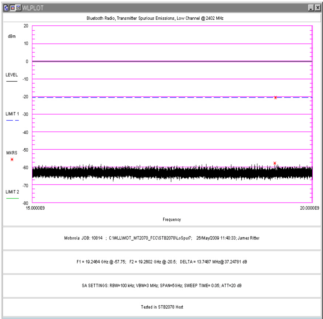
Figure 57. Conducted Spurious Emissions, Low Channel 15- 20GHz (in STB2078 Host)
