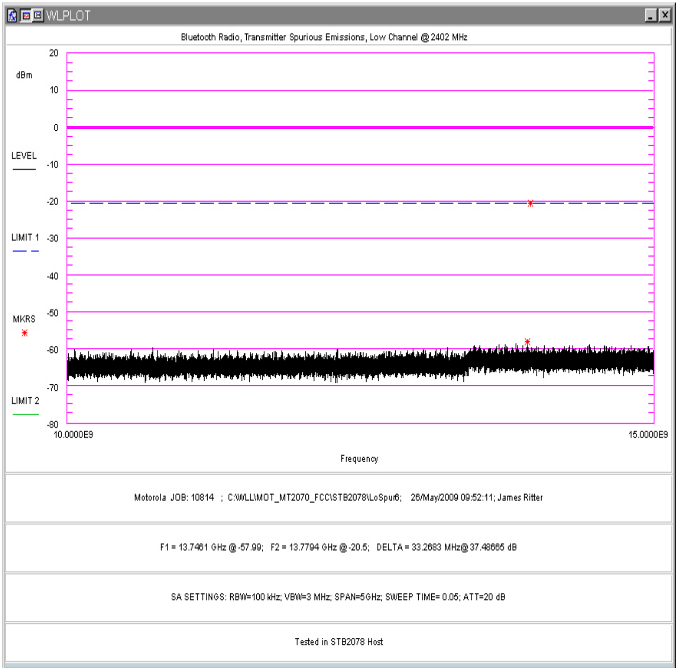
Figure 56. Conducted Spurious Emissions, Low Channel 10- 15GHz (in STB2078 Host)
