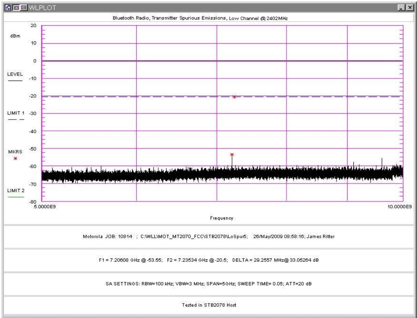
Figure 55. Conducted Spurious Emissions, Low Channel 5-10GHz (in STB2078 Host)
