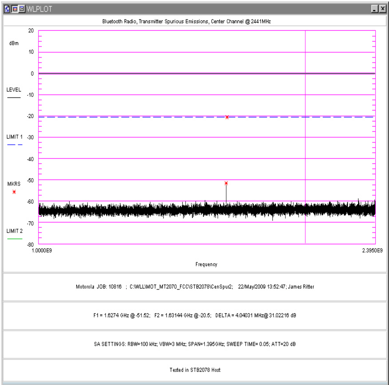
Figure 60. Conducted Spurious Emissions, Mid Channel 1 – 2.395GHz (in STB2078 Host)
