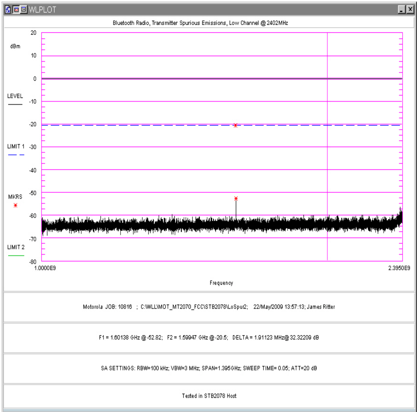
Figure 52. Conducted Spurious Emissions, Low Channel 1 – 2.395GHz (in STB2078 Host)
