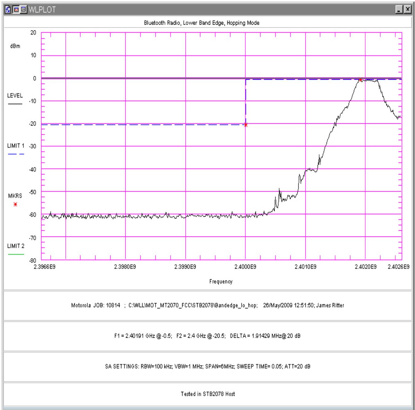
Figure 48. Lower Band Edge Plot, Hopping Mode (in STB2078 Host)
