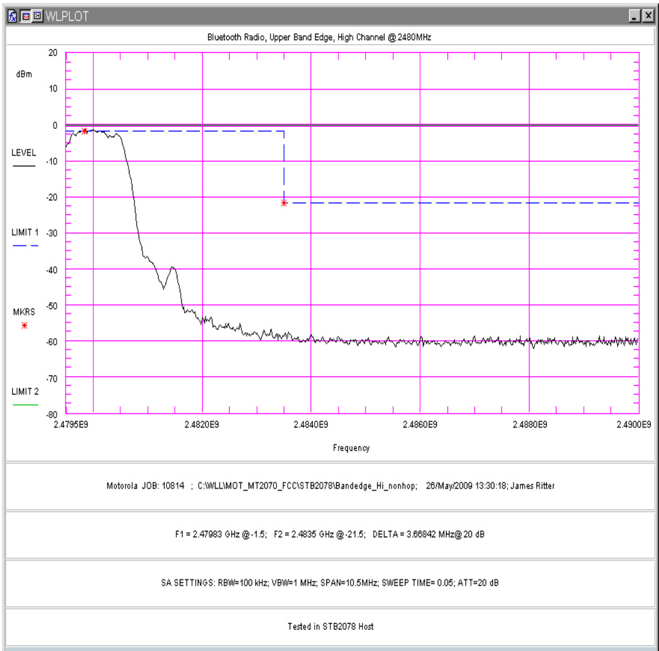
Figure 49. Upper Band Edge Plot, High Channel (in STB2078 Host)
