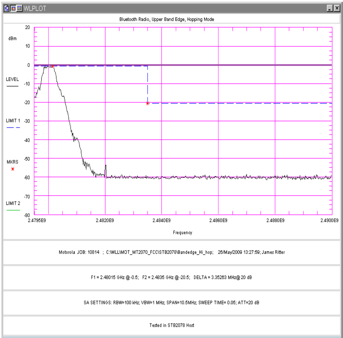
Figure 50. Upper Band Edge Plot, Hopping Mode (in STB2078 Host)
