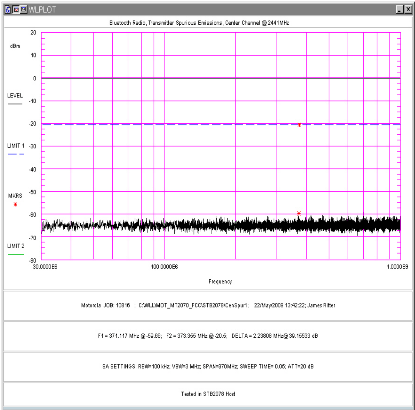
Figure 59 Conducted Spurious Emissions, Mid Channel 30 - 1000MHz (in STB2078 Host)
