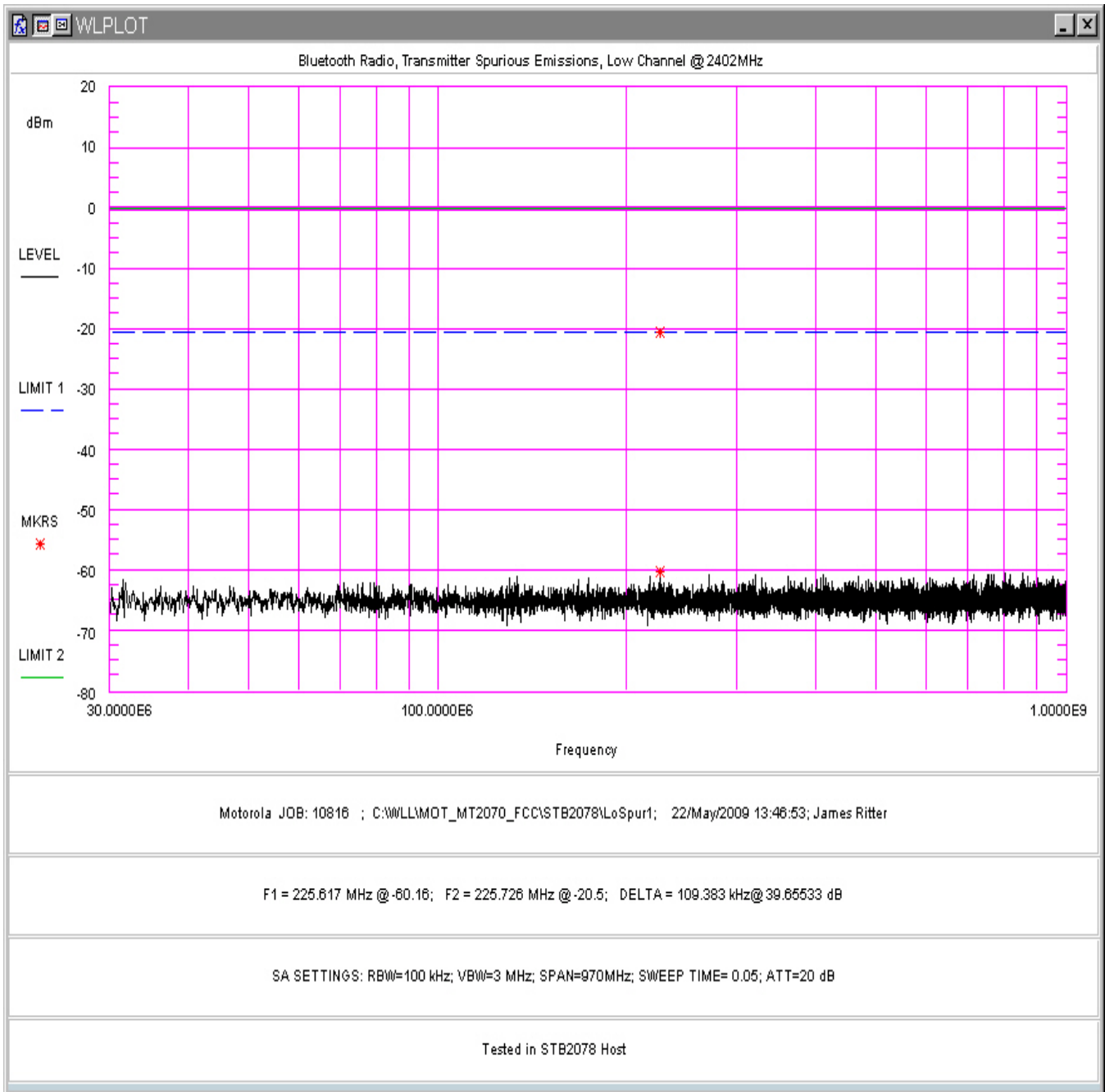
Figure 51. Conducted Spurious Emissions, Low Channel 30 - 1000MHz (in STB2078 Host)
