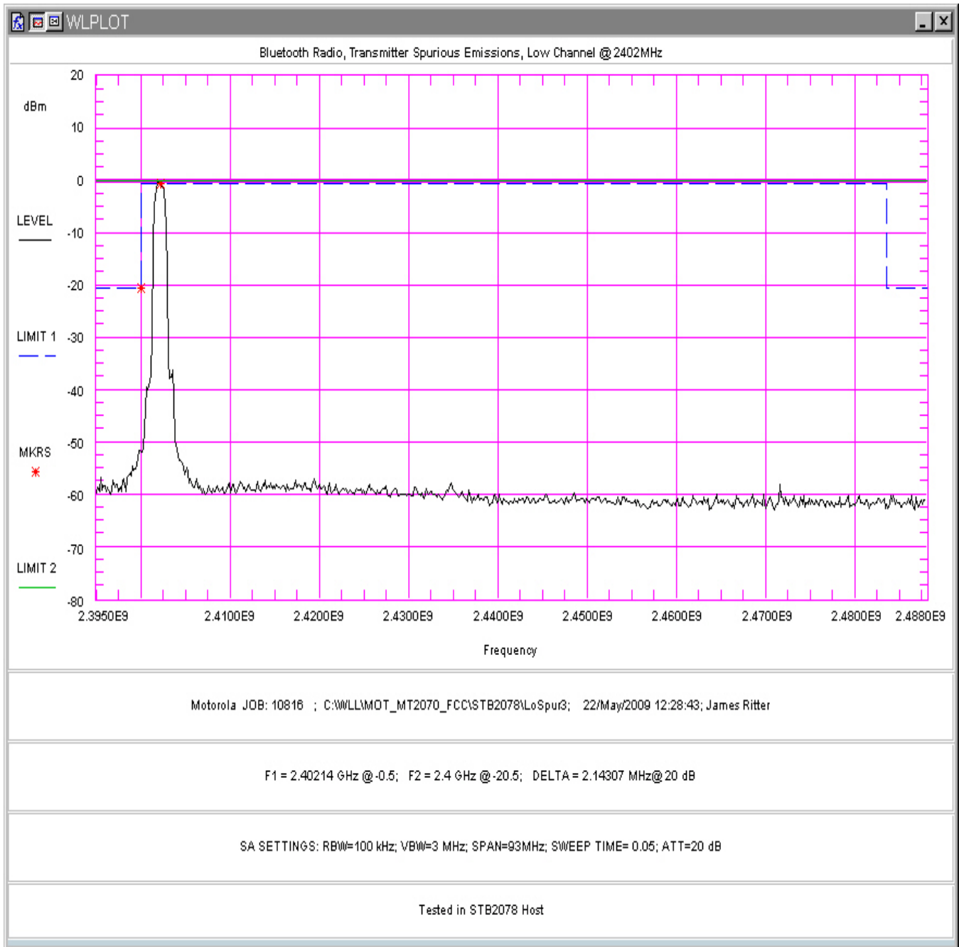
Figure 53. Conducted Spurious Emissions, Low Channel 2.395- 2.488GHz (in STB2078 Host)
