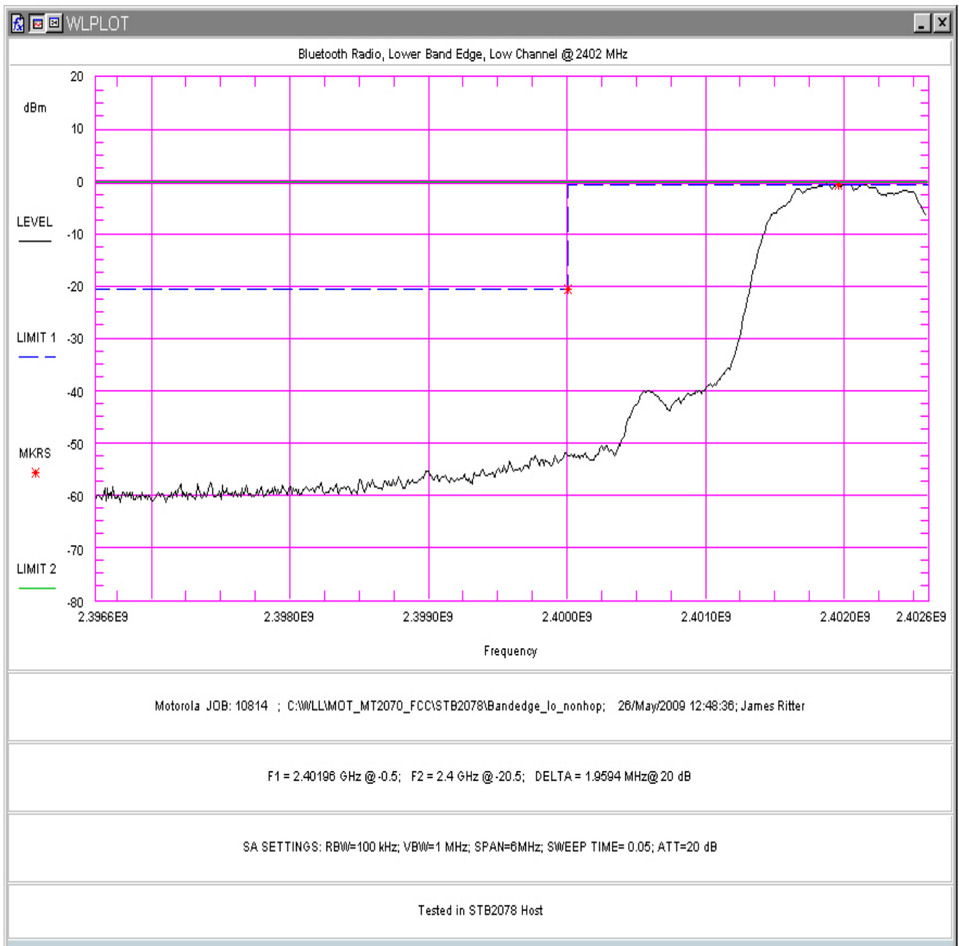
Figure 47. Lower Band Edge Plot, Low Channel (in STB2078 Host)
