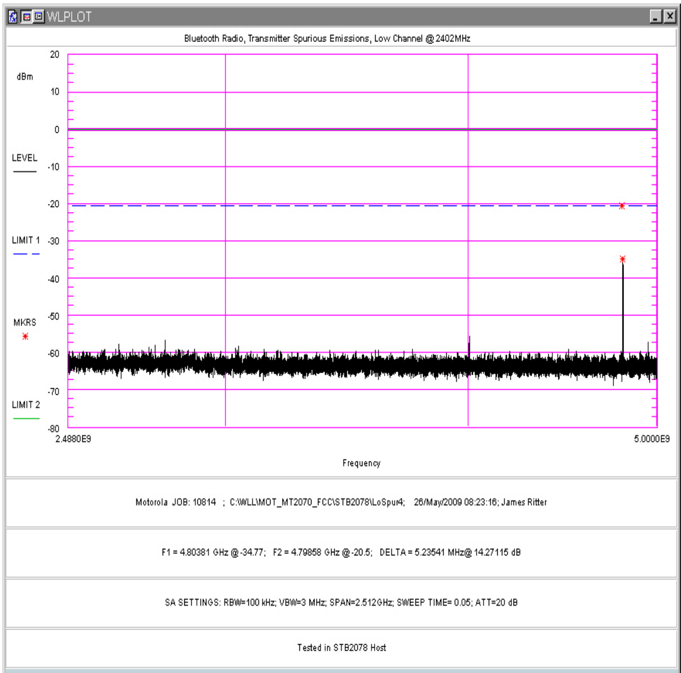
Figure 54. Conducted Spurious Emissions, Low Channel 2.488 – 5 GHz (in STB2078 Host)
