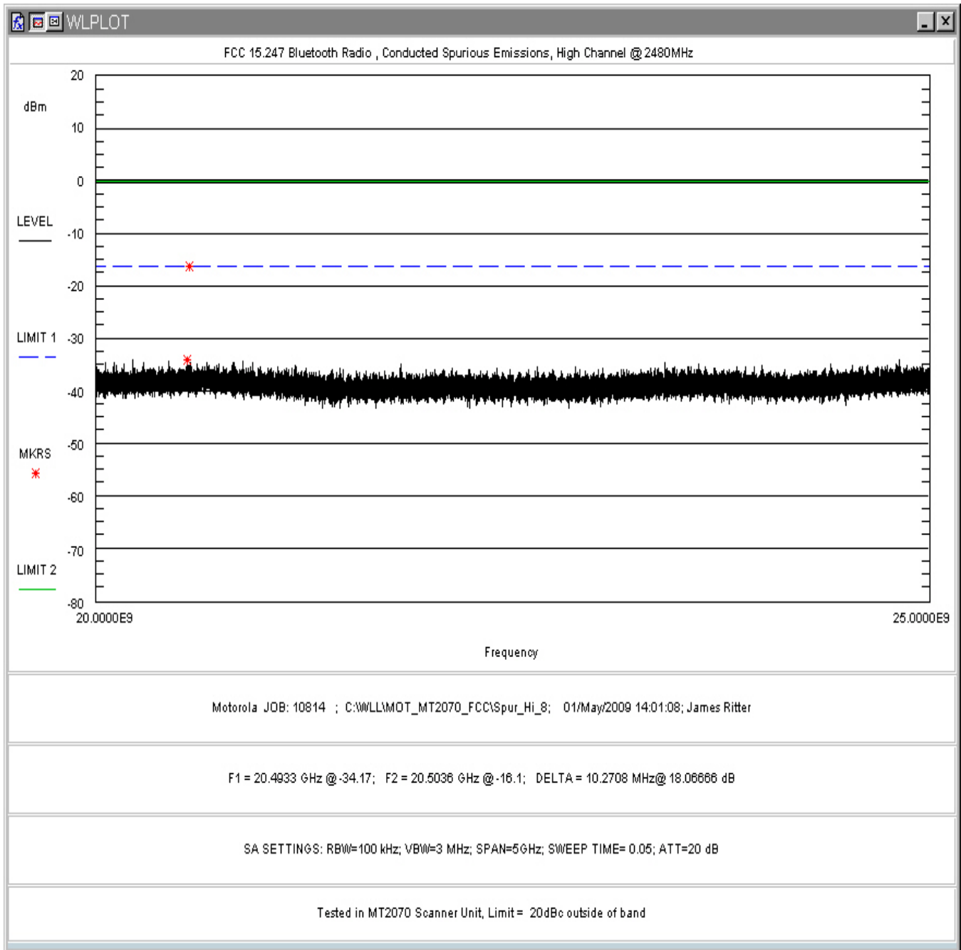
Figure 46. Conducted Spurious Emissions, High Channel 20-25GHz (in MT2070 Host)
