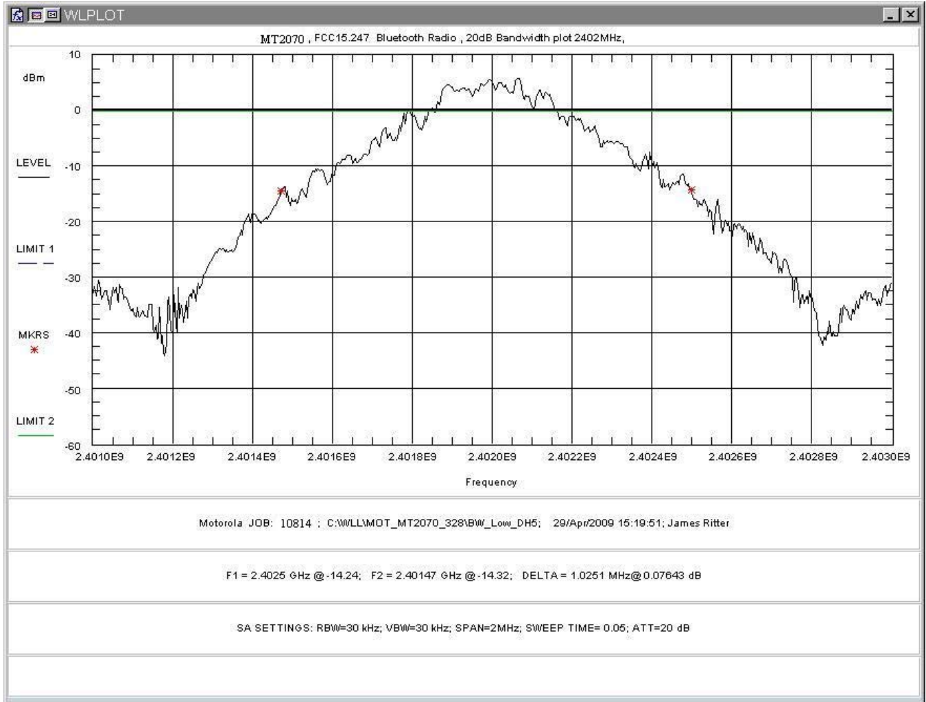
Figure 14. Occupied Bandwidth, Low Channel
