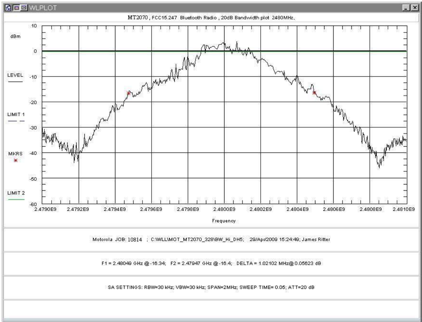
Figure 16. Occupied Bandwidth, High Channel
