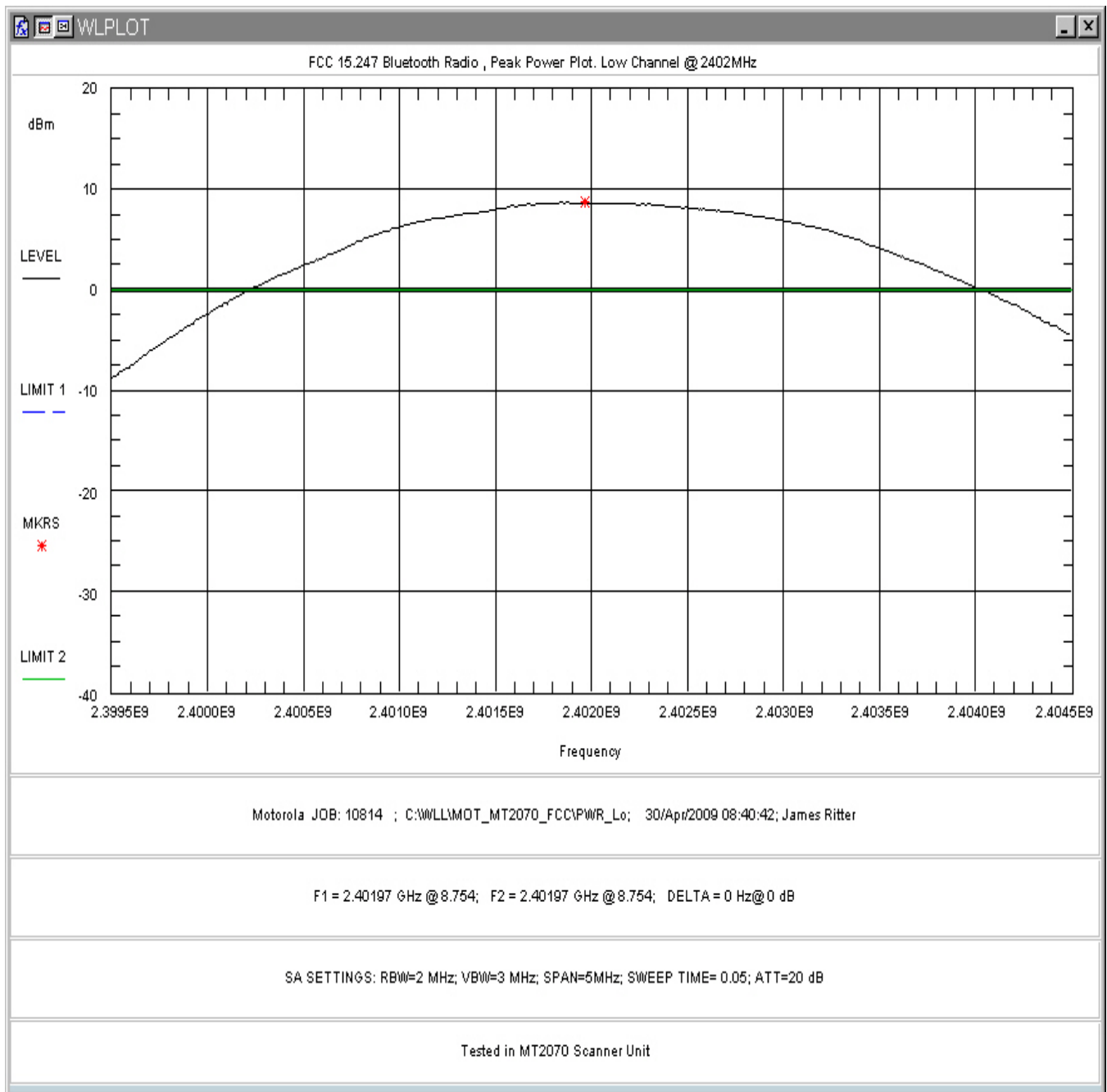
Figure 8. RF Peak Power, Low Channel (In MT2070 Host)
