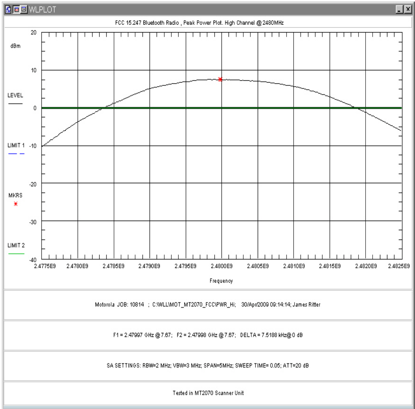
Figure 10. RF Peak Power, High Channel (In MT2070 Host)
