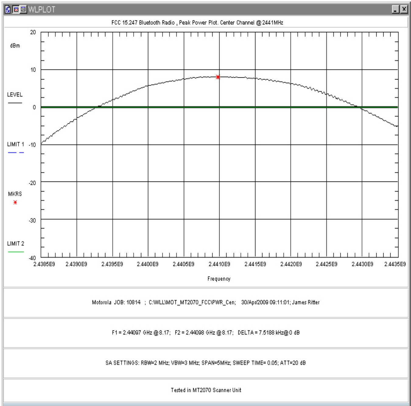
Figure 9. RF Peak Power, Mid Channel (In MT2070 Host)
