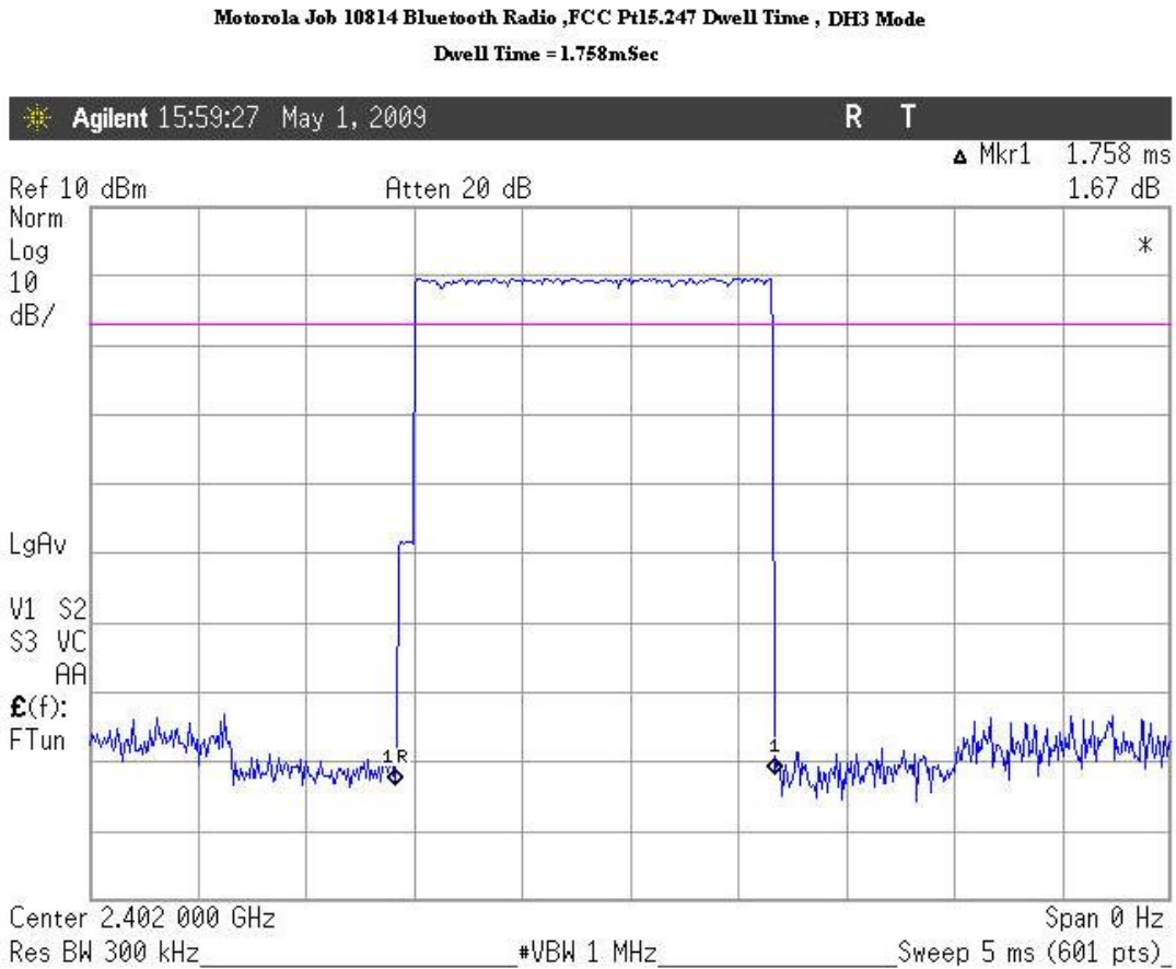
Figure 3. Single Hop Dwell Time DH3 Mode
