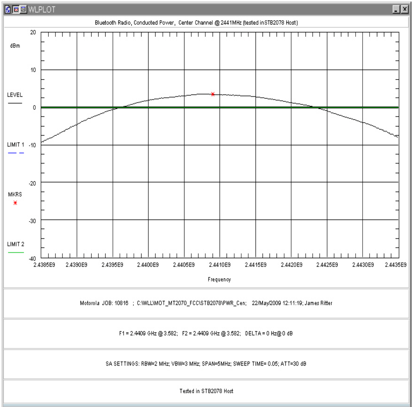
Figure 12. RF Peak Power, Mid Channel (In STB2078 Host)
