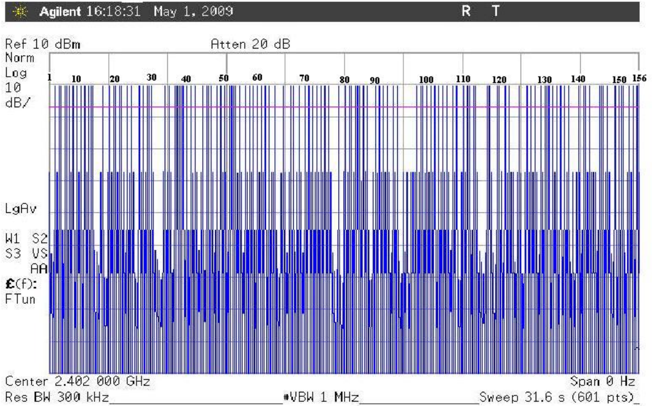
Figure 6. Dwell time per channel over 31.6 Seconds, DH3 Mode
