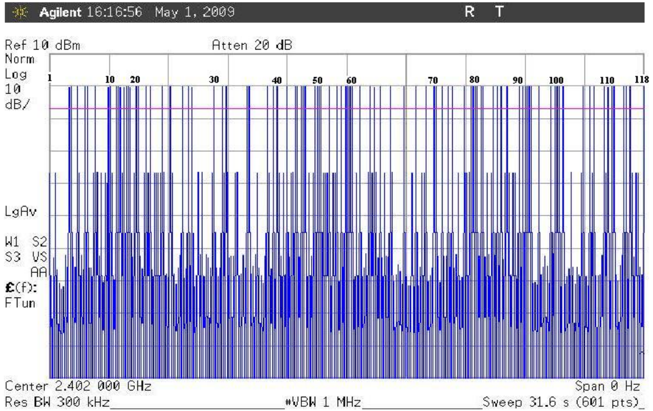
Figure 7. Dwell time per channel over 31.6 Seconds, DH5 Mode
