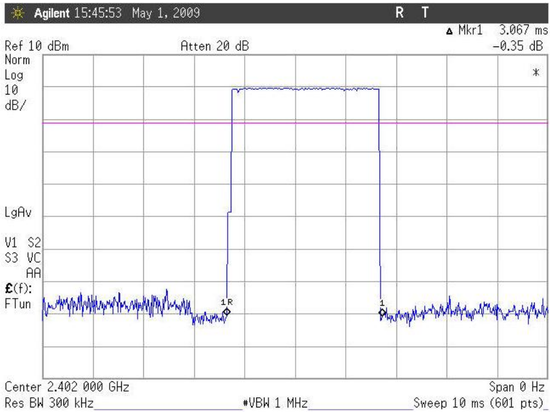
Figure 4. Single Hop Dwell Time DH5 Mode
