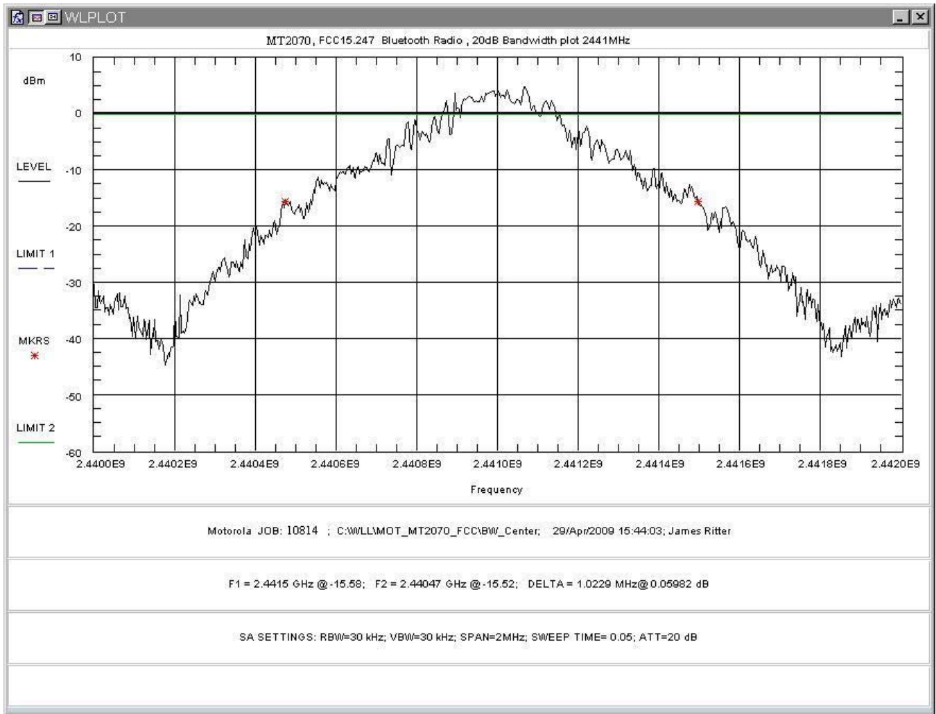
Figure 15. Occupied Bandwidth, Mid Channel
