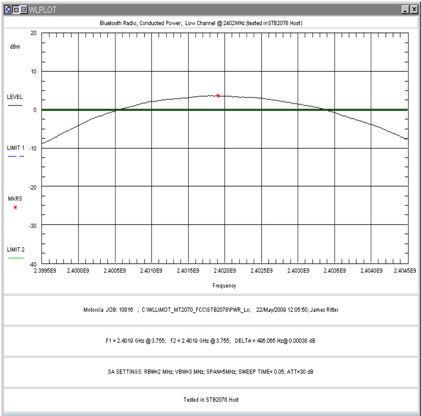
Figure 11. RF Peak Power, Low Channel (In STB2078 Host)
