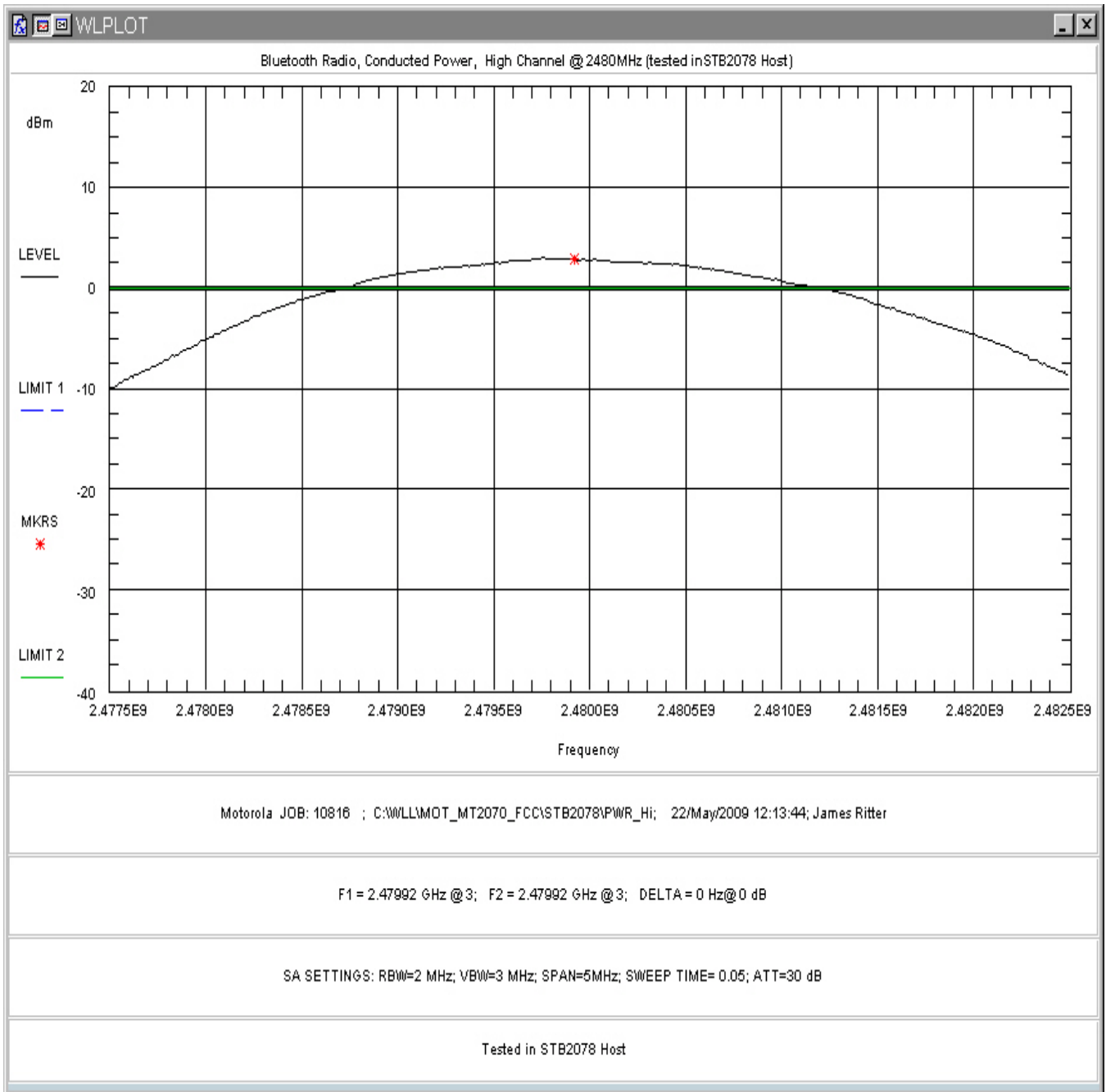
Figure 13.RF Peak Power, High Channel (In STB2078 Host)
