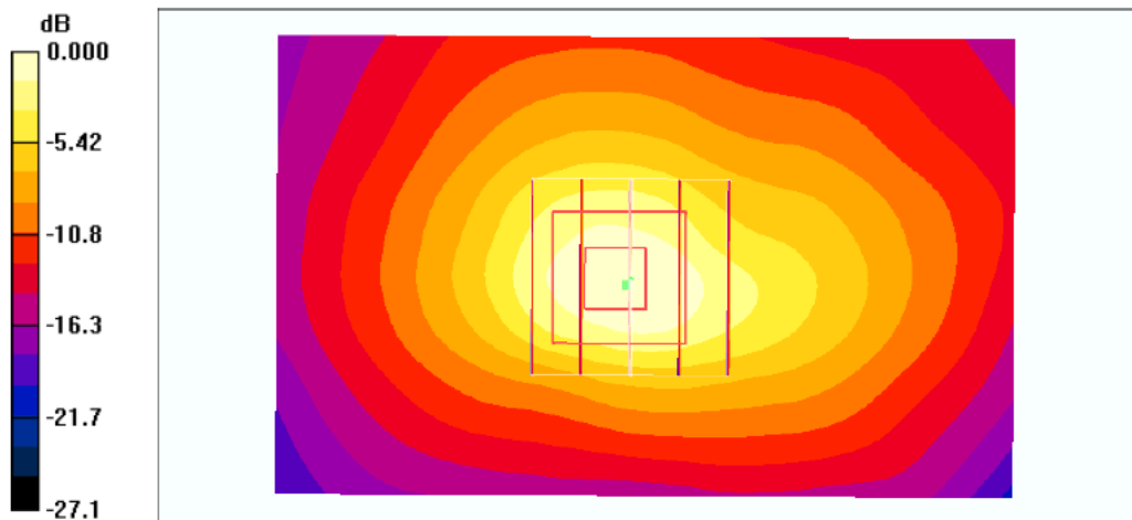
0 dB = 0.123mW/g
