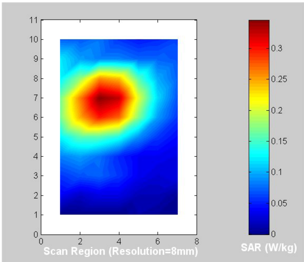
(a) 5.26 GHz normal mode (see Table 3 for the peak 1-g SAR).
