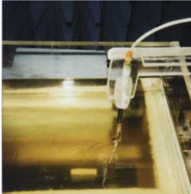
Fig. 6. Photograph of the Askey Corporation 802.11 a/b Cardbus Card inserted into a portable computer (as in Fig. 1) placed with the card edge at 90^\circ and separated from the bottom of the phantom by 0 cm for "end-on" testing of SAR. As in Fig. 5, here too, a Styrofoam block is used under the base to prevent bending of the 2 mm thin base of the phantom.
