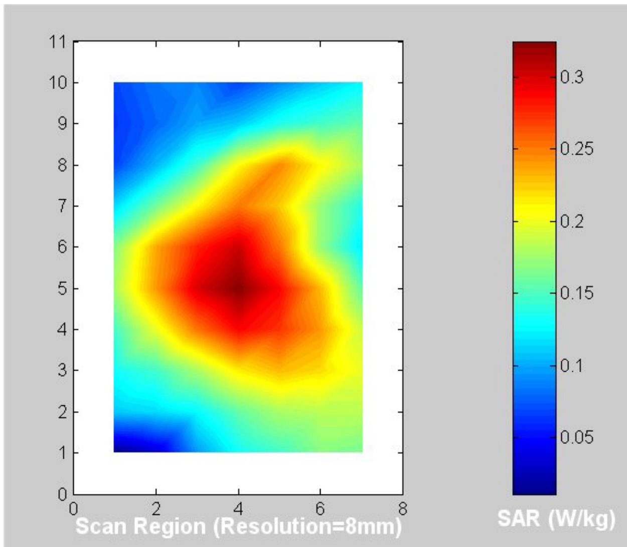
(a) 5.26 GHz normal mode (see Table 7 for the peak 1-g SAR).
