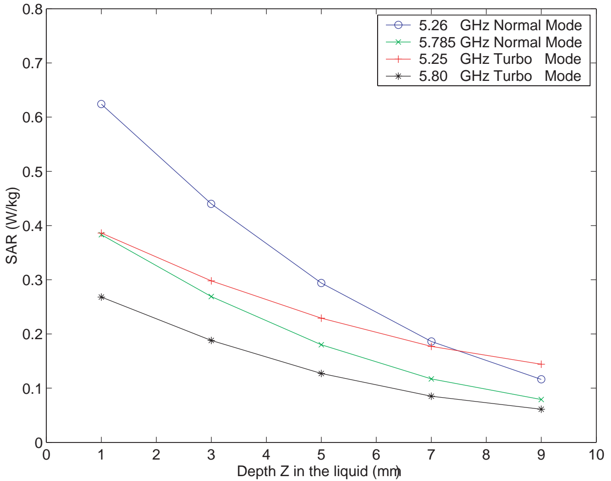
Fig. 16. Plot of the SAR variations as a function of depth Z in the liquid for locations of highest SAR (from Tables 3-6 -- Above-lap position) for Askey 802.11 a/b Cardbus Card.
