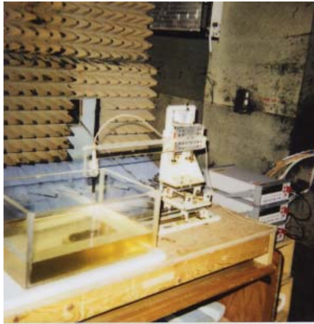
Fig. 3. Photograph of the three-dimensional stepper-motor-controlled SAR measurement system using a planar phantom (see Fig. 5 for a detailed examination of the placement of Askey Corporation 802.11 a/b Cardbus Card relative to this phantom).
