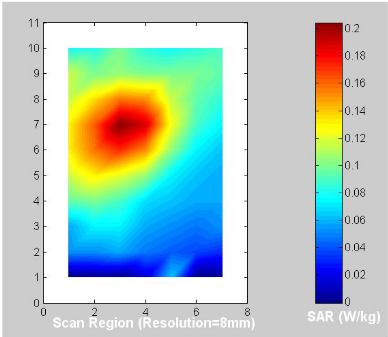
(c) 5.25 GHz turbo mode (see Table 5 for the peak 1-g SAR).
