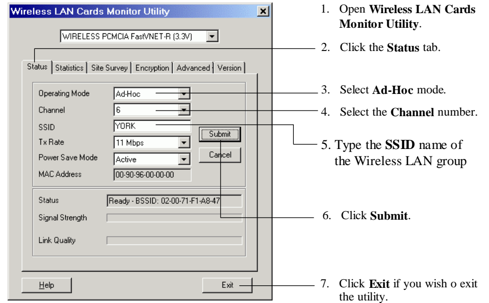
Figure 3-1 Ad-Hoc Configuration
