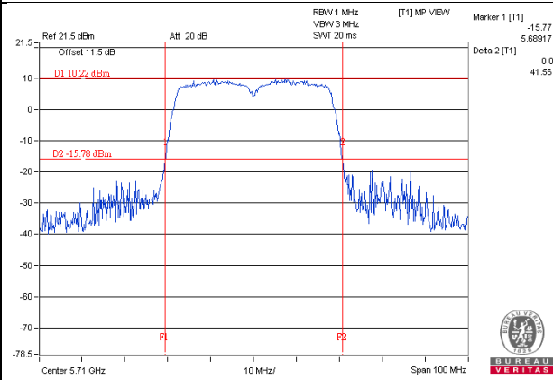
802.11ac (VHT40) / Chain 3 - CH142 (UNII-2C Band)
