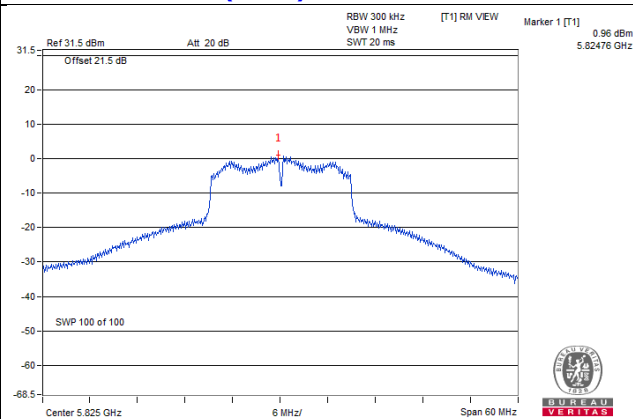
802.11n (HT20)_Chain 0 / CH165
