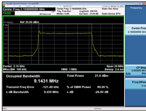
10MHz 64QAM-Lower
