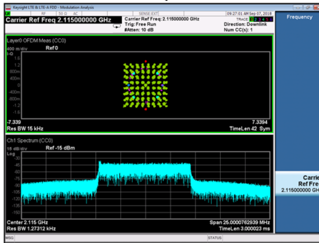
64QAM
