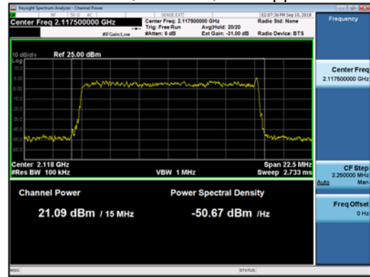
15MHz QPSK+16QAM - Upper
