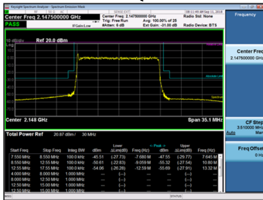
15MHz 64QAM-Lower
