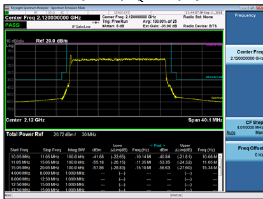
20MHz 64QAM-Lower
