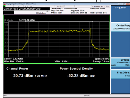
20MHz QPSK+16QAM - Upper
