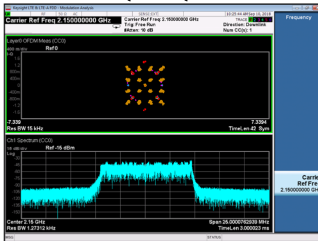
QPSK+16QAM
