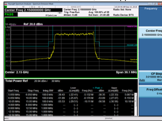
10MHz QPSK+16QAM - Upper
