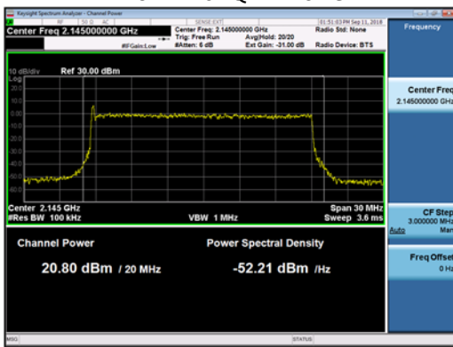
20MHz 64QAM-Lower
