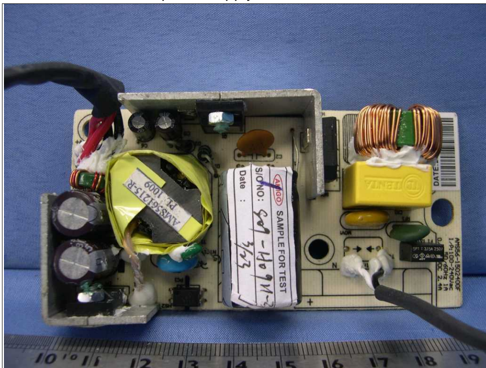
Internal power supply: AMS56-1502400F
