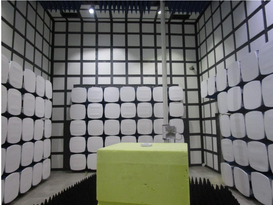
Transmitter Radiated Unwanted Emissions(Above 1GHz)
