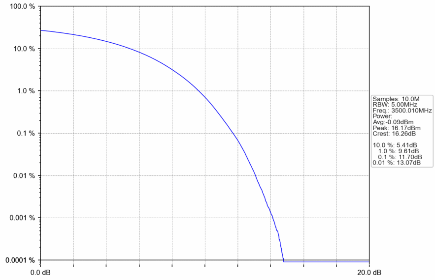
n78e_30kHz_SISO_NTNV_100MHz_CP-OFDM 256 QAM_3500.01MHz_Outer_Full
