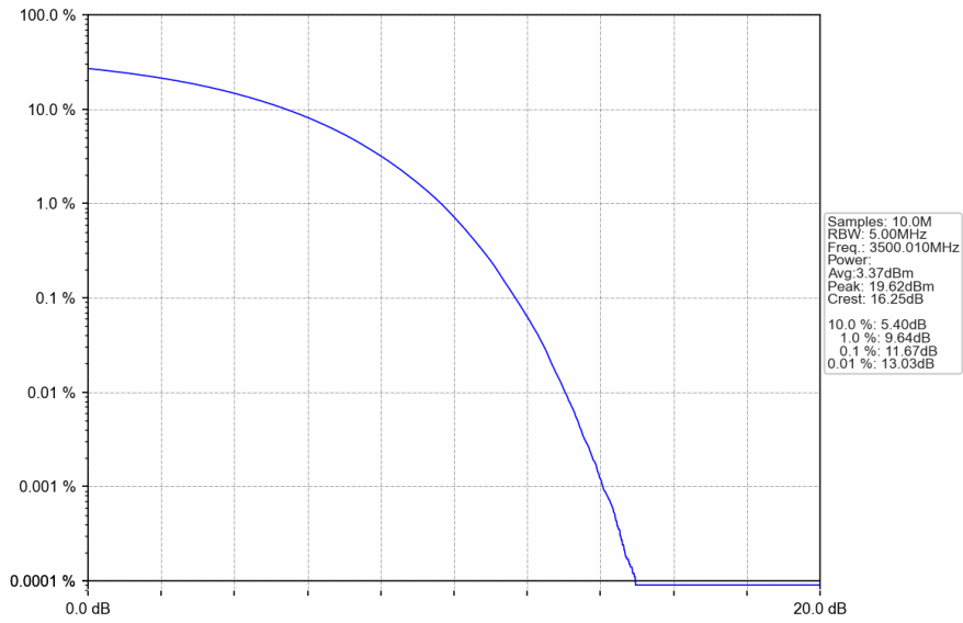
n78e_30kHz_SISO_NTNV_90MHz_CP-OFDM 64 QAM_3500.01MHz_Outer_Full
