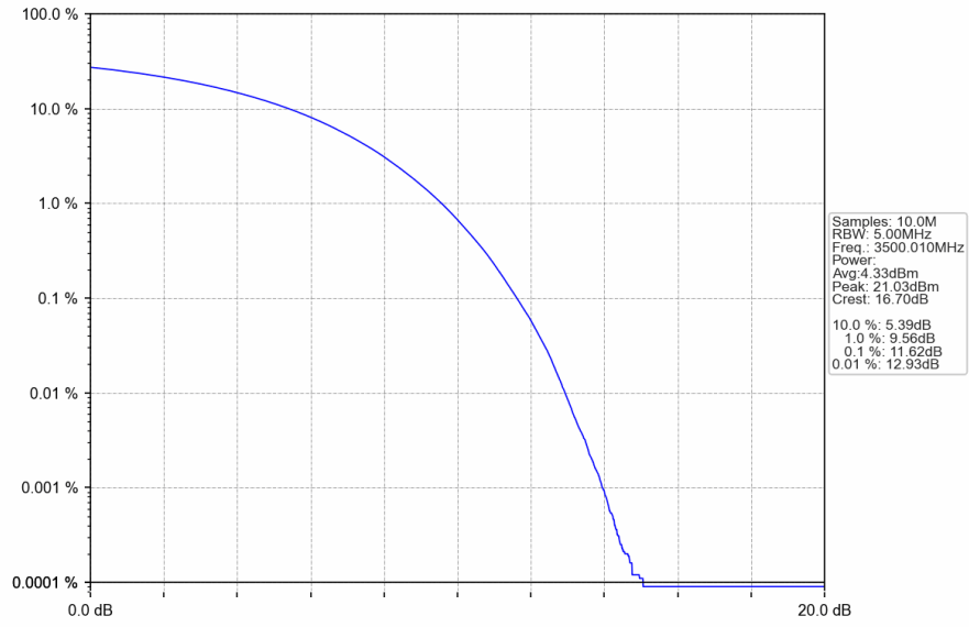
n78e_30kHz_SISO_NTNV_80MHz_CP-OFDM QPSK_3500.01MHz_Outer_Full
