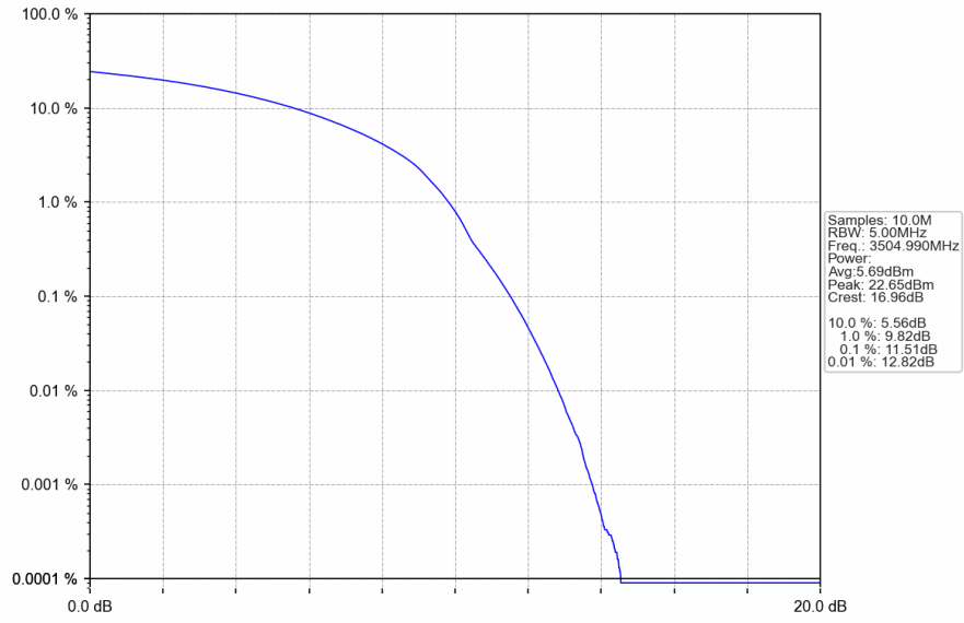
n78e_30kHz_SISO_NTNV_90MHz_DFT-s-OFDM QPSK_3504.99MHz_Outer_Full
