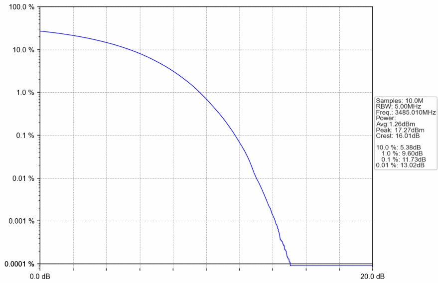
n78e_30kHz_SISO_NTNV_70MHz_CP-OFDM 256 QAM_3485.01MHz_Outer_Full
