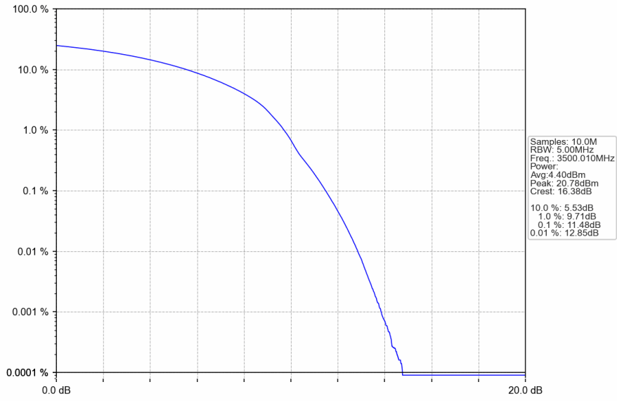
n78e_30kHz_SISO_NTNV_90MHz_DFT-s-OFDM_64_QAM_3500.01MHz_Outer_Full
