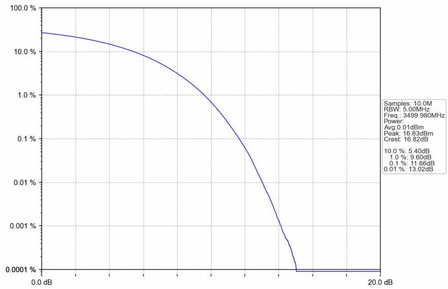
n78e_30kHz_SISO_NTNV_100MHz_CP-OFDM 256 QAM_3499.98MHz_Outer_Full
