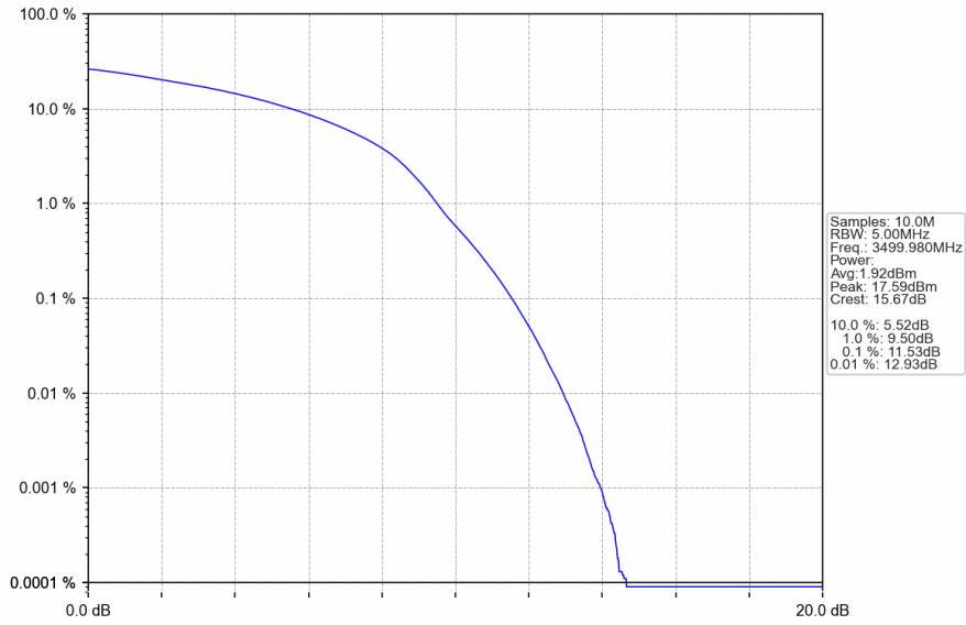
n78e_30kHz_SISO_NTNV_100MHz_DFT-s-OFDM 256 QAM_3499.98MHz_Outer_Full
