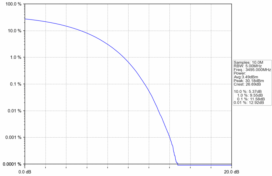
n78e_30kHz_SISO_NTNV_90MHz_CP-OFDM 64 QAM_3495MHz_Outer_Full
