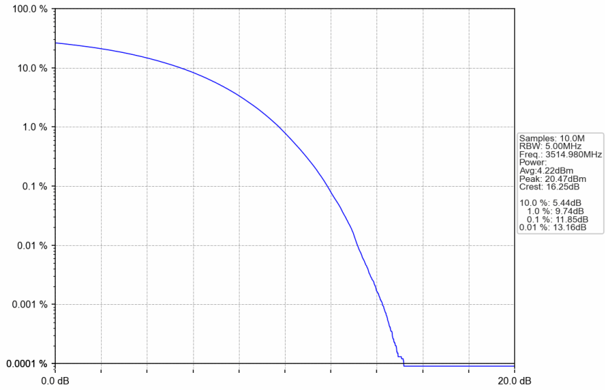
n78e_30kHz_SISO_NTNV_70MHz_CP-OFDM 64 QAM_3514.98MHz_Outer_Full
