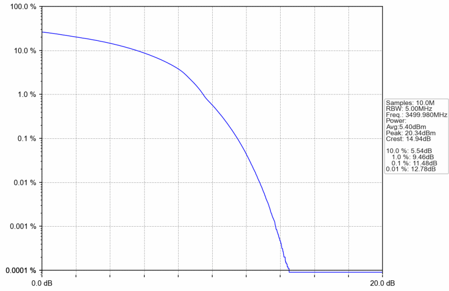
n78e_30kHz_SISO_NTNV_100MHz_DFT-s-OFDM QPSK_3499.98MHz_Outer_Full
