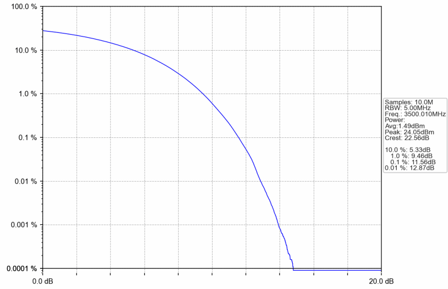
n78e_30kHz_SISO_NTNV_70MHz_CP-OFDM 256 QAM_3500.01MHz_Outer_Full
