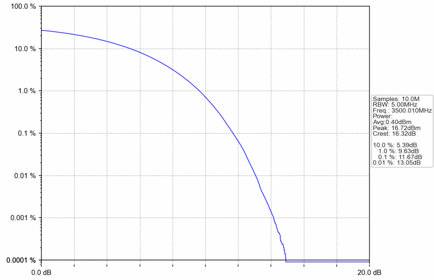
n78e_30kHz_SISO_NTNV_90MHz_CP-OFDM_256_QAM_3500.01MHz_Outer_Full
