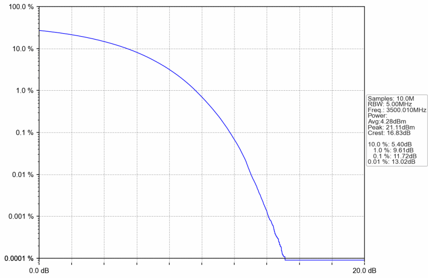
n78e_30kHz_SISO_NTNV_70MHz_CP-OFDM 64 QAM_3500.01MHz_Outer_Full
