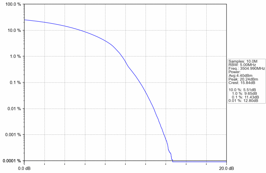
n78e_30kHz_SISO_NTNV_90MHz_DFT-s-OFDM_64_QAM_3504.99MHz_Outer_Full
