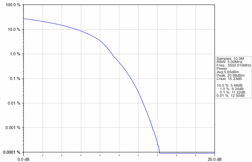
n78e_30kHz_SISO_NTNV_100MHz_DFT-s-OFDM QPSK_3500.01MHz_Outer_Full
