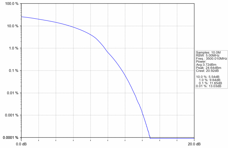
n78e_30kHz_SISO_NTNV_100MHz_DFT-s-OFDM 64 QAM_3500.01MHz_Outer_Full
