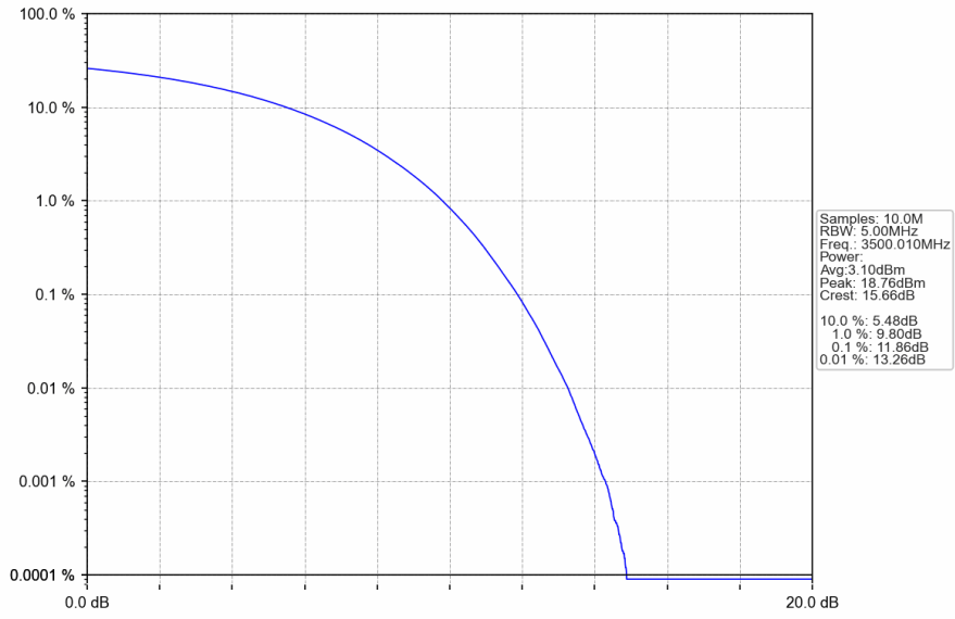
n78e_30kHz_SISO_NTNV_100MHz_CP-OFDM QPSK_3500.01MHz_Outer_Full
