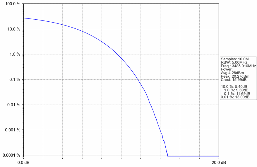
n78e_30kHz_SISO_NTNV_70MHz_CP-OFDM 64 QAM_3485.01MHz_Outer_Full
