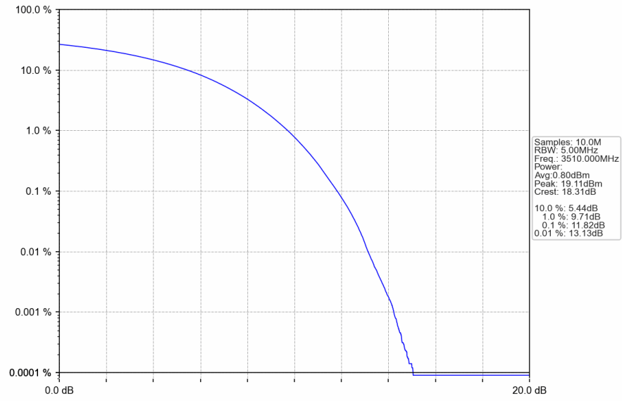
n78e_30kHz_SISO_NTNV_80MHz_CP-OFDM_256_QAM_3510MHz_Outer_Full
