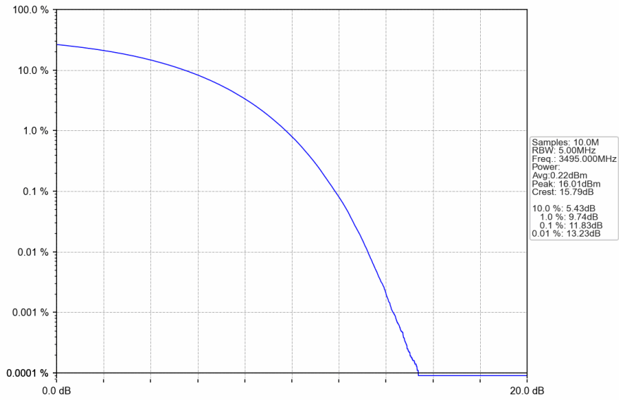
n78e_30kHz_SISO_NTNV_90MHz_CP-OFDM 256 QAM_3495MHz_Outer_Full
