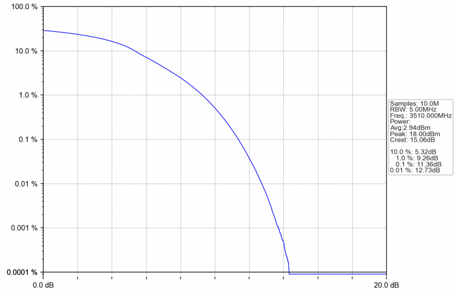
n78e_30kHz_SISO_NTNV_80MHz_DFT-s-OFDM_256_QAM_3510MHz_Outer_Full
