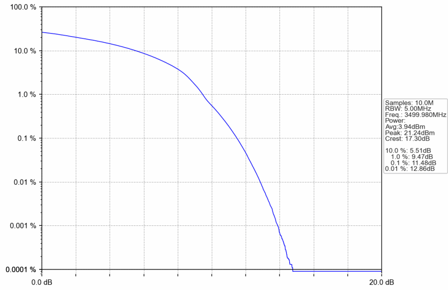
n78e_30kHz_SISO_NTNV_100MHz_DFT-s-OFDM 64 QAM_3499.98MHz_Outer_Full
