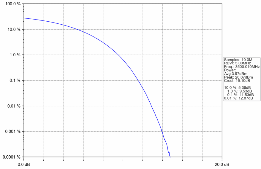
n78e_30kHz_SISO_NTNV_90MHz_CP-OFDM_QPSK_3500.01MHz_Outer_Full
