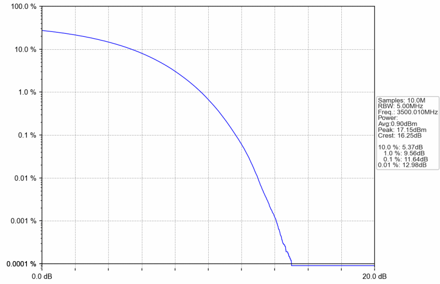
n78e_30kHz_SISO_NTNV_80MHz_CP-OFDM_256_QAM_3500.01MHz_Outer_Full
