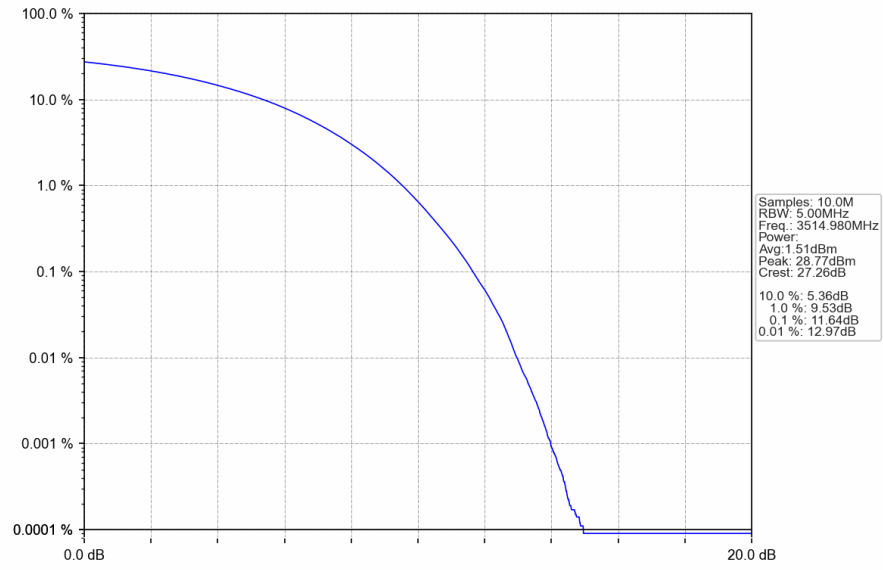
n78e_30kHz_SISO_NTNV_70MHz_CP-OFDM 256 QAM_3514.98MHz_Outer_Full
