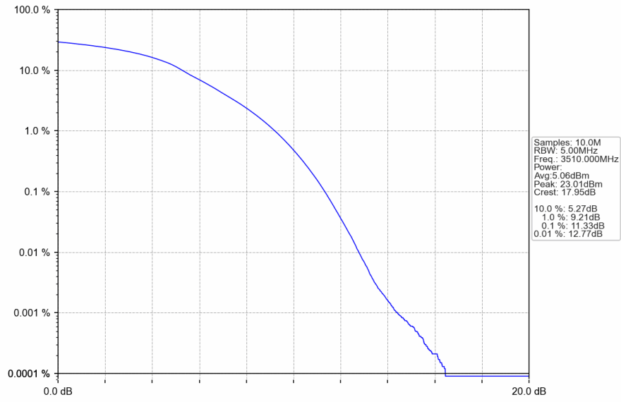
n78e_30kHz_SISO_NTNV_80MHz_DFT-s-OFDM_64_QAM_3510MHz_Outer_Full
