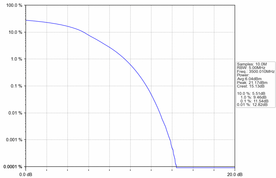
n78e_30kHz_SISO_NTNV_80MHz_DFT-s-OFDM QPSK_3500.01MHz_Outer_Full
