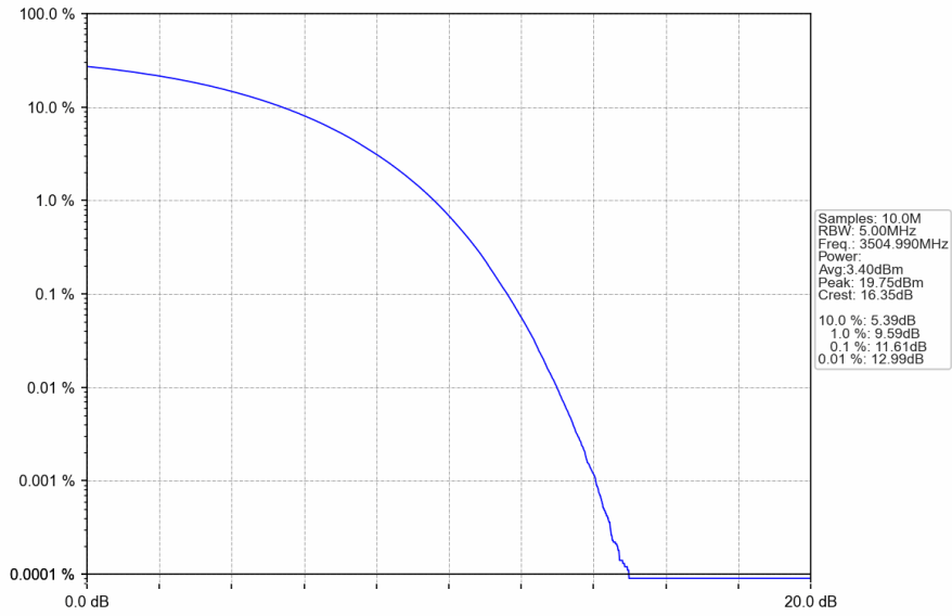
n78e_30kHz_SISO_NTNV_90MHz_CP-OFDM 64 QAM_3504.99MHz_Outer_Full
