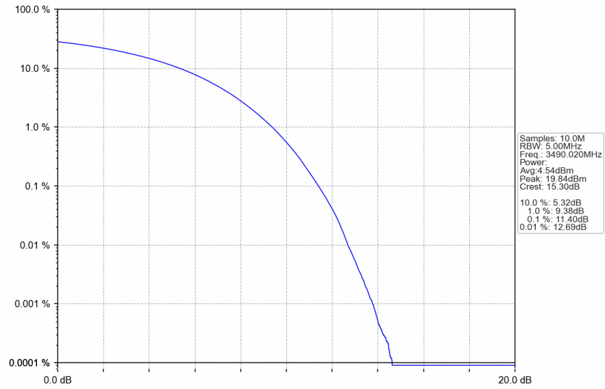
n78e_30kHz_SISO_NTNV_80MHz_CP-OFDM_QPSK_3490.02MHz_Outer_Full
