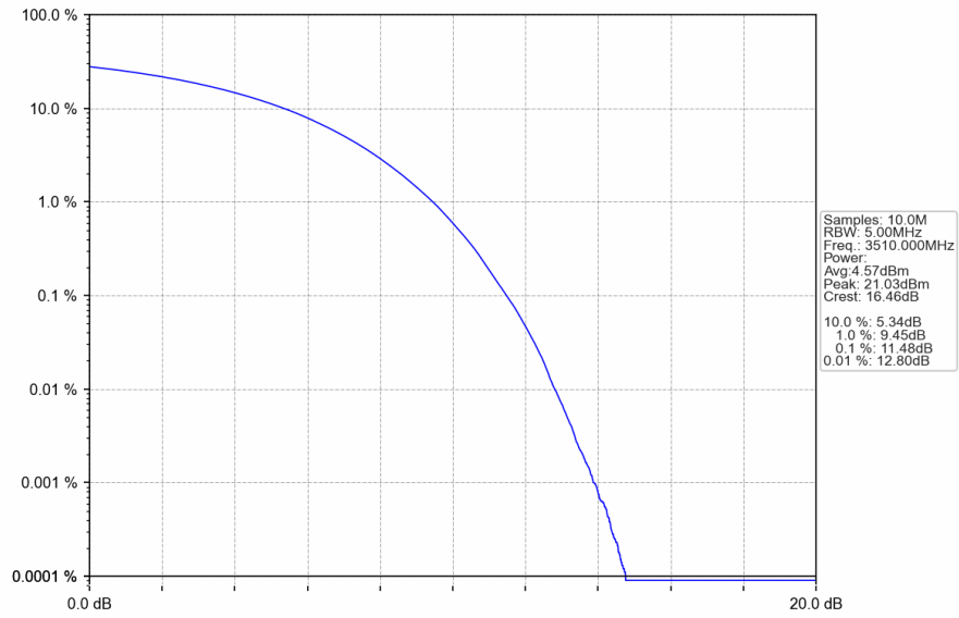
n78e_30kHz_SISO_NTNV_80MHz_CP-OFDM QPSK_3510MHz_Outer_Full
