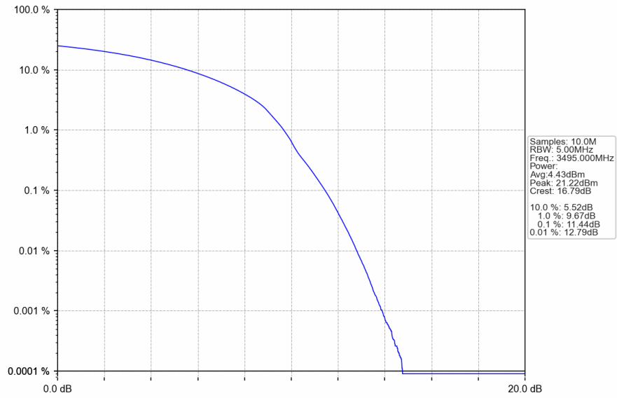
n78e_30kHz_SISO_NTNV_90MHz_DFT-s-OFDM 64 QAM_3495MHz_Outer_Full
