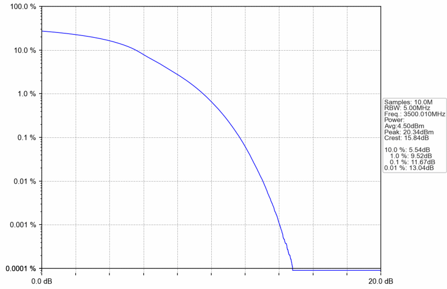
n78e_30kHz_SISO_NTNV_80MHz_DFT-s-OFDM_64_QAM_3500.01MHz_Outer_Full
