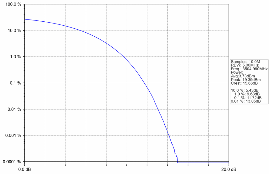
n78e_30kHz_SISO_NTNV_90MHz_CP-OFDM_QPSK_3504.99MHz_Outer_Full
