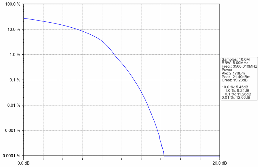
n78e_30kHz_SISO_NTNV_100MHz_DFT-s-OFDM_256_QAM_3500.01MHz_Outer_Full
