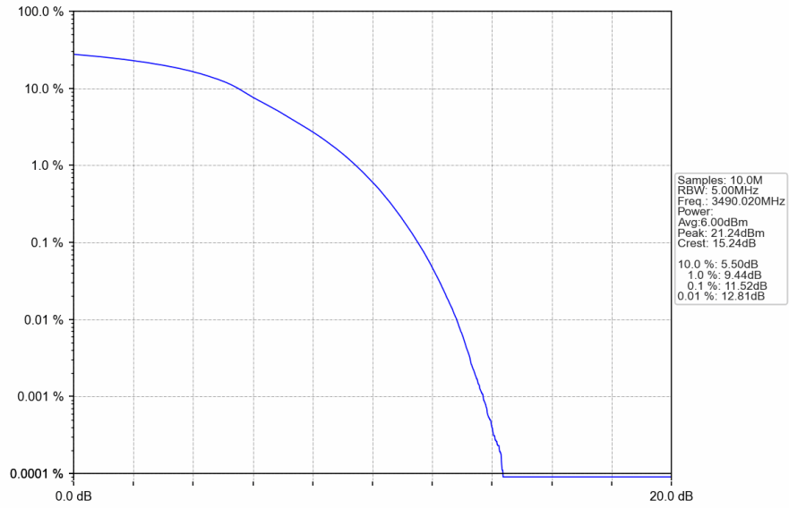
n78e_30kHz_SISO_NTNV_80MHz_DFT-s-OFDM QPSK_3490.02MHz_Outer_Full
