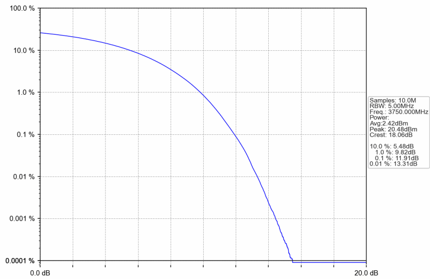
n78a_30kHz_SISO_NTNV_100MHz_CP-OFDM 64 QAM_3750MHz_Outer_Full
