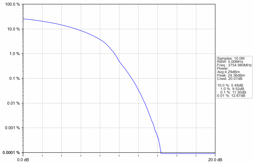
n78a_30kHz_SISO_NTNV_90MHz_DFT-s-OFDM_64_QAM_3754.98MHz_Outer_Full
