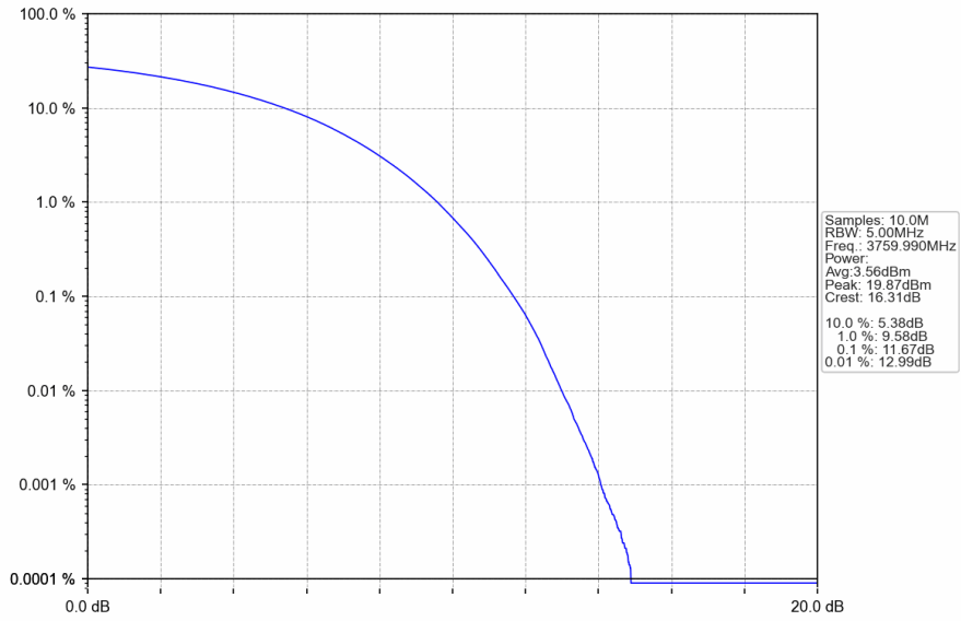
n78a_30kHz_SISO_NTNV_80MHz_CP-OFDM 64 QAM_3759.99MHz_Outer_Full
