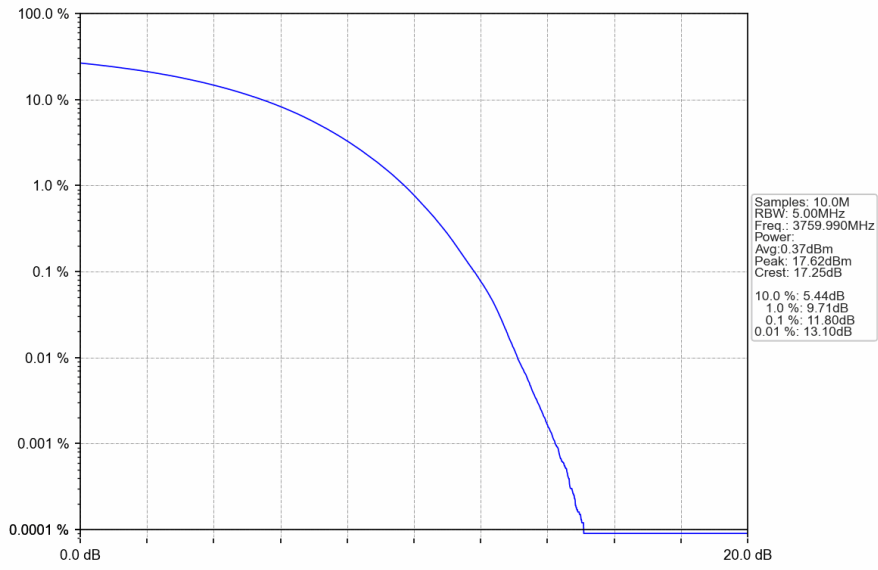
n78a_30kHz_SISO_NTNV_80MHz_CP-OFDM 256 QAM_3759.99MHz_Outer_Full
