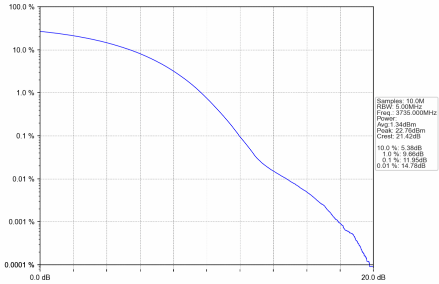
n78a_30kHz_SISO_NTNV_70MHz_CP-OFDM 256 QAM_3735MHz_Outer_Full
