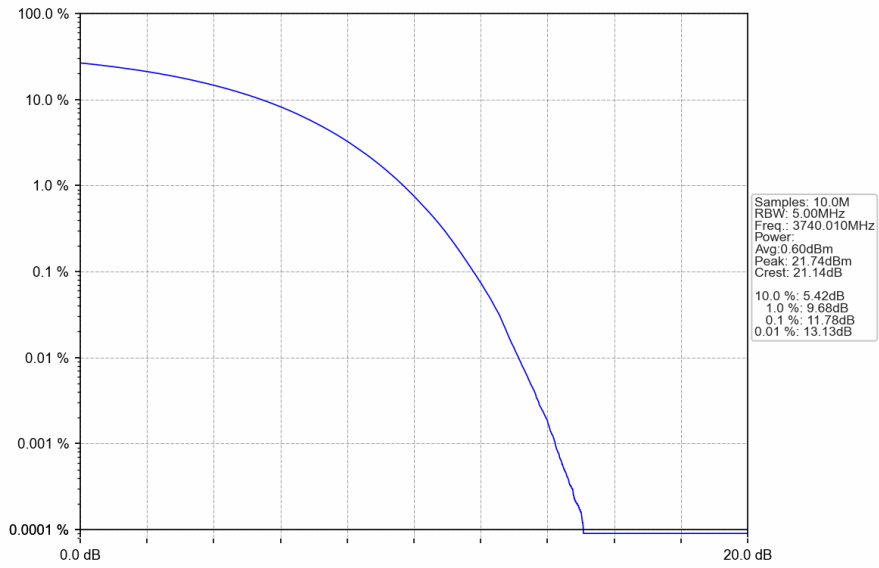
n78a_30kHz_SISO_NTNV_80MHz_CP-OFDM 256 QAM_3740.01MHz_Outer_Full
