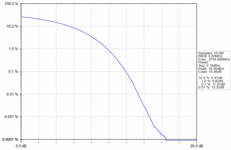
n78a_30kHz_SISO_NTNV_90MHz_CP-OFDM 256 QAM_3754.98MHz_Outer_Full
