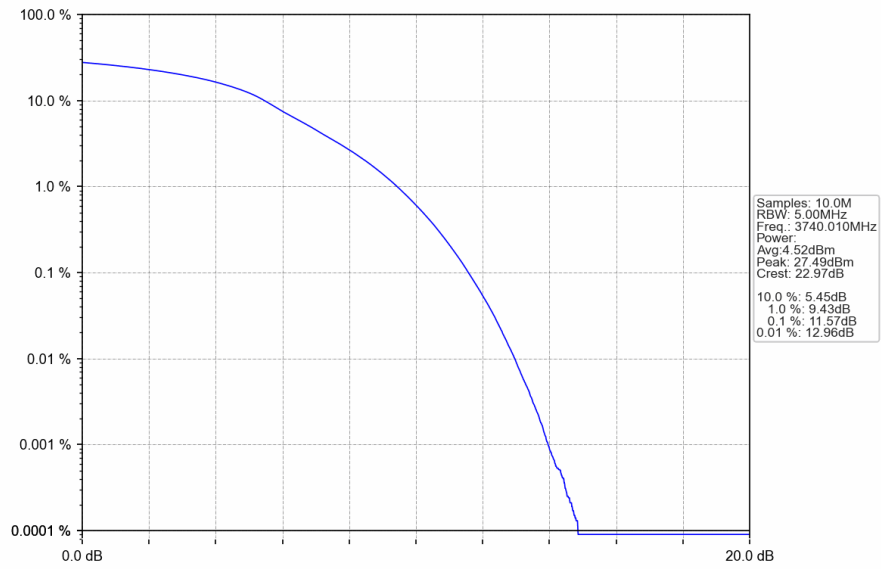
n78a_30kHz_SISO_NTNV_80MHz_DFT-s-OFDM 64 QAM_3740.01MHz_Outer_Full
