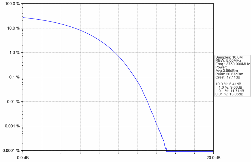
n78a_30kHz_SISO_NTNV_90MHz_CP-OFDM QPSK_3750MHz_Outer_Full
