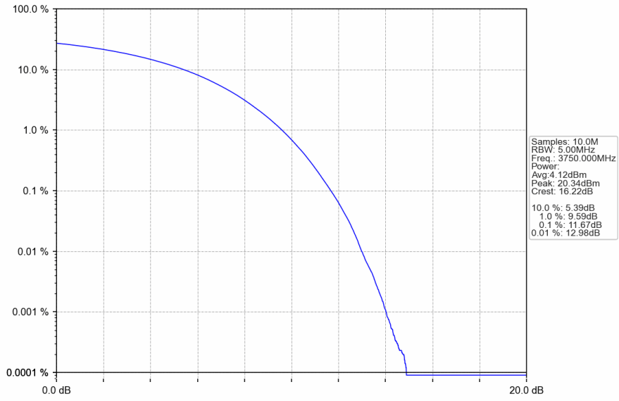
n78a_30kHz_SISO_NTNV_80MHz_CP-OFDM_QPSK_3750MHz_Outer_Full
