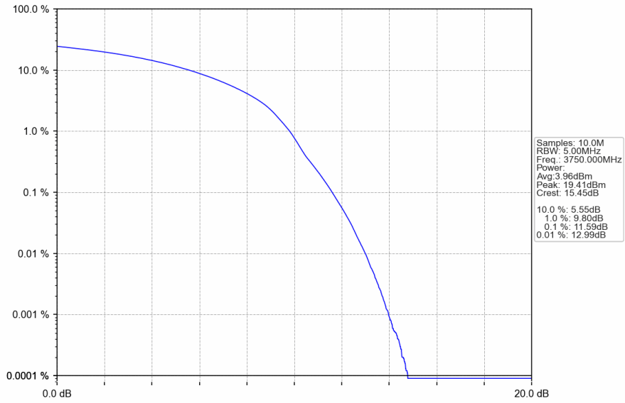
n78a_30kHz_SISO_NTNV_90MHz_DFT-s-OFDM_64_QAM_3750MHz_Outer_Full
