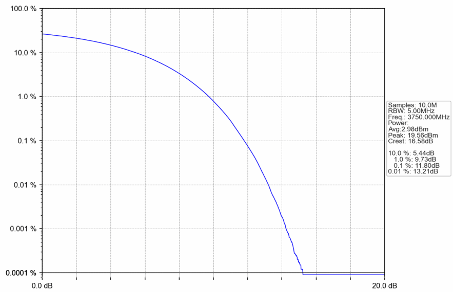
n78a_30kHz_SISO_NTNV_90MHz_CP-OFDM 64 QAM_3750MHz_Outer_Full
