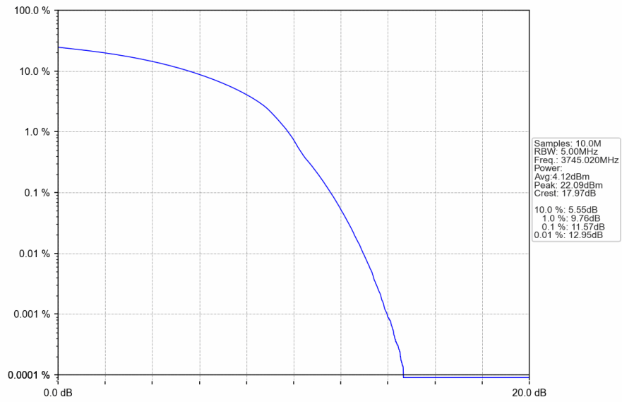
n78a_30kHz_SISO_NTNV_90MHz_DFT-s-OFDM 64 QAM_3745.02MHz_Outer_Full
