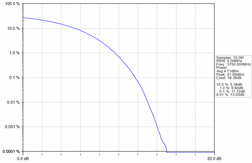
n78a_30kHz_SISO_NTNV_70MHz_CP-OFDM QPSK_3750MHz_Outer_Full
