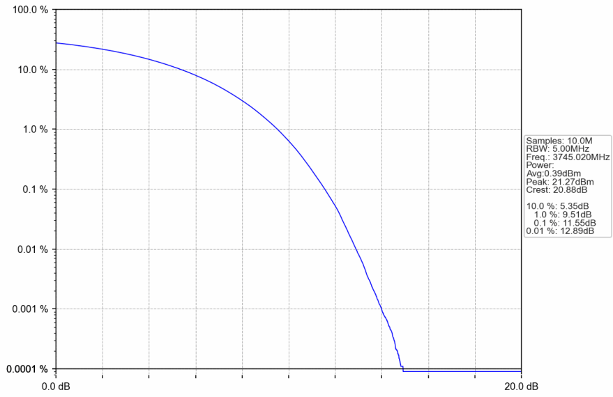
n78a_30kHz_SISO_NTNV_90MHz_CP-OFDM 256 QAM_3745.02MHz_Outer_Full
