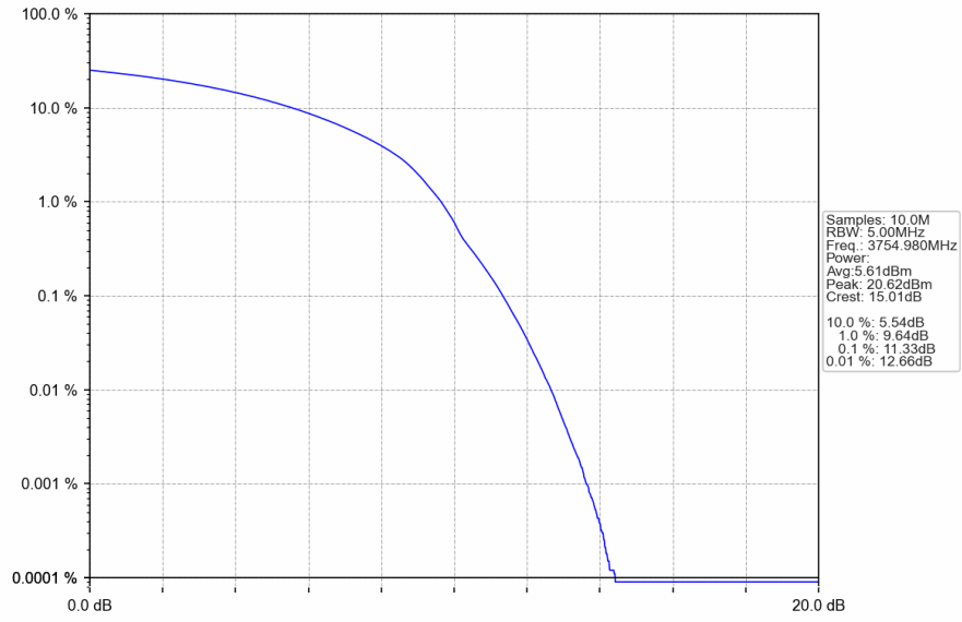
n78a_30kHz_SISO_NTNV_90MHz_DFT-s-OFDM QPSK_3754.98MHz_Outer_Full
