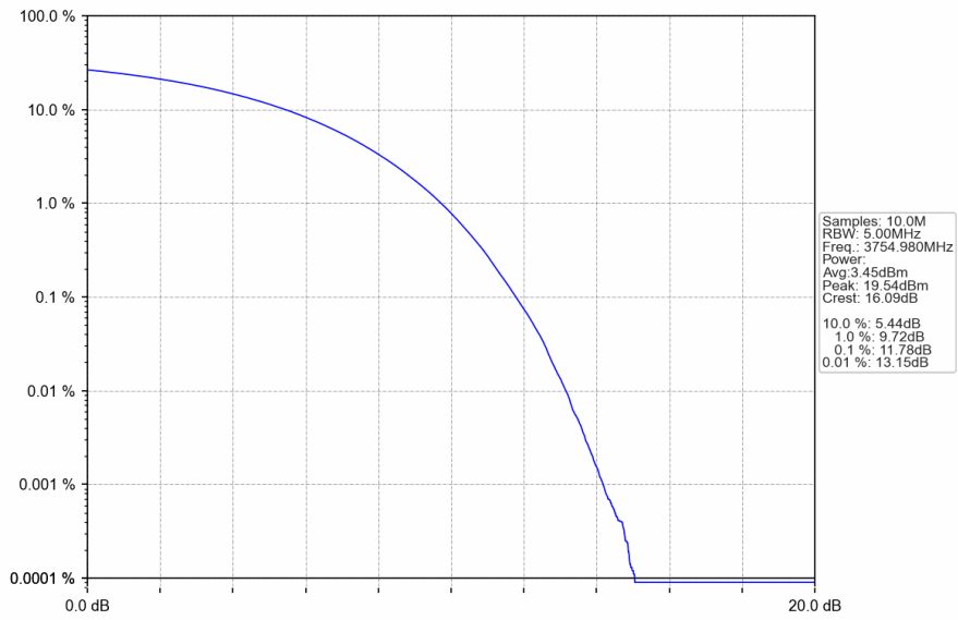
n78a_30kHz_SISO_NTNV_90MHz_CP-OFDM QPSK_3754.98MHz_Outer_Full
