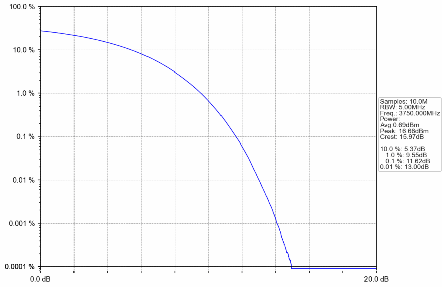
n78a_30kHz_SISO_NTNV_80MHz_CP-OFDM 256 QAM_3750MHz_Outer_Full
