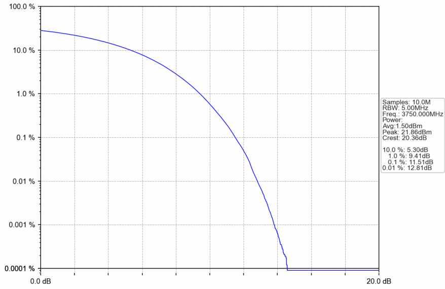
n78a_30kHz_SISO_NTNV_70MHz_CP-OFDM 256 QAM_3750MHz_Outer_Full
