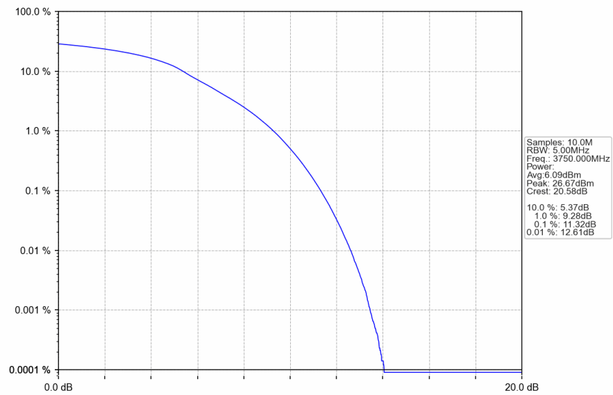
n78a_30kHz_SISO_NTNV_80MHz_DFT-s-OFDM QPSK_3750MHz_Outer_Full
