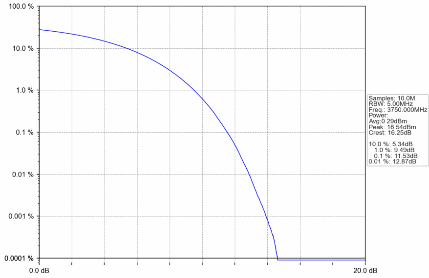
n78a_30kHz_SISO_NTNV_90MHz_CP-OFDM 256 QAM_3750MHz_Outer_Full
