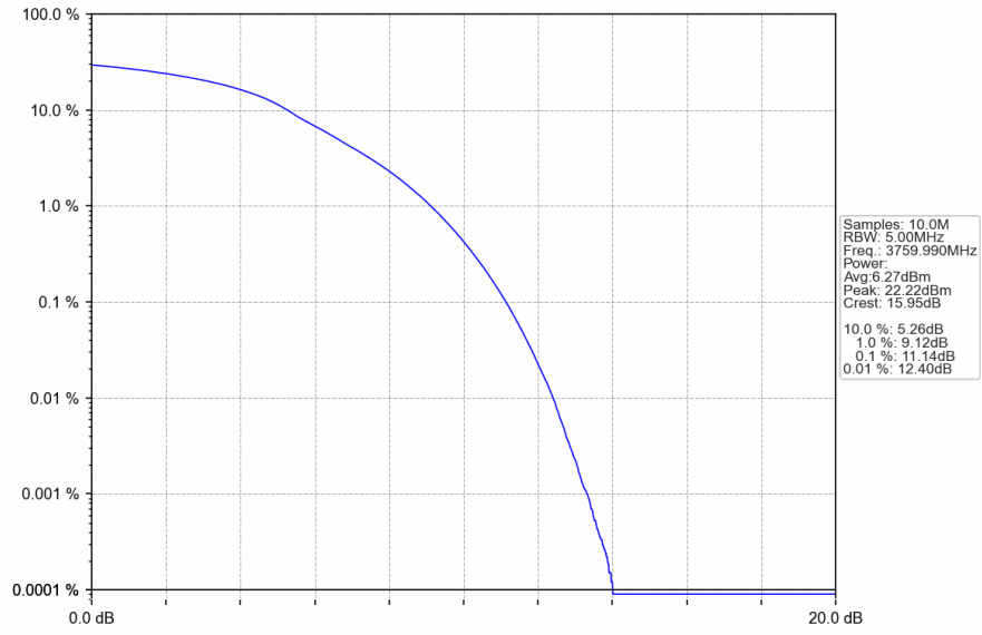
n78a_30kHz_SISO_NTNV_80MHz_DFT-s-OFDM QPSK_3759.99MHz_Outer_Full
