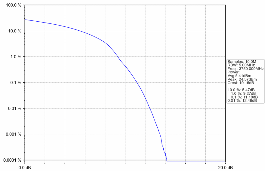
n78a_30kHz_SISO_NTNV_100MHz_DFT-s-OFDM QPSK_3750MHz_Outer_Full
