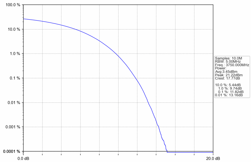
n78a_30kHz_SISO_NTNV_80MHz_CP-OFDM 64 QAM_3750MHz_Outer_Full
