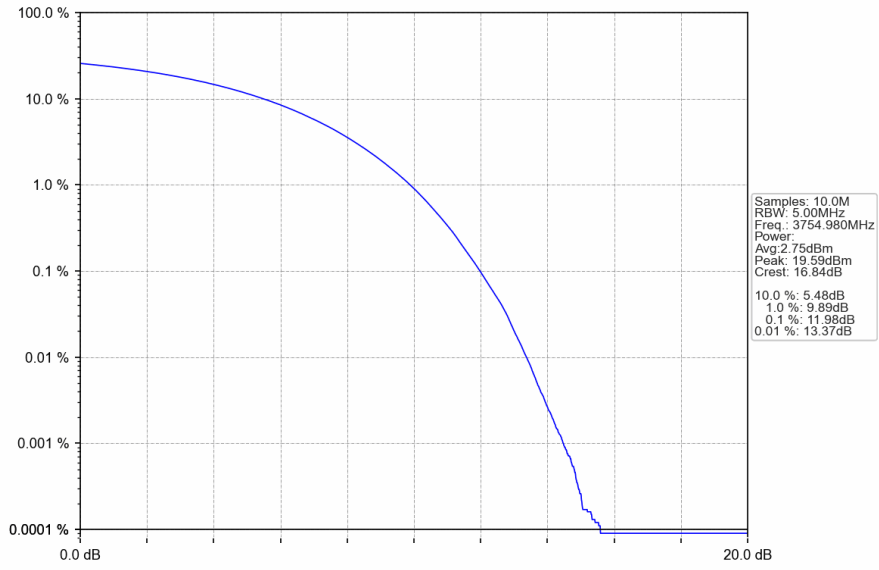
n78a_30kHz_SISO_NTNV_90MHz_CP-OFDM 64 QAM_3754.98MHz_Outer_Full
