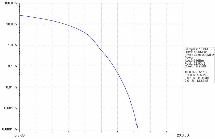
n78a_30kHz_SISO_NTNV_100MHz_DFT-s-OFDM_64_QAM_3750MHz_Outer_Full
