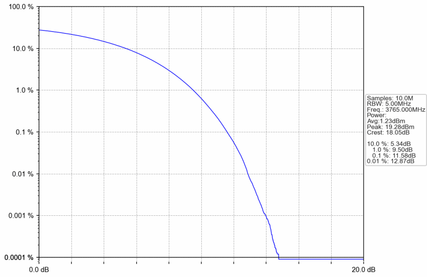
n78a_30kHz_SISO_NTNV_70MHz_CP-OFDM 256 QAM_3765MHz_Outer_Full
