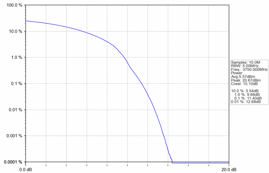
n78a_30kHz_SISO_NTNV_90MHz_DFT-s-OFDM QPSK_3750MHz_Outer_Full
