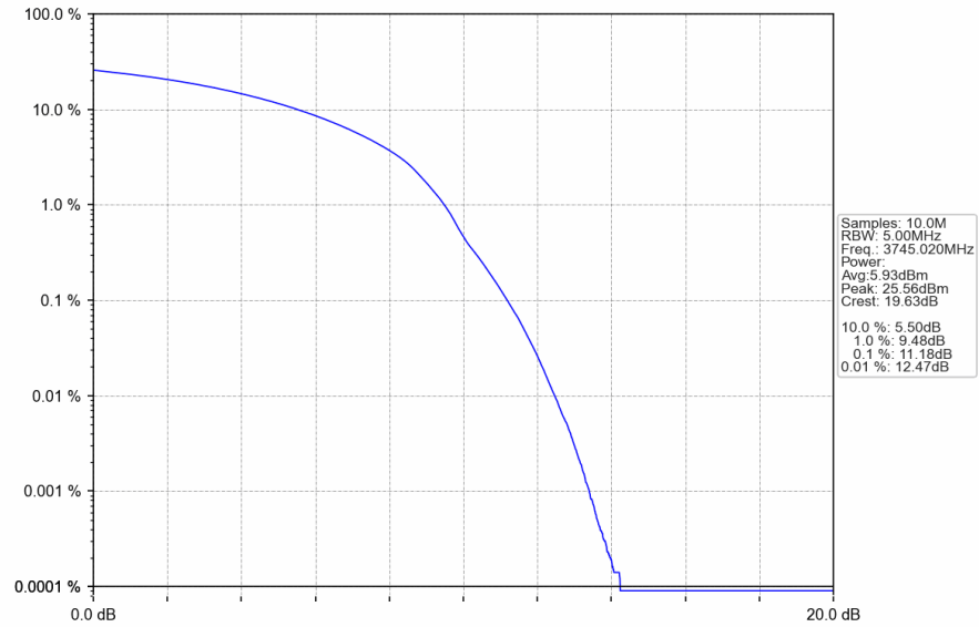
n78a_30kHz_SISO_NTNV_90MHz_DFT-s-OFDM QPSK_3745.02MHz_Outer_Full
