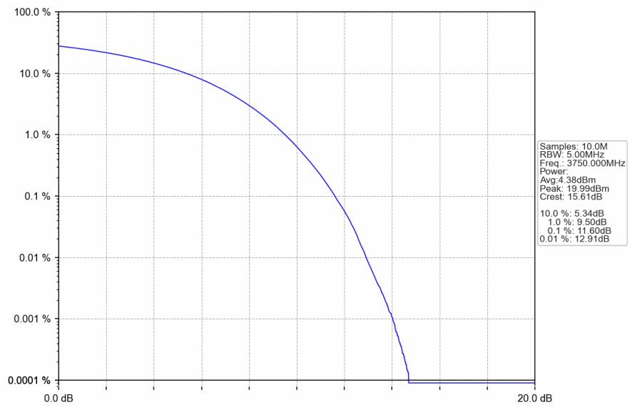
n78a_30kHz_SISO_NTNV_70MHz_CP-OFDM 64 QAM_3750MHz_Outer_Full
