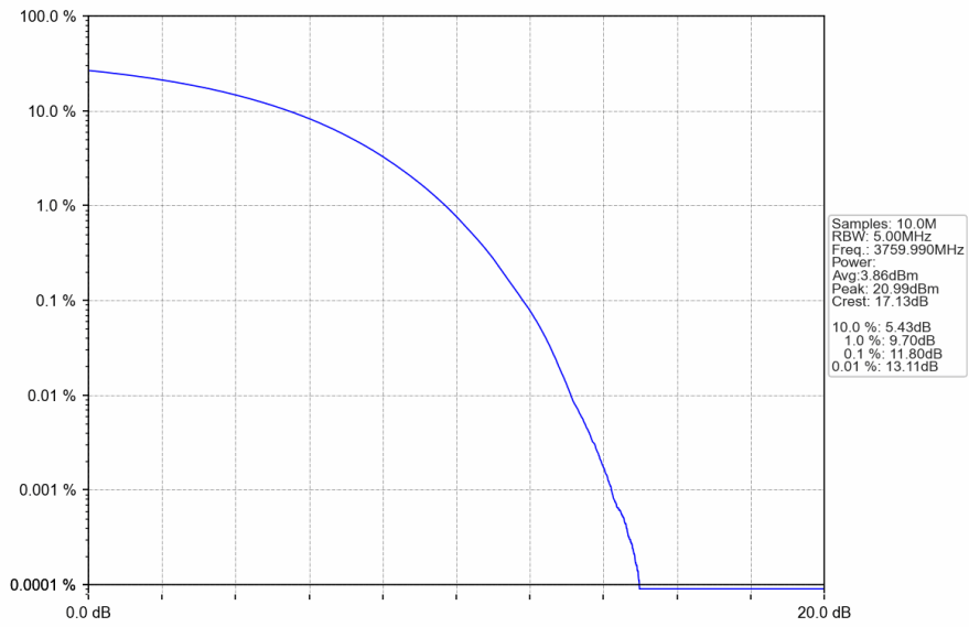
n78a_30kHz_SISO_NTNV_80MHz_CP-OFDM_QPSK_3759.99MHz_Outer_Full
