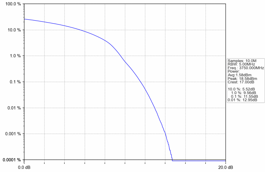
n78a_30kHz_SISO_NTNV_100MHz_DFT-s-OFDM_256_QAM_3750MHz_Outer_Full
