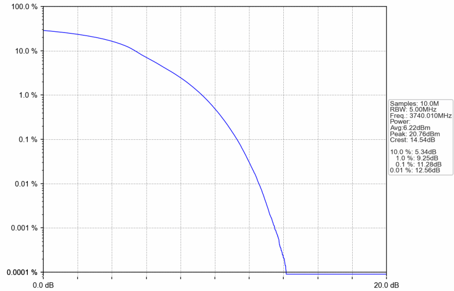
n78a_30kHz_SISO_NTNV_80MHz_DFT-s-OFDM QPSK_3740.01MHz_Outer_Full
