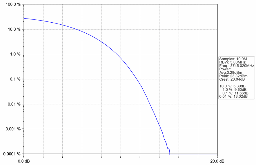
n78a_30kHz_SISO_NTNV_90MHz_CP-OFDM 64 QAM_3745.02MHz_Outer_Full
