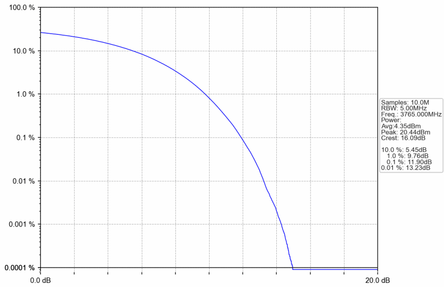
n78a_30kHz_SISO_NTNV_70MHz_CP-OFDM QPSK_3765MHz_Outer_Full
