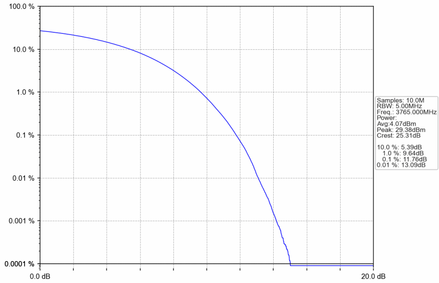
n78a_30kHz_SISO_NTNV_70MHz_CP-OFDM 64 QAM_3765MHz_Outer_Full
