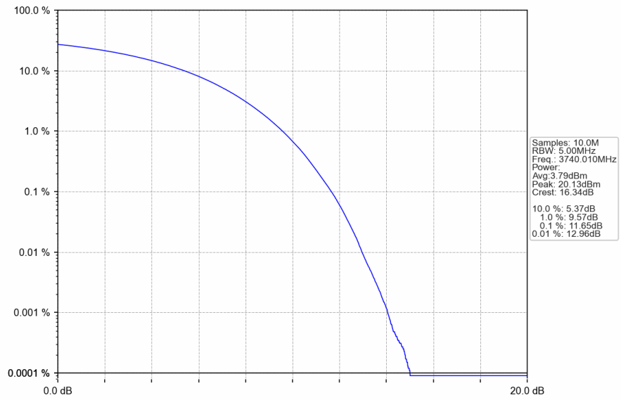
n78a_30kHz_SISO_NTNV_80MHz_CP-OFDM 64 QAM_3740.01MHz_Outer_Full
