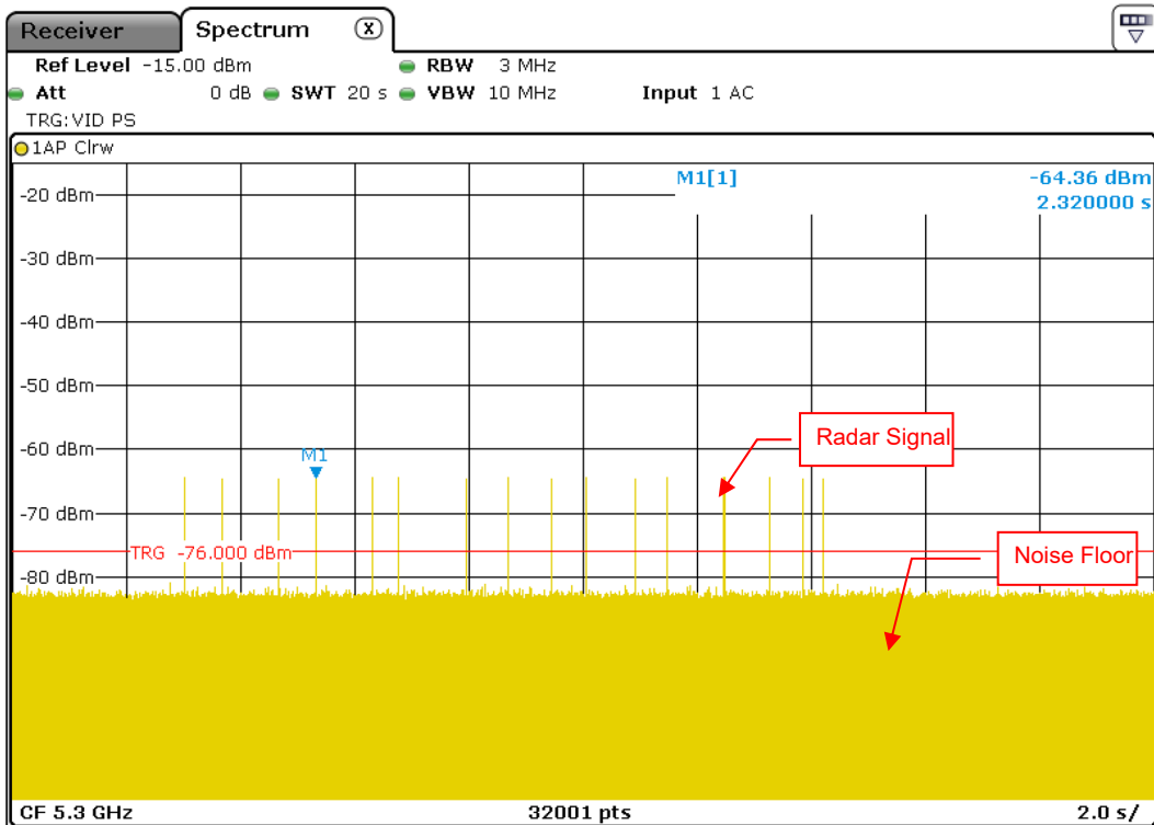
Radar Signal 5
