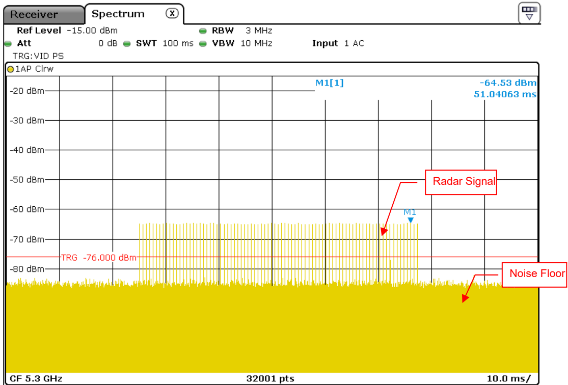
Radar Signal 1
