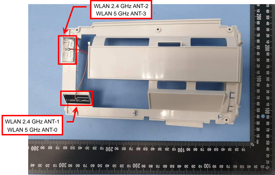
EUT Photo (28)
