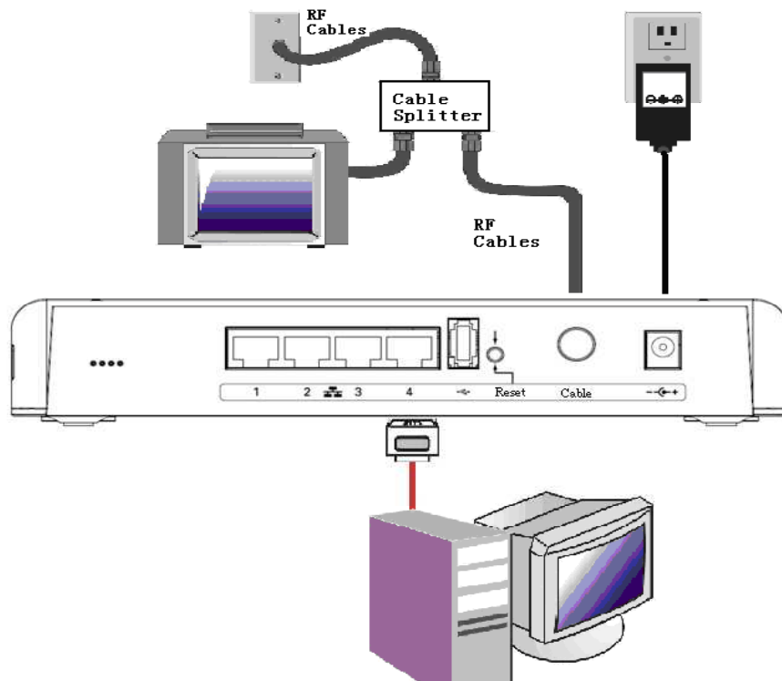
Fig.2: Ethernet Connection
