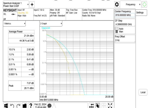
Band26-Part90s_5MHz_64QAM_RB25_0_CH26740
