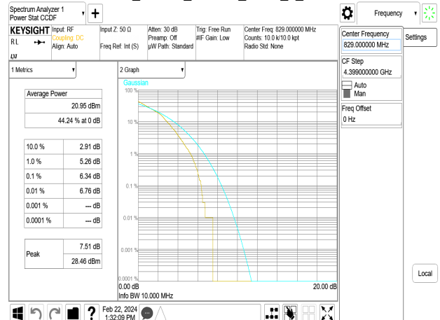
Band26_10MHz_64QAM_RB50_0_CH26840
