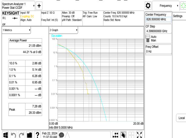
Band26_5MHz_64QAM_RB25_0_CH26815
