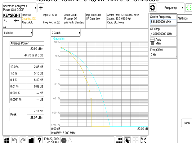
Band26_15MHz_64QAM_RB75_0_CH26865
