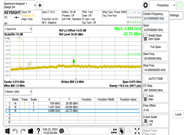
Band17_5MHz_QPSK_RB1_0_CH23790
