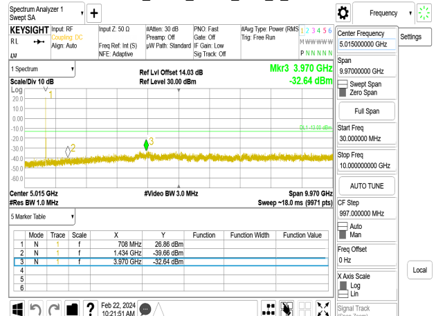
Band17_5MHz_QPSK_RB1_0_CH23790
