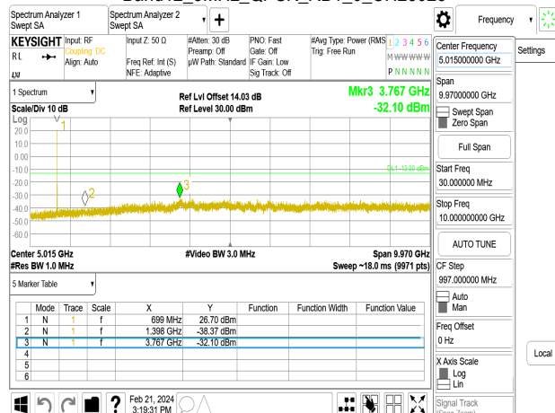
Band12_3MHz_QPSK_RB1_0_CH23095
