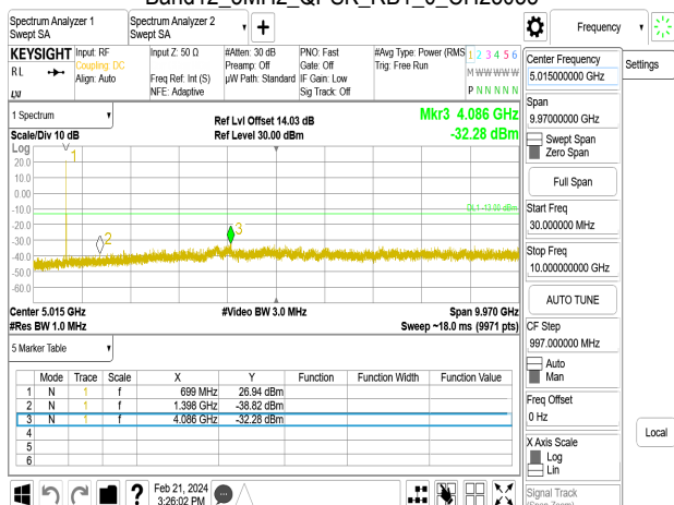
Band12_5MHz_QPSK_RB1_0_CH23095
