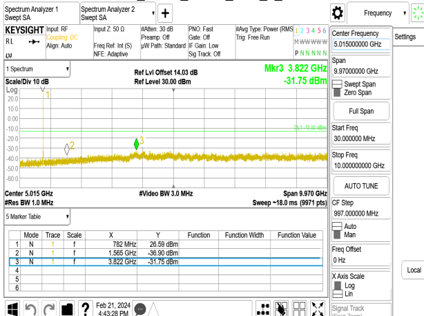
Band13_5MHz_QPSK_RB1_0_CH23255
