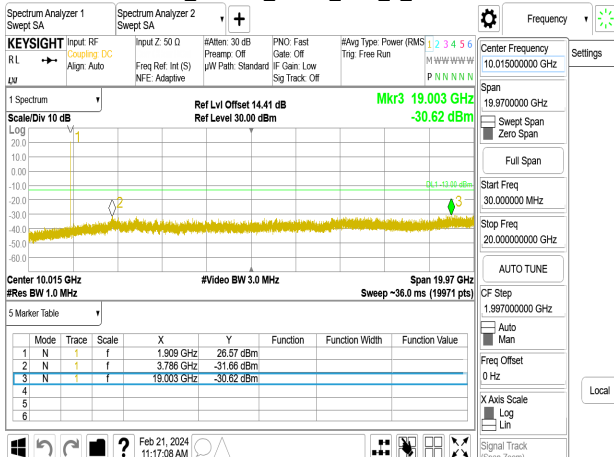
Band2_1.4MHz_QPSK_RB1_0_CH19193
