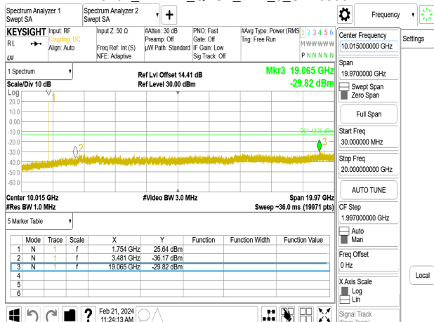
Band4_1.4MHz_QPSK_RB1_0_CH20393
