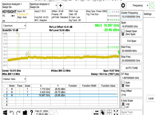
Band4_5MHz_QPSK_RB1_0_CH20175
