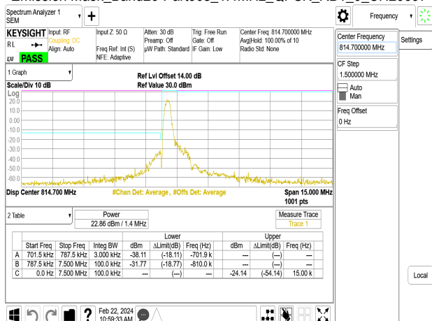
Emission Mask_Band26-Part90s_1.4MHz_QPSK_RB1_5_CH26783
