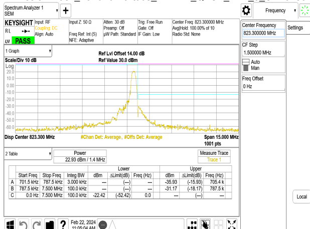
Emission Mask_Band26-Part90s_1.4MHz_QPSK_RB1_5_CH26783
