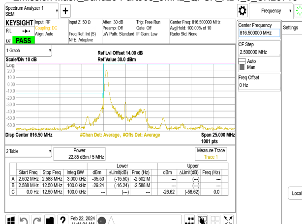
Emission Mask_Band26-Part90s_5MHz_QPSK_RB1_24_CH26765
