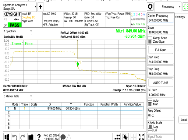
Band Edge_Band26_10MHz_QPSK_RB1_0_CH26840
