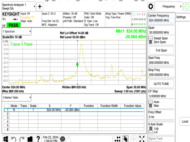
Band Edge_Band26_15MHz_QPSK_RB1_0_CH26865
