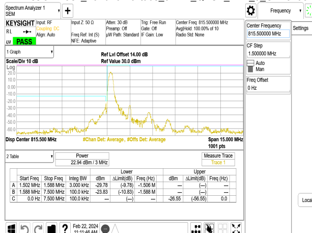
Emission Mask_Band26-Part90s_3MHz_QPSK_RB1_0_CH26705
