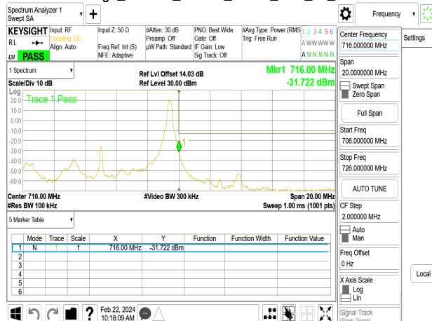
Band Edge_Band17_10MHz_QPSK_RB50_0_CH23780
