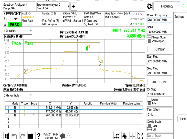
Band Edge_Band13_5MHz_QPSK_RB25_0_CH23255
