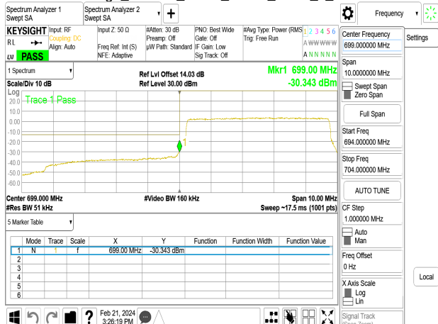
Band Edge_Band12_5MHz_QPSK_RB25_0_CH23035
