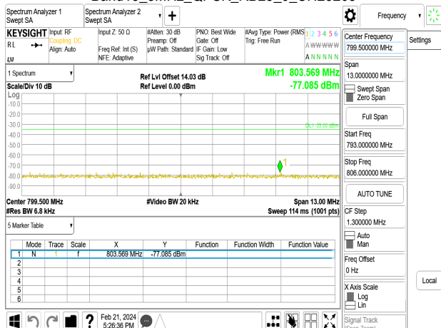
Band13_5MHz_QPSK_RB25_0_CH23255
