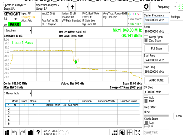
Band Edge_Band5_5MHz_QPSK_RB25_0_CH20625
