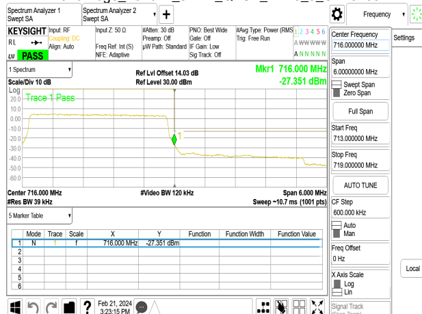
Band Edge_Band12_3MHz_QPSK_RB15_0_CH23165
