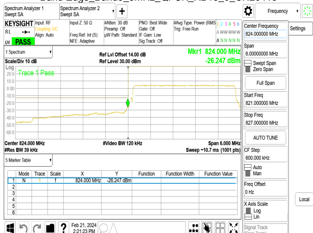
Band Edge_Band5_3MHz_QPSK_RB15_0_CH20635
