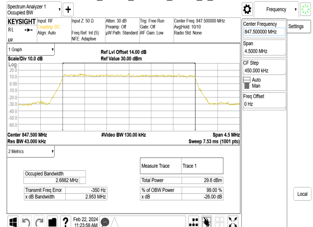
Band26_3MHz_64QAM_RB15_0_CH27025
