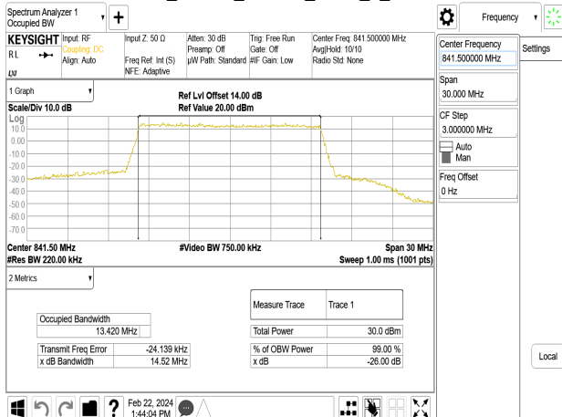
Band26_15MHz_64QAM_RB75_0_CH26965
