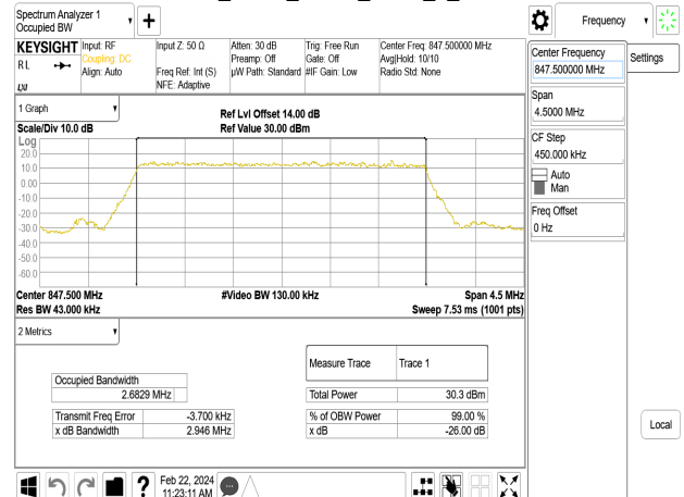
Band26_3MHz_QPSK_RB15_0_CH27025
