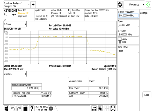
Band26_10MHz_64QAM_RB50_0_CH26990
