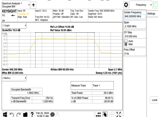
Band26_1.4MHz_64QAM_RB6_0_CH27033
