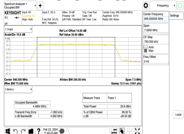
Band26_5MHz_16QAM_RB25_0_CH27015
