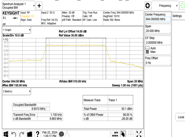
Band26_10MHz_16QAM_RB50_0_CH26990
