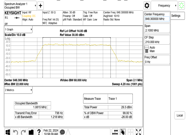
Band26_1.4MHz_16QAM_RB6_0_CH27033
