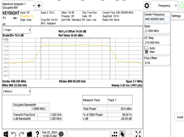
Band26_1.4MHz_QPSK_RB6_0_CH27033
