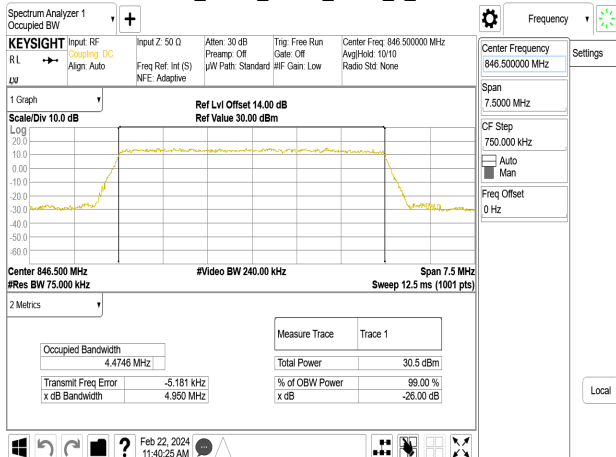
Band26_5MHz_QPSK_RB25_0_CH27015
