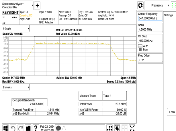
Band26_3MHz_16QAM_RB15_0_CH27025
