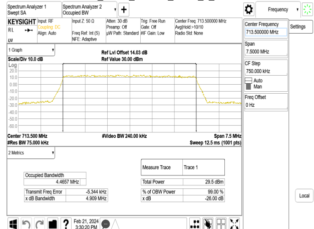
Band12_5MHz_16QAM_RB25_0_CH23155
