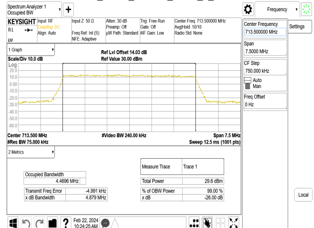
Band17_5MHz_16QAM_RB25_0_CH23825
