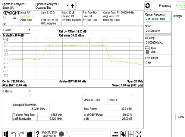
Band12_10MHz_16QAM_RB50_0_CH23130
