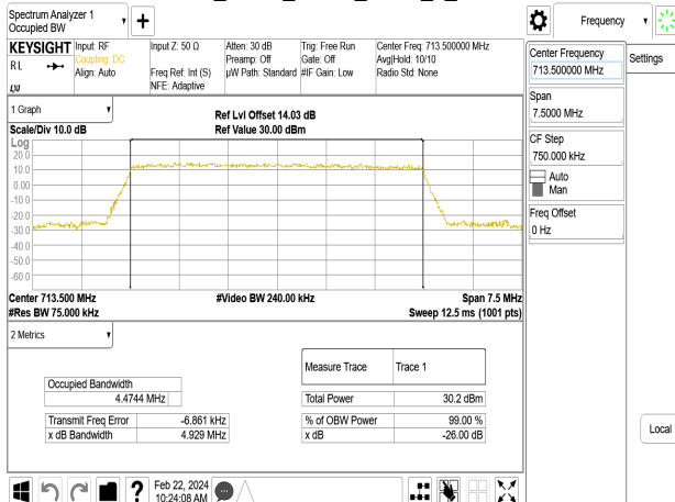
Band17_5MHz_QPSK_RB25_0_CH23825
