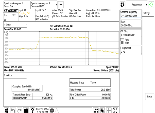
Band12_10MHz_64QAM_RB50_0_CH23130
