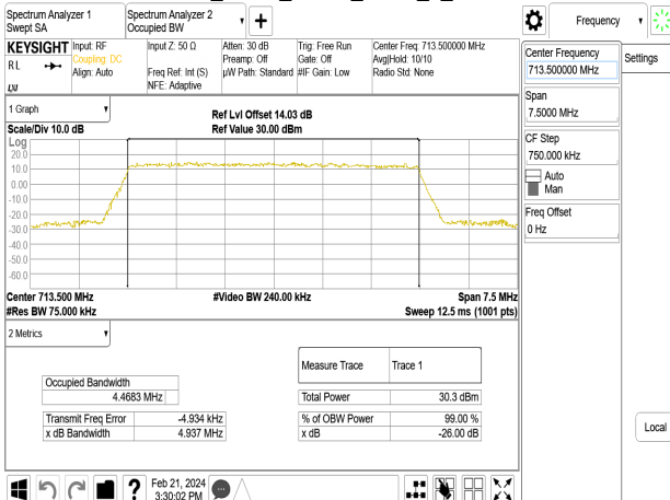
Band12_5MHz_QPSK_RB25_0_CH23155
