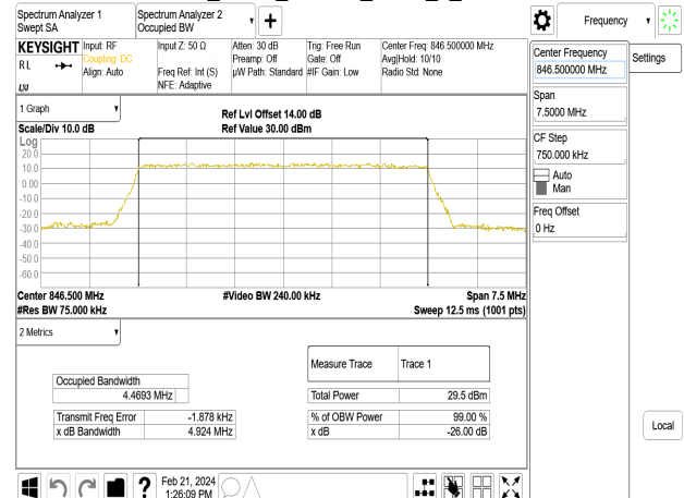
Band5_5MHz_16QAM_RB25_0_CH20625
