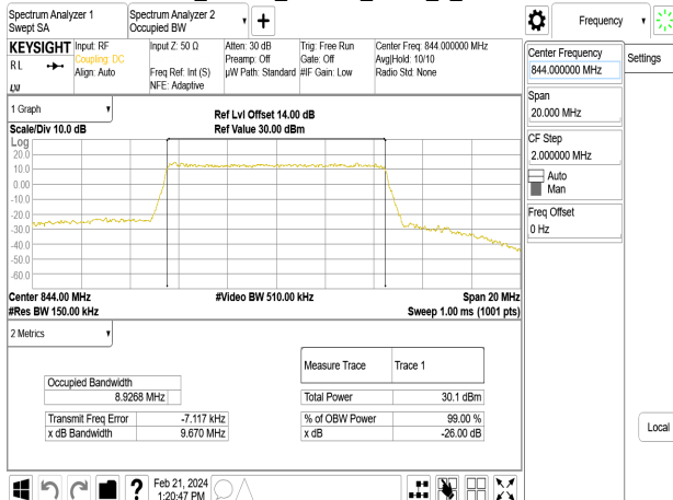
Band5_10MHz_16QAM_RB50_0_CH20600
