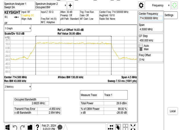
Band12_3MHz_QPSK_RB15_0_CH23165
