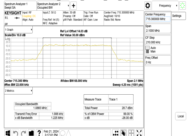
Band12_1.4MHz_16QAM_RB6_0_CH23173
