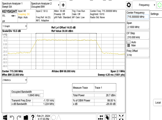
Band12_1.4MHz_64QAM_RB6_0_CH23173
