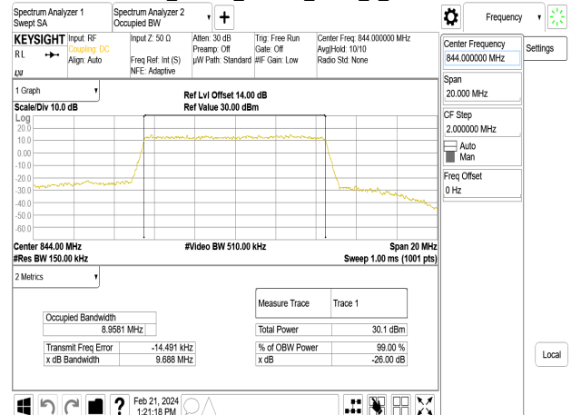
Band5_10MHz_64QAM_RB50_0_CH20600
