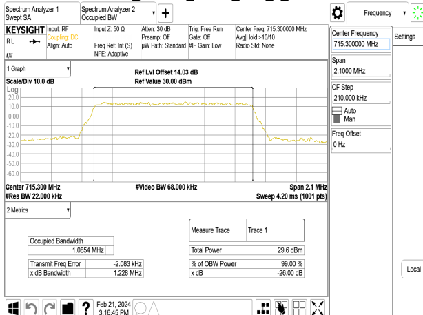
Band12_1.4MHz_QPSK_RB6_0_CH23173
