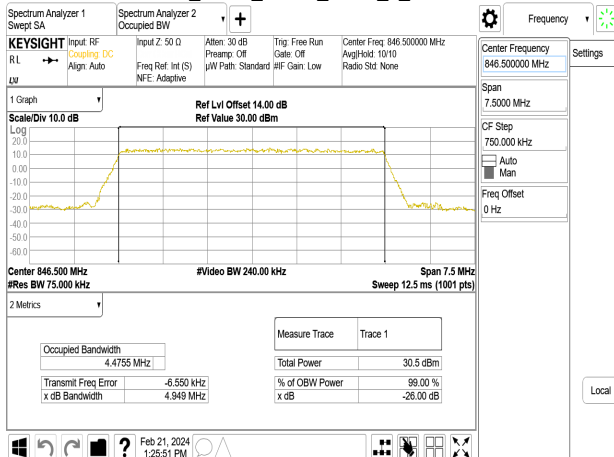
Band5_5MHz_QPSK_RB25_0_CH20625
