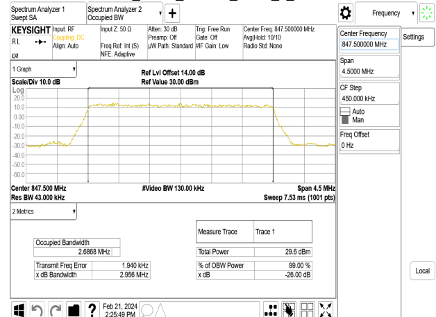
Band5_3MHz_64QAM_RB15_0_CH20635
