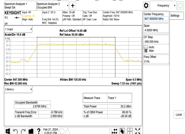
Band5_3MHz_QPSK_RB15_0_CH20635
