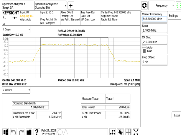
Band5_1.4MHz_64QAM_RB6_0_CH20643
