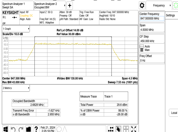
Band5_3MHz_16QAM_RB15_0_CH20635
