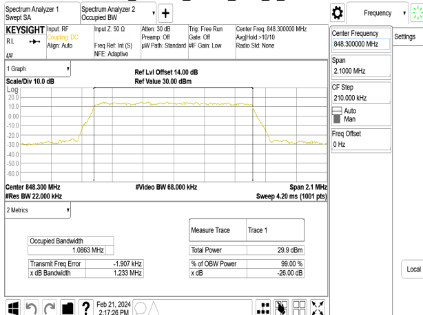
Band5_1.4MHz_QPSK_RB6_0_CH20643
