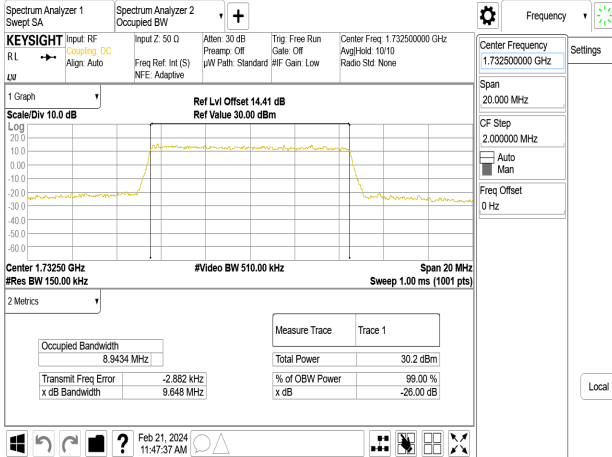
Band4_10MHz_16QAM_RB50_0_CH20350
