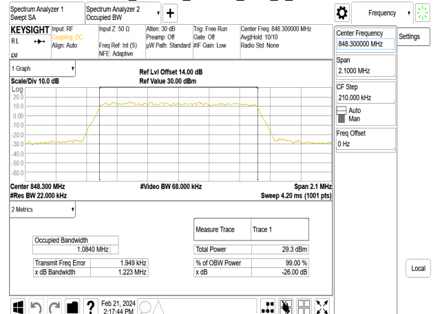
Band5_1.4MHz_16QAM_RB6_0_CH20643
