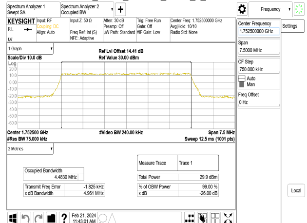
Band4_5MHz_16QAM_RB25_0_CH20375
