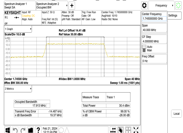
Band4_20MHz_64QAM_RB100_0_CH20300
