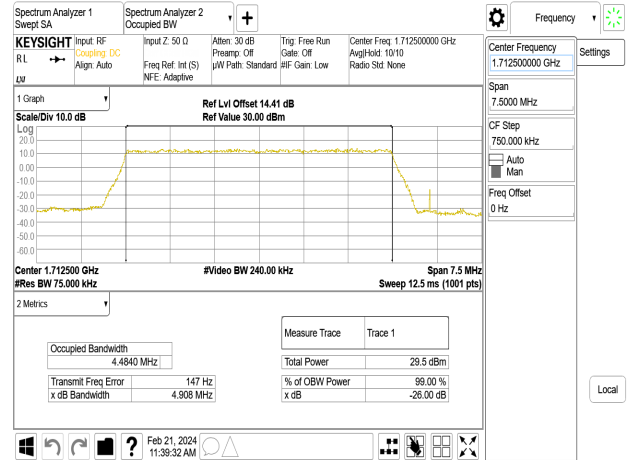
Band4_5MHz_16QAM_RB25_0_CH20175
