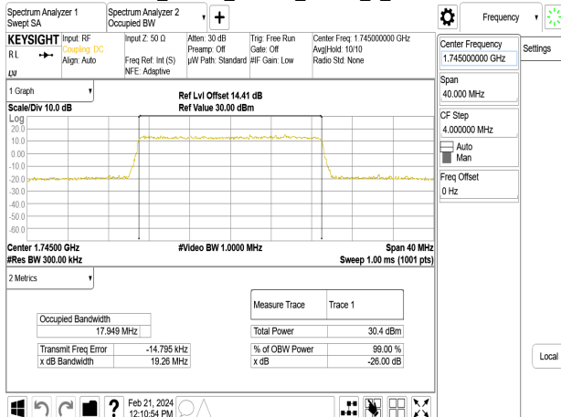
Band4_20MHz_16QAM_RB100_0_CH20300
