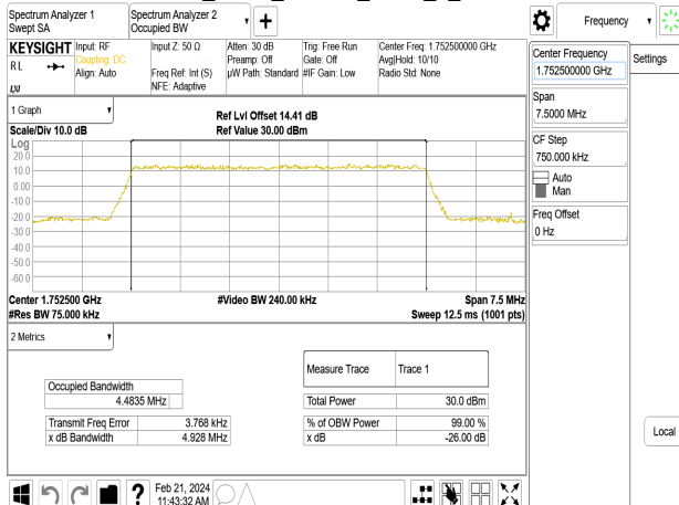
Band4_5MHz_64QAM_RB25_0_CH20375
