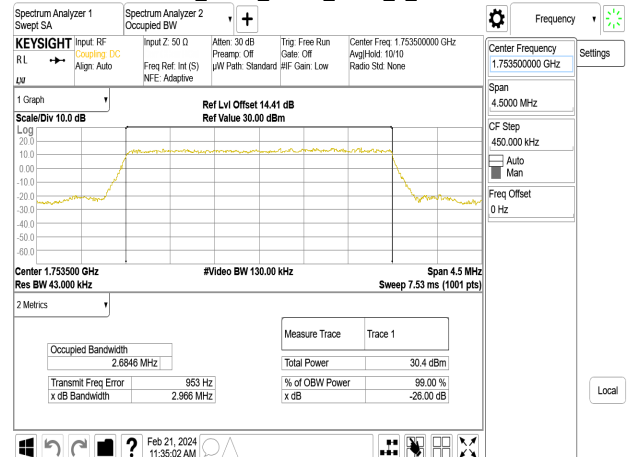
Band4_3MHz_QPSK_RB15_0_CH20385
