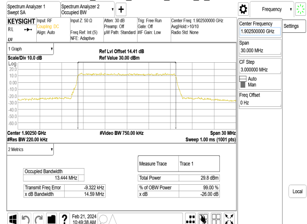
Band2_15MHz_16QAM_RB75_0_CH19125
