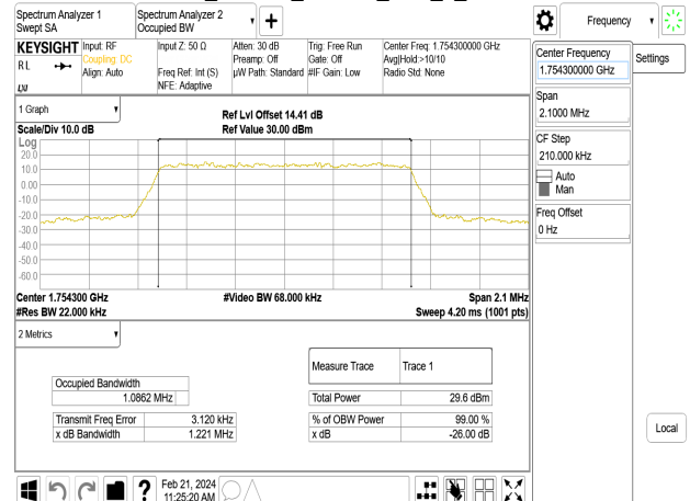
Band4_1.4MHz_16QAM_RB6_0_CH20393
