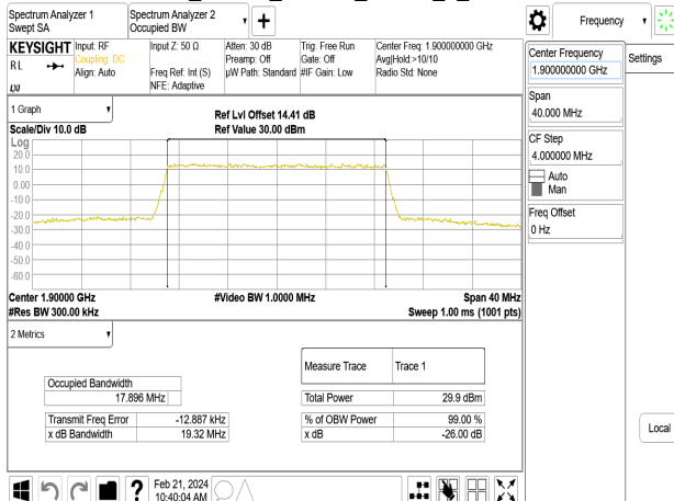
Band2_20MHz_16QAM_RB100_0_CH19100
