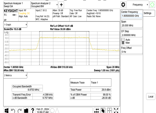
Band2_10MHz_64QAM_RB50_0_CH19150
