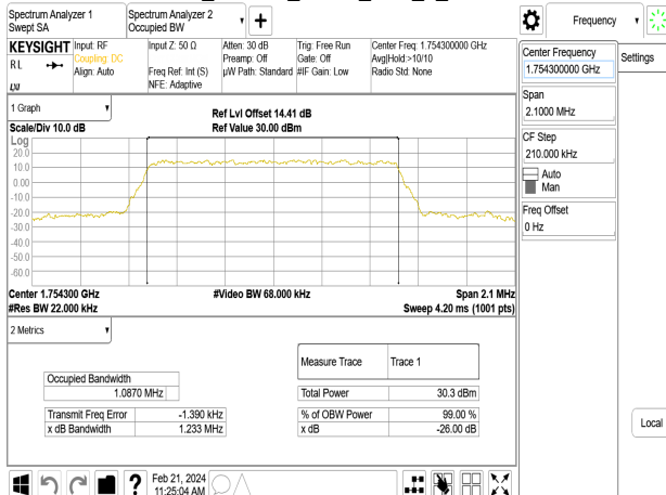
Band4_1.4MHz_QPSK_RB6_0_CH20393
