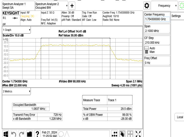
Band4_1.4MHz_64QAM_RB6_0_CH20393
