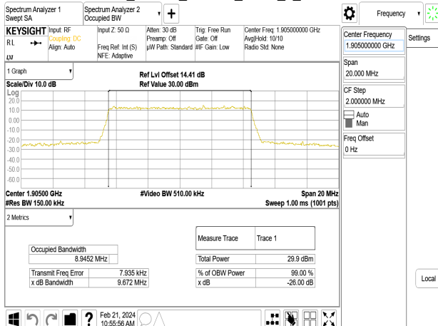
Band2_10MHz_16QAM_RB50_0_CH19150
