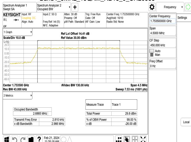
Band4_3MHz_16QAM_RB15_0_CH20385
