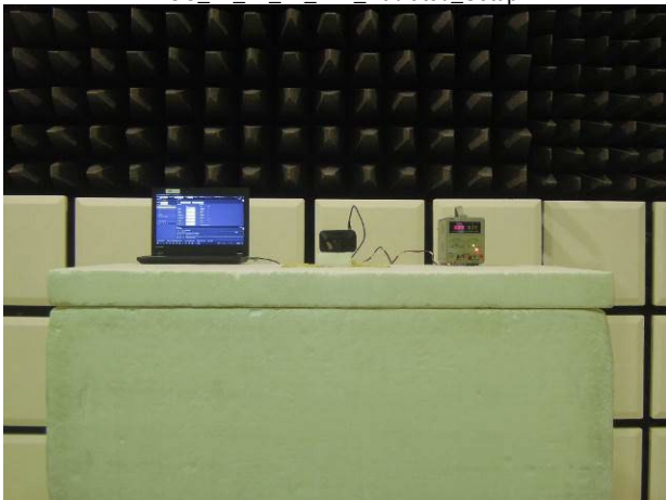
FCC_22_24_27_LTE_Radiated_Setup
