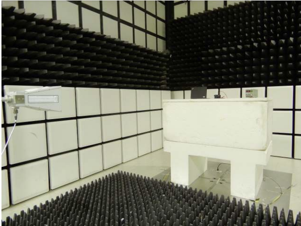
Co-location_Setup
