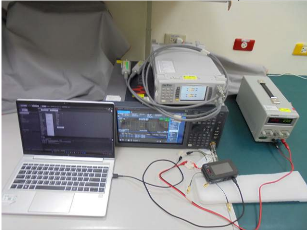
FCC_22_24_27_LTE_Conducted_setup1
