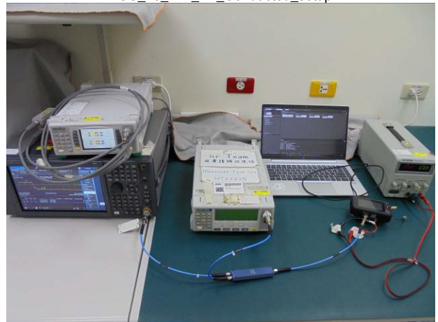
FCC_15_247_BT_Conducted_setup
