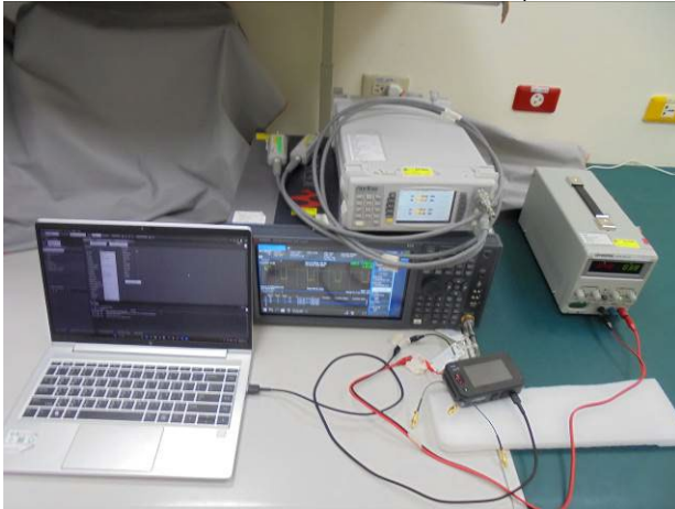
FCC 15 407 WLAN Conducted_setup
