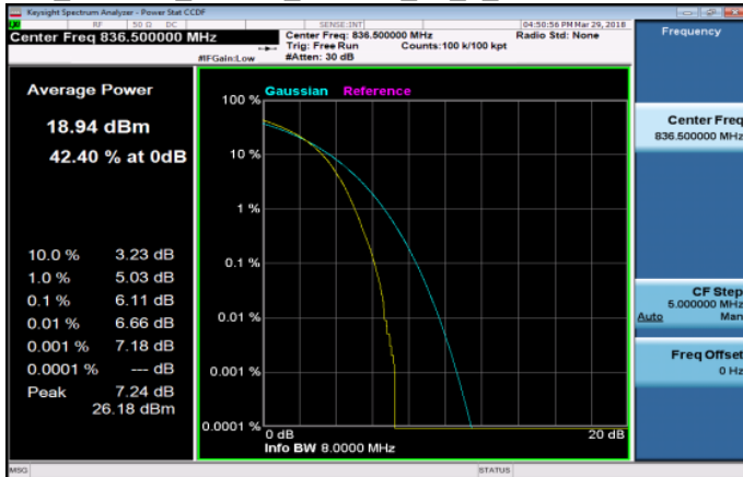
LTE_Band26_15MHz_16QAM_75_0_MidCH26915-836.5
