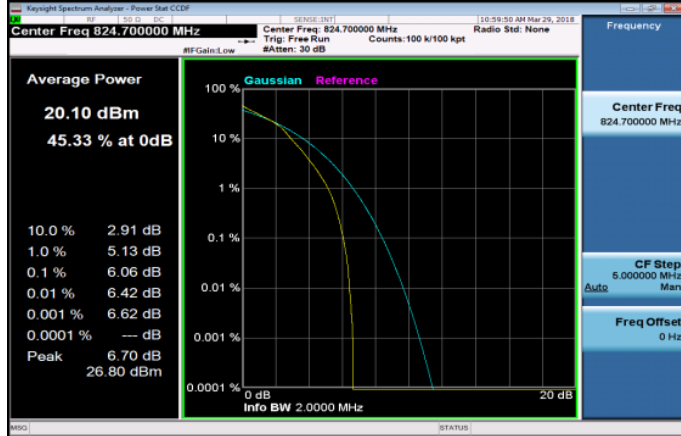
LTE_Band5_1_4MHz_16QAM_6_0_LowCH20407-824.7
