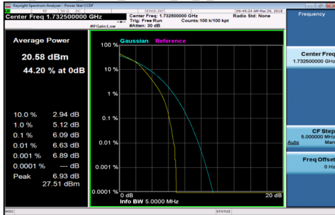
LTE_Band4_5MHz_16QAM_25_0_MidCH20175-1732.5
