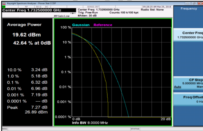
LTE_Band4_15MHz_16QAM_75_0_MidCH20175-1732.5
