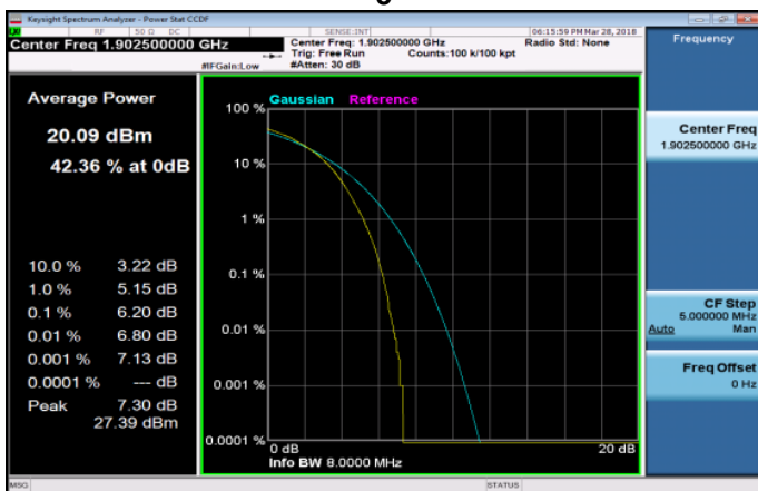
LTE_Band2_15MHz_16QAM_75_0_HighCH19125-1902.
