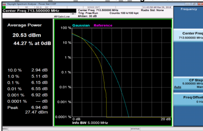
LTE_Band17_5MHz_16QAM_25_0_HighCH23825-713.5
