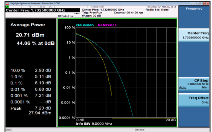
LTE_Band4_10MHz_16QAM_50_0_MidCH20175-1732.5
