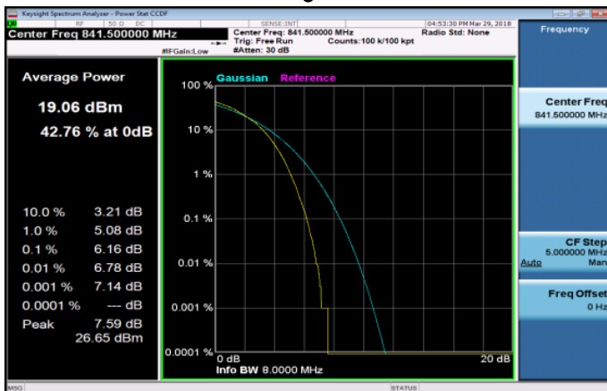
LTE_Band26_15MHz_16QAM_75_0_HighCH26965-841.
