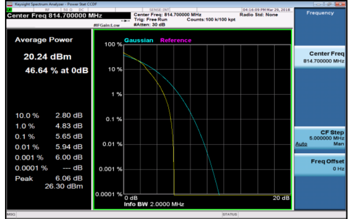
90_LTE_Band26_1_4MHz_16QAM_6_0_LowCH26697-814.7
