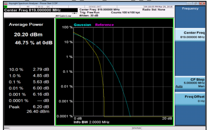
Part 90_LTE_Band26_1_4MHz_16QAM_6_0_MidCH26740-819
