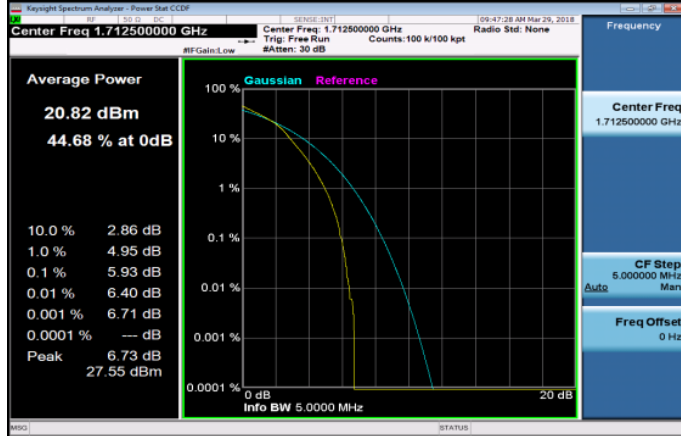
LTE_Band4_5MHz_16QAM_25_0_LowCH1975-1712.5
