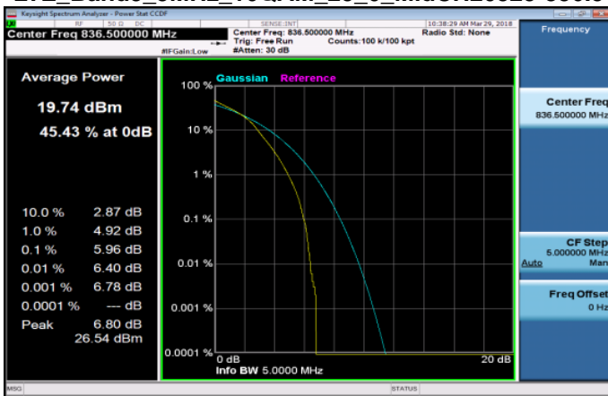
LTE_Band5_5MHz_16QAM_25_0_MidCH20525-836.5
