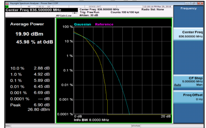
LTE_Band26 10MHz_16QAM_50_0_MidCH26915-836.5
