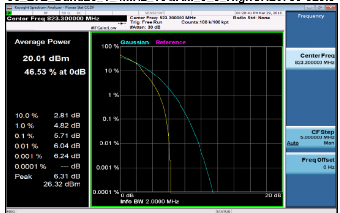
90_LTE_Band26_1_4MHz_16QAM_6_0_HighCH26783-823.3
