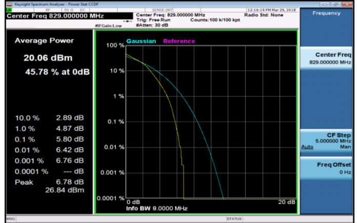
LTE_Band26 10MHz_16QAM_50_0_LowCH26840-829
