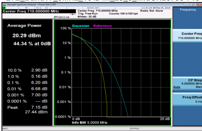
LTE_Band17_5MHz_16QAM_25_0_MidCH23790-710
