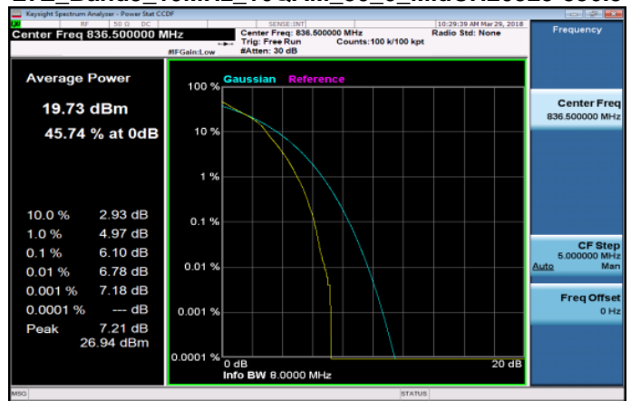
LTE_Band5_10MHz_16QAM_50_0_MidCH20525-836.5
