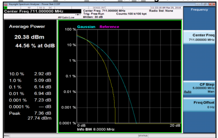
LTE_Band17_10MHz_16QAM_50_0_HighCH23800-711
