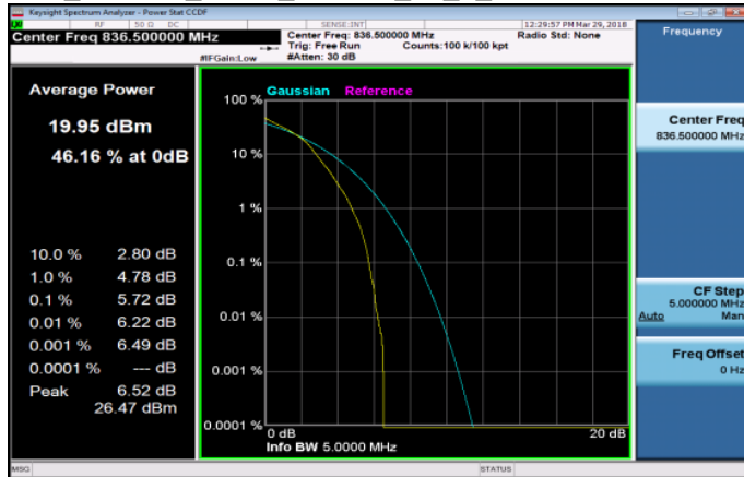
LTE_Band26 5MHz_16QAM_25_0_MidCH26915-836.5
