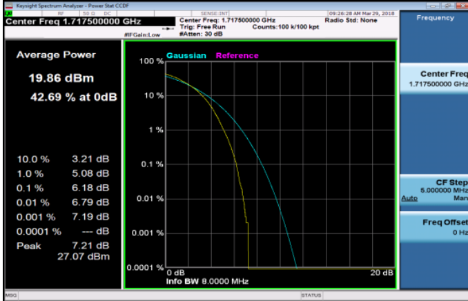
LTE_Band4_15MHz_16QAM_75_0_LowCH20025-1717.5
