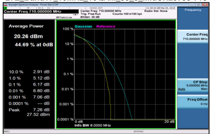
LTE_Band17_10MHz_16QAM_50_0_MidCH23790-710
