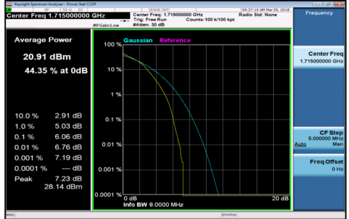
LTE_Band4_10MHz_16QAM_50_0_LowCH20000-1715
