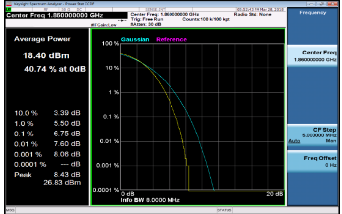
LTE_Band2_20MHz_16QAM_100_0_LowCH18700-1860
