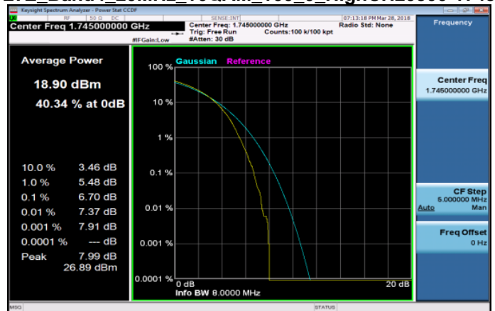
LTE_Band4_20MHz_16QAM_100_0_HighCH20300-1745
