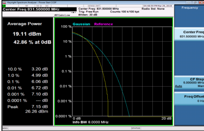
LTE_Band26_15MHz_16QAM_75_0_LowCH26865-831.5
