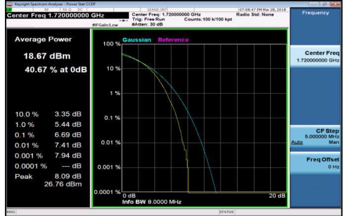
LTE_Band4_20MHz_16QAM_100_0_LowCH20050-1720
