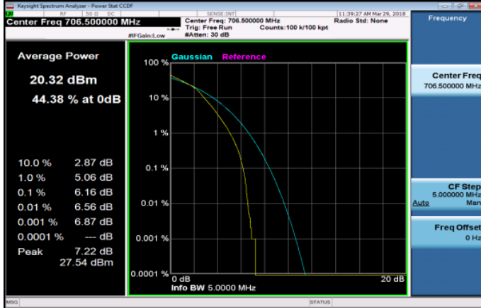
LTE_Band17_5MHz_16QAM_25_0_LowCH23755-706.5
