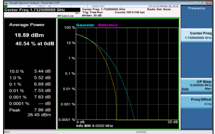
LTE_Band4_20MHz_16QAM_100_0_MidCH20175-1732.5
