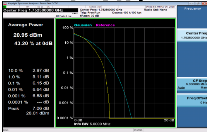
LTE_Band4_5MHz_16QAM_25_0_HighCH20375-1752.5
