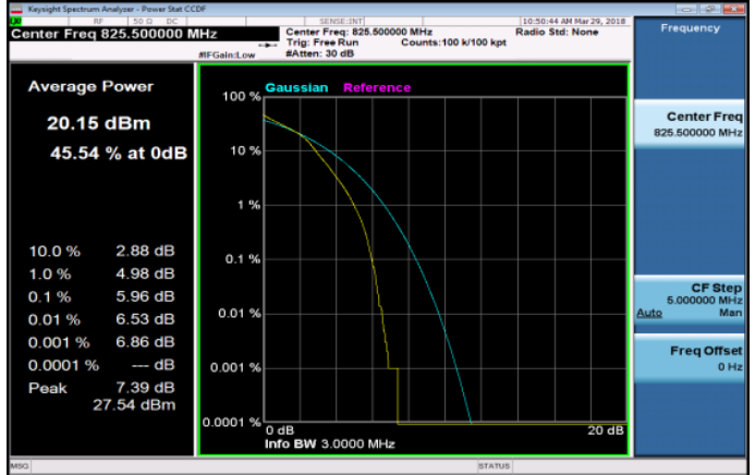
LTE_Band5_3MHz_16QAM_15_0_LowCH20415-825.5
