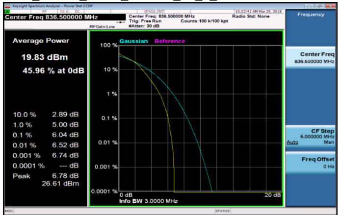
LTE_Band5_3MHz_16QAM_15_0_MidCH20525-836.5
