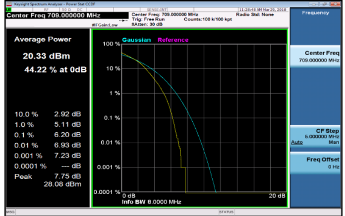
LTE_Band17_10MHz_16QAM_50_0_LowCH23780-709
