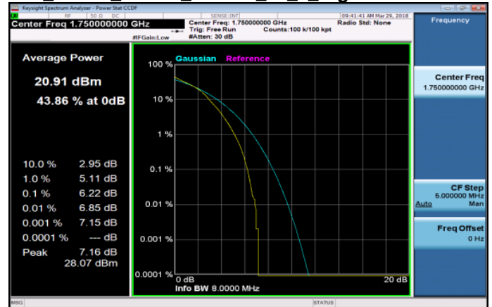
LTE_Band4_10MHz_16QAM_50_0_HighCH20350-1750
