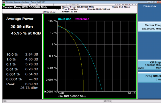
LTE_Band26 5MHz_16QAM_25_0_LowCH26815-826.5
