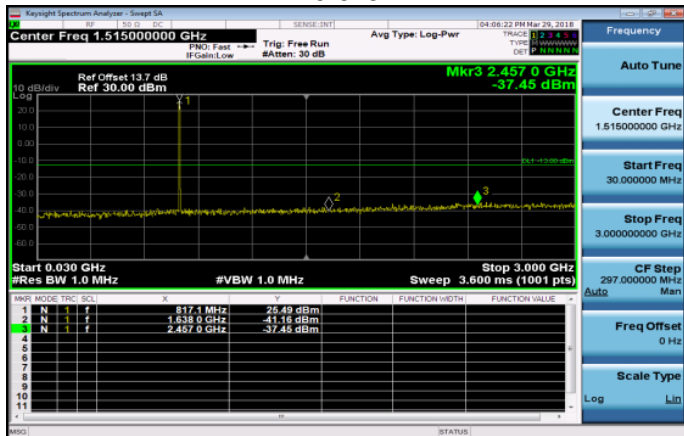
30MHz~3GHz_Band26_3MHz_QPSK_1_0_MidCH2674 0-819
