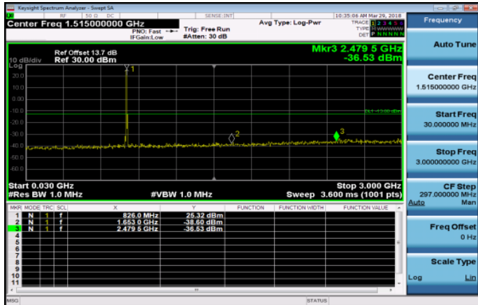
30MHz~3GHz_Band5_5MHz_QPSK_1_0_LowCH20425 -826.5
