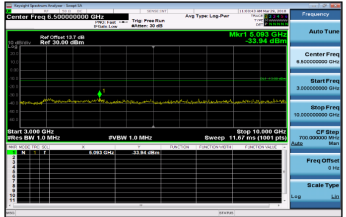
3GHz~10GHz_Band5_1_4MHz_QPSK_1_0_MidCH205 25-836.5
