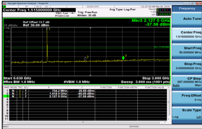
30MHz~3GHz_Band17_10MHz_QPSK_1_0_LowCH237 80-709
