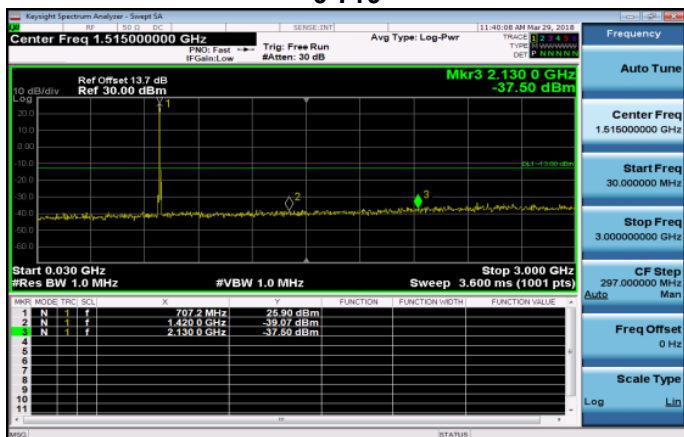
30MHz~3GHz_Band17_5MHz_QPSK_1_0_MidCH2379 0-710
