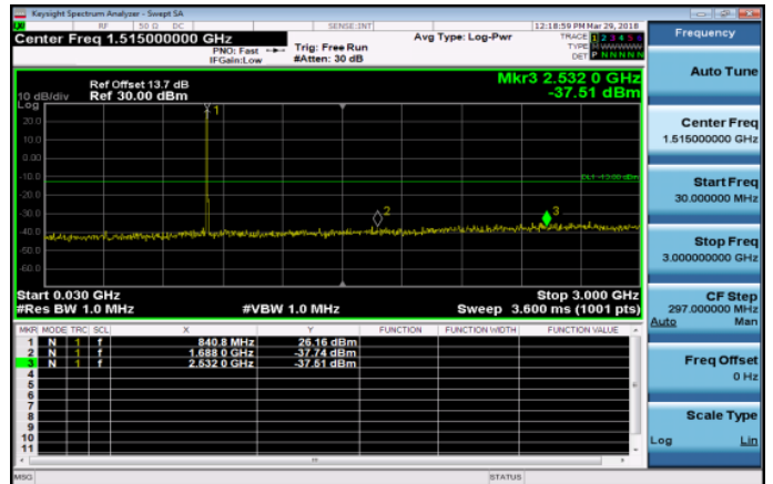
30MHz~3GHz_Band26_10MHz_QPSK_1_0_HighCH26 990-844
