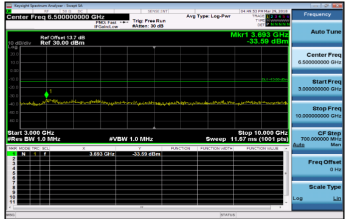
3GHz~10GHz_Band26_15MHz_QPSK_1_0_MidCH269 15-836.5
