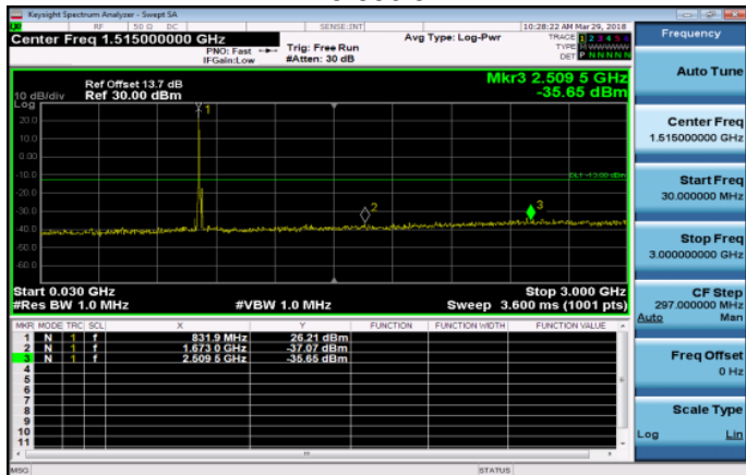
30MHz~3GHz_Band5_10MHz_QPSK_1_0_MidCH2052 5-836.5
