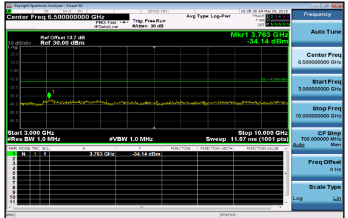
3GHz~10GHz_Band5_10MHz_QPSK_1_0_MidCH2052 5-836.5
