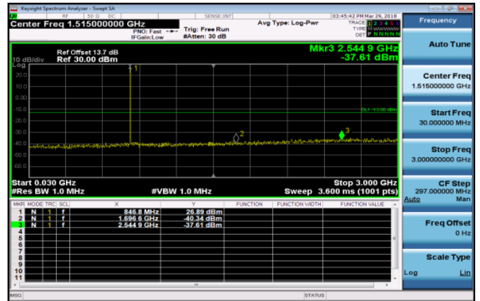
30MHz~3GHz_Band26_1_4MHz_QPSK_1_0_HighCH2 7033-848.3
