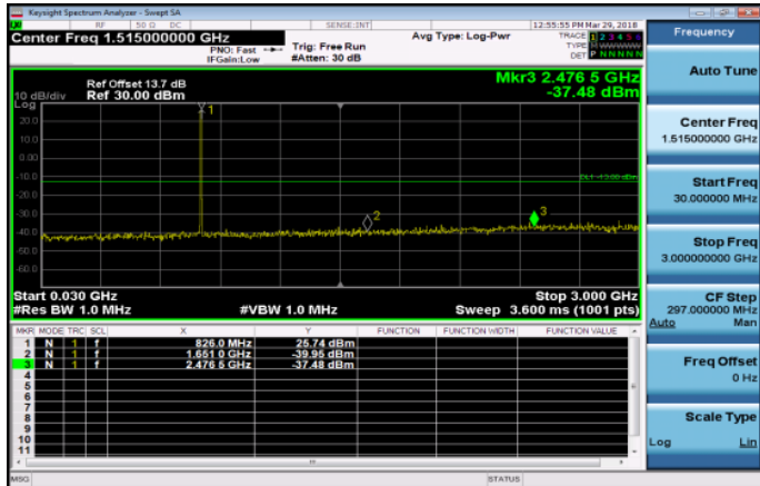
30MHz~3GHz_Band26_3MHz_QPSK_1_0_LowCH2680 5-825.5
