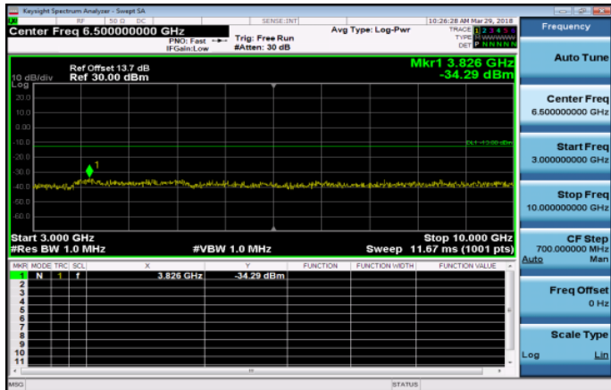
3GHz~10GHz_Band5_10MHz_QPSK_1_0_LowCH2045 0-829
