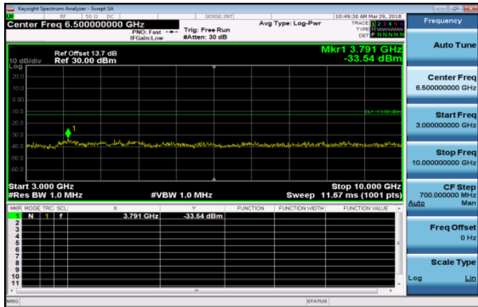
3GHz~10GHz_Band5_3MHz_QPSK_1_0_LowCH20415 -825.5
