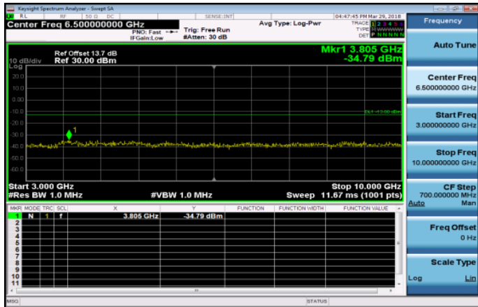
3GHz~10GHz_Band26_15MHz_QPSK_1_0_LowCH268 65-831.5
