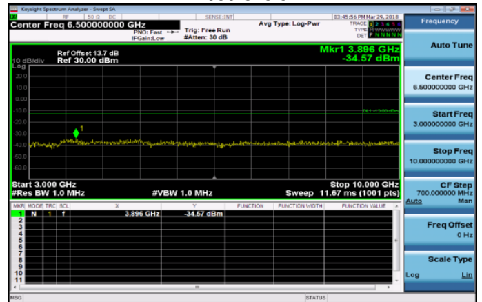
3GHz~10GHz_Band26_1_4MHz_QPSK_1_0_HighCH2 7033-848.3
