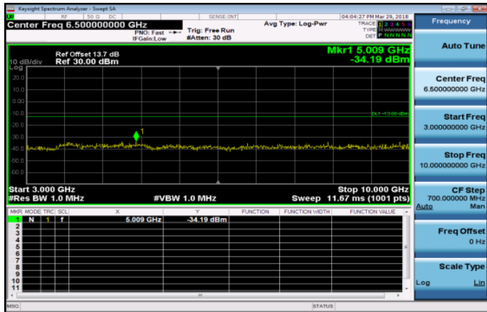
3GHz~10GHz_Band26_3MHz_QPSK_1_0_LowCH2670 5-815.5
