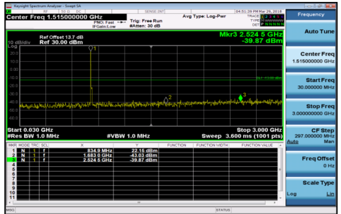
30MHz~3GHz_Band26_15MHz_QPSK_1_0_HighCH26 965-841.5
