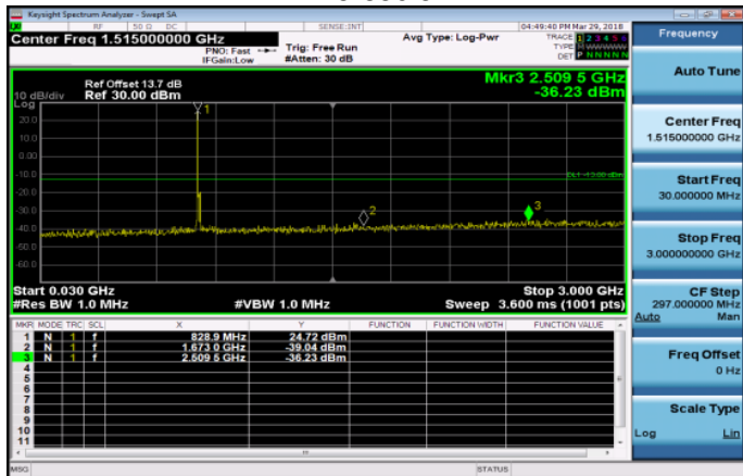
30MHz~3GHz_Band26_15MHz_QPSK_1_0_MidCH269 15-836.5
