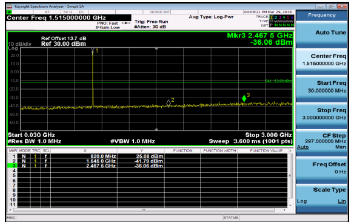
30MHz~3GHz_Band26_3MHz_QPSK_1_0_HighCH267 75-822.5
