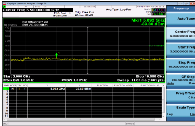
3GHz~10GHz_Band26_1_4MHz_QPSK_1_0_LowCH26 797-824.7
