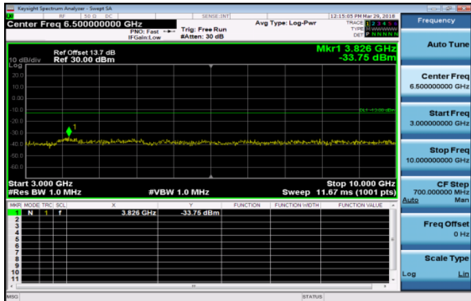
3GHz~10GHz_Band26_10MHz_QPSK_1_0_LowCH268 40-829
