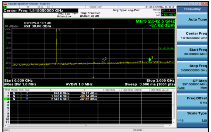
30MHz~3GHz_Band26_3MHz_QPSK_1_0_HighCH270 25-847.5
