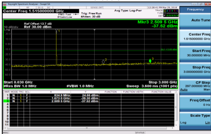
30MHz~3GHz_Band26_5MHz_QPSK_1_0_MidCH2691 5-836.5
