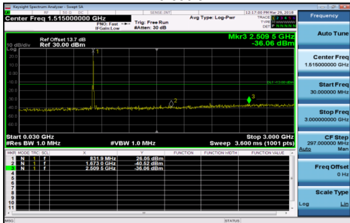
30MHz~3GHz_Band26_10MHz_QPSK_1_0_MidCH269 15-836.5
