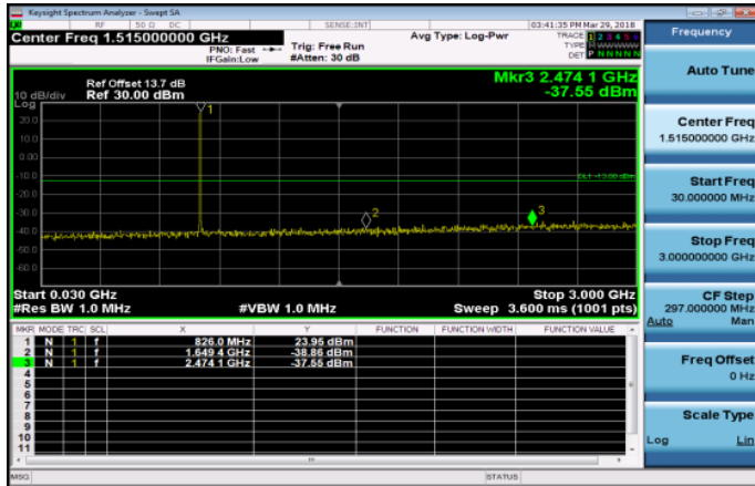
30MHz~3GHz_Band26_1_4MHz_QPSK_1_0_LowCH26 797-824.7
