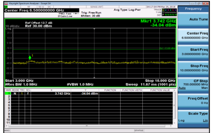
3GHz~10GHz_Band26_1_4MHz_QPSK_1_0_MidCH26 740-819
