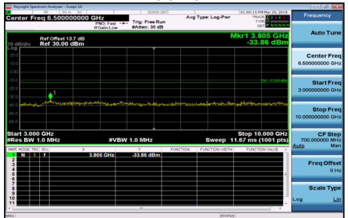
3GHz~10GHz_Band26_3MHz_QPSK_1_0_HighCH270 25-847.5
