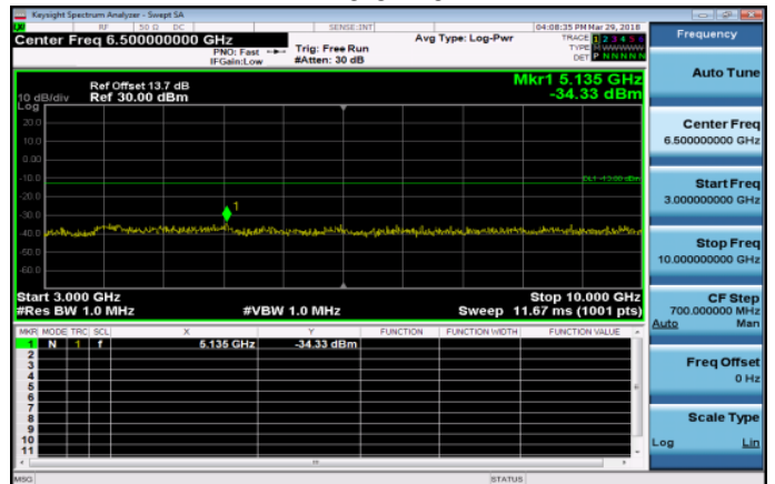
3GHz~10GHz_Band26_3MHz_QPSK_1_0_HighCH267 75-822.5
