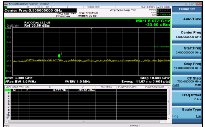
3GHz~10GHz_Band26_1_4MHz_QPSK_1_0_HighCH26 6783-823.3
