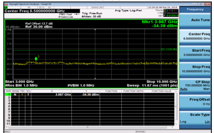
3GHz~10GHz_Band5_5MHz_QPSK_1_0_HighCH2062 5-846.5
