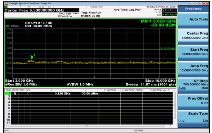
3GHz~10GHz_Band5_3MHz_QPSK_1_0_MidCH20525-836.5
