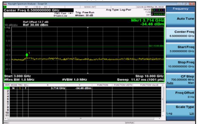
3GHz~10GHz_Band26_10MHz_QPSK_1_0_HighCH26 990-844
