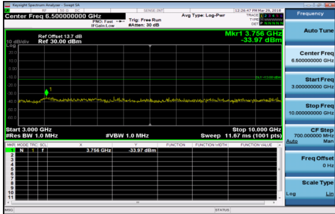
3GHz~10GHz_Band26_5MHz_QPSK_1_0_LowCH2681 5-826.5
