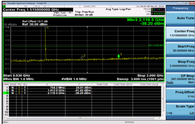
30MHz~3GHz_Band17_5MHz_QPSK_1_0_LowCH2375 5-706.5
