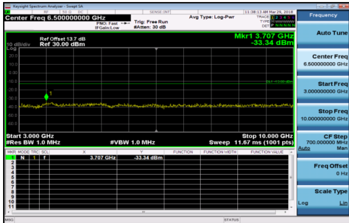
3GHz~10GHz_Band17_5MHz_QPSK_1_0_LowCH2375 5-706.5
