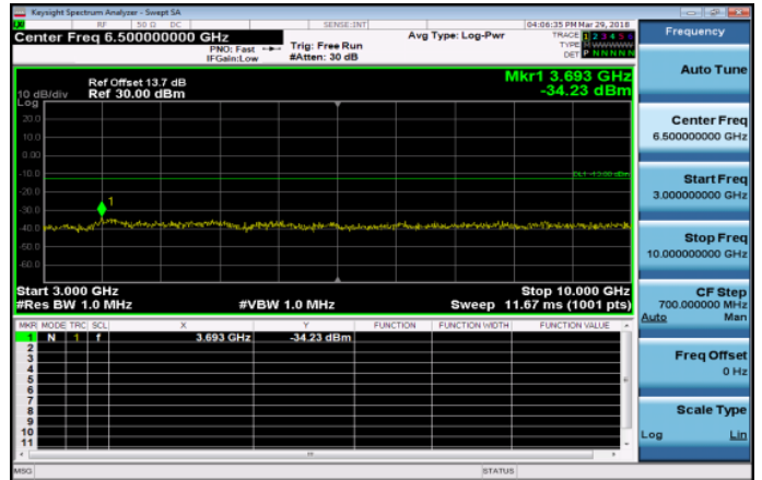
3GHz~10GHz_Band26_3MHz_QPSK_1_0_MidCH2674 0-819
