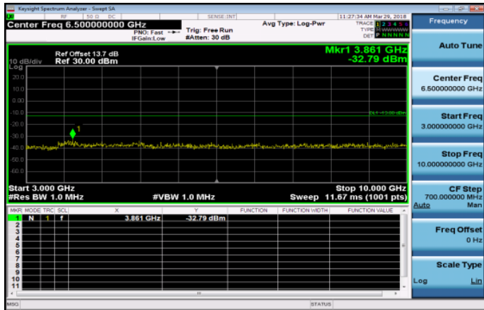
3GHz~10GHz_Band17_10MHz_QPSK_1_0_LowCH237 80-709
