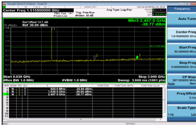
30MHz~3GHz_Band26_1_4MHz_QPSK_1_0_MidCH26 740-819
