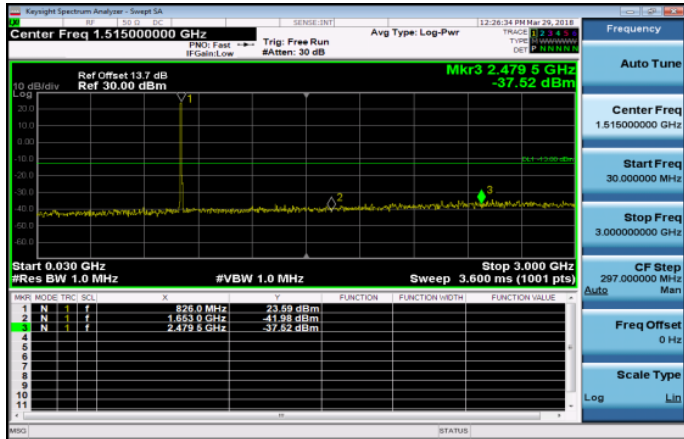
30MHz~3GHz_Band26_5MHz_QPSK_1_0_LowCH2681 5-826.5
