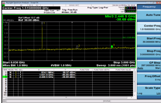
30MHz~3GHz_Band26_3MHz_QPSK_1_0_LowCH2670 5-815.5
