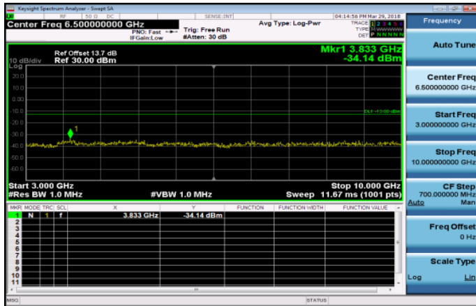
3GHz~10GHz_Band26_1_4MHz_QPSK_1_0_LowCH26 697-814.7
