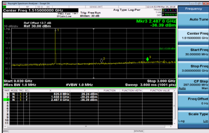
30MHz~3GHz_Band26_10MHz_QPSK_1_0_LowCH268 40-829
