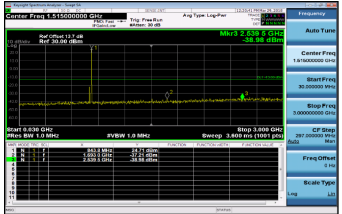
30MHz~3GHz_Band26_5MHz_QPSK_1_0_HighCH270 15-846.5
