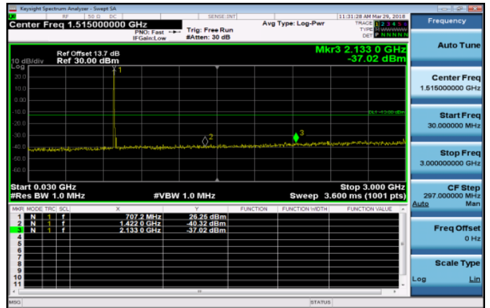
30MHz~3GHz_Band17_10MHz_QPSK_1_0_HighCH23 800-711
