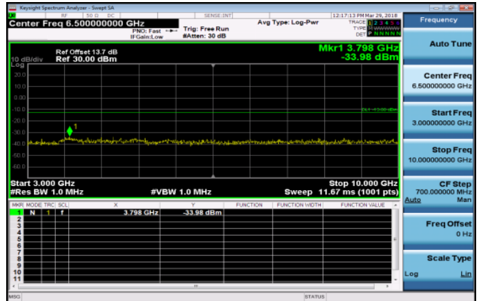
3GHz~10GHz_Band26_10MHz_QPSK_1_0_MidCH269 15-836.5
