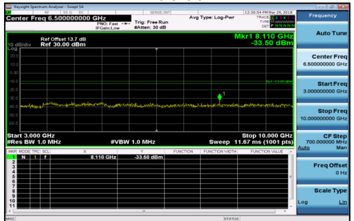
3GHz~10GHz_Band26_5MHz_QPSK_1_0_HighCH270 15-846.5
