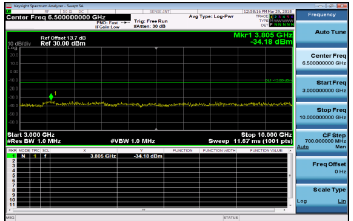
3GHz~10GHz_Band26_3MHz_QPSK_1_0_MidCH2691 5-836.5
