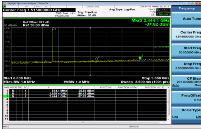
30MHz~3GHz_Band26_1_4MHz_QPSK_1_0_LowCH26 697-814.7
