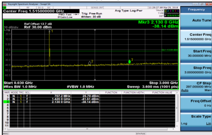
30MHz~3GHz_Band17_10MHz_QPSK_1_0_MidCH237 90-710
