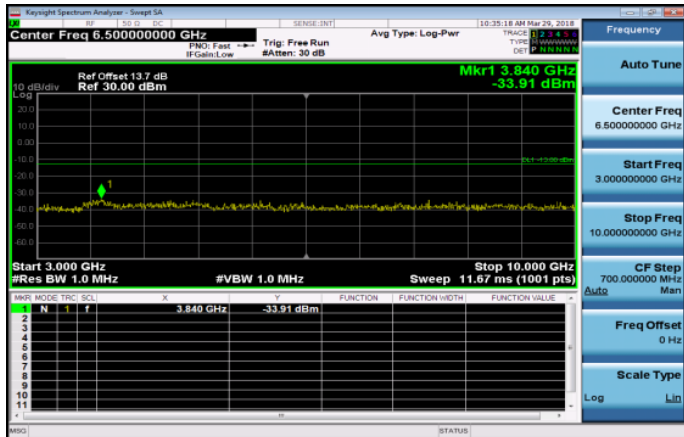
3GHz~10GHz_Band5_5MHz_QPSK_1_0_LowCH20425 -826.5
