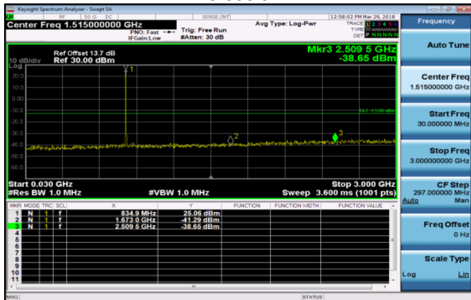
30MHz~3GHz_Band26_3MHz_QPSK_1_0_MidCH2691 5-836.5
