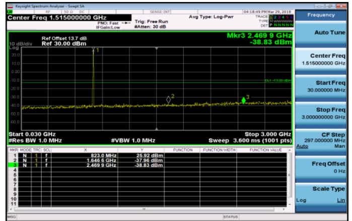
30MHz~3GHz_Band26_1_4MHz_QPSK_1_0_HighCH26 6783-823.3
