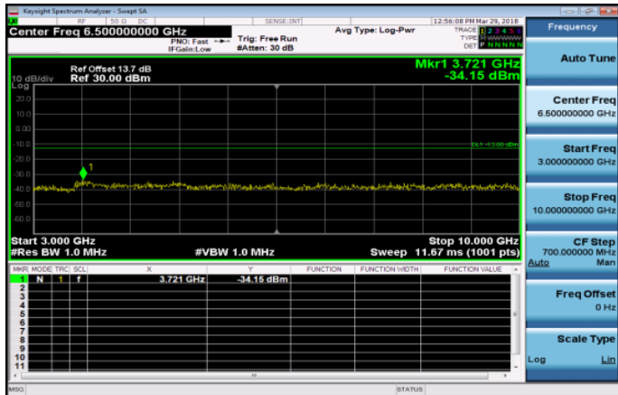
3GHz~10GHz_Band26_3MHz_QPSK_1_0_LowCH2680 5-825.5
