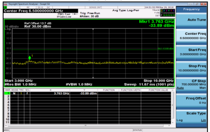
3GHz~10GHz_Band26_15MHz_QPSK_1_0_HighCH26 965-841.5
