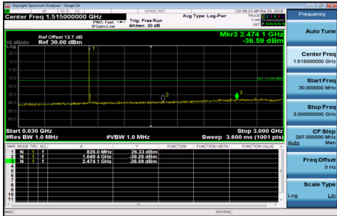
30MHz~3GHz_Band5_1_4MHz_QPSK_1_0_LowCH204 07-824.7
