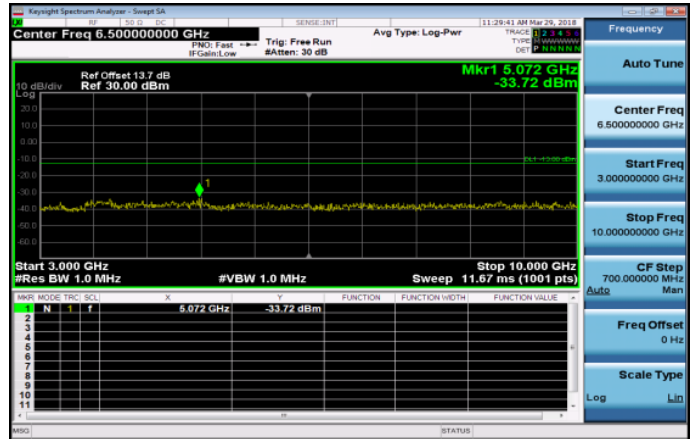
3GHz~10GHz_Band17_10MHz_QPSK_1_0_MidCH237 90-710
