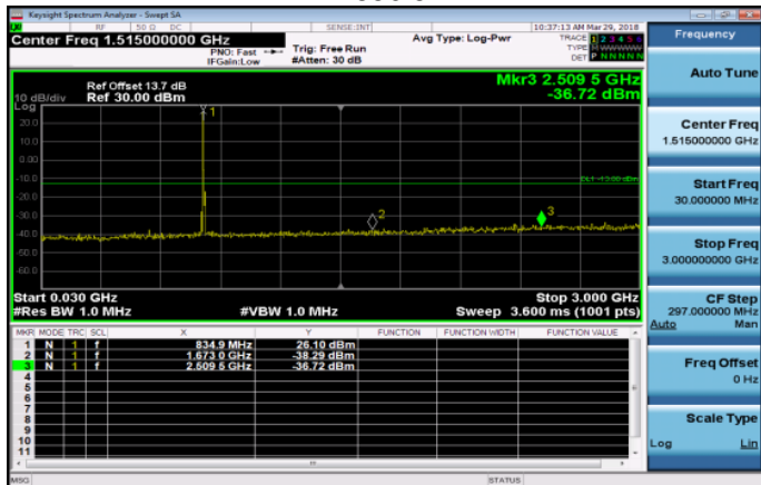
30MHz~3GHz_Band5_5MHz_QPSK_1_0_MidCH20525 -836.5
