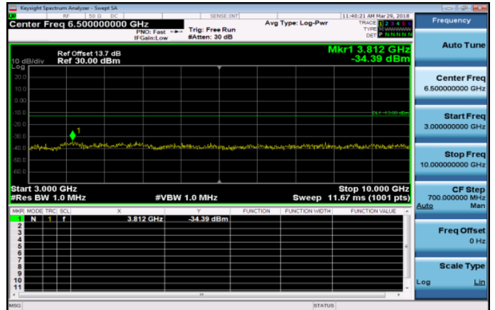
3GHz~10GHz_Band17_5MHz_QPSK_1_0_MidCH2379 0-710
