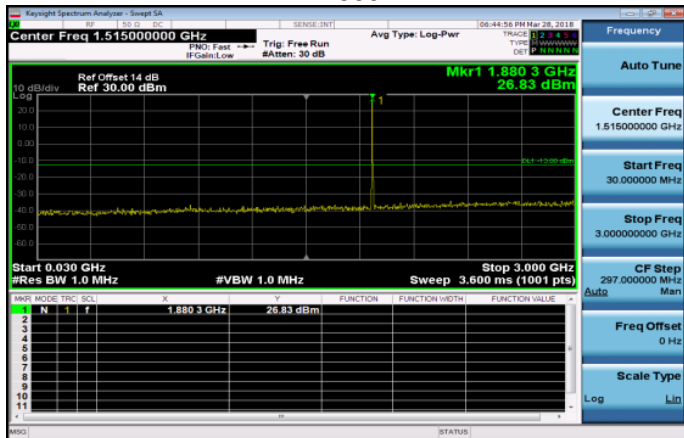
30MHz~3GHz_Band2_3MHz_QPSK_1_0_MidCH18900-1880
