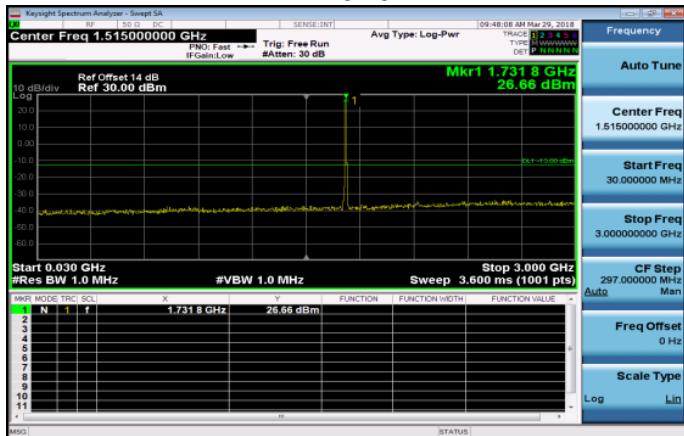
30MHz~3GHz_Band4_5MHz_QPSK_1_0_MidCH20175-1732.5
