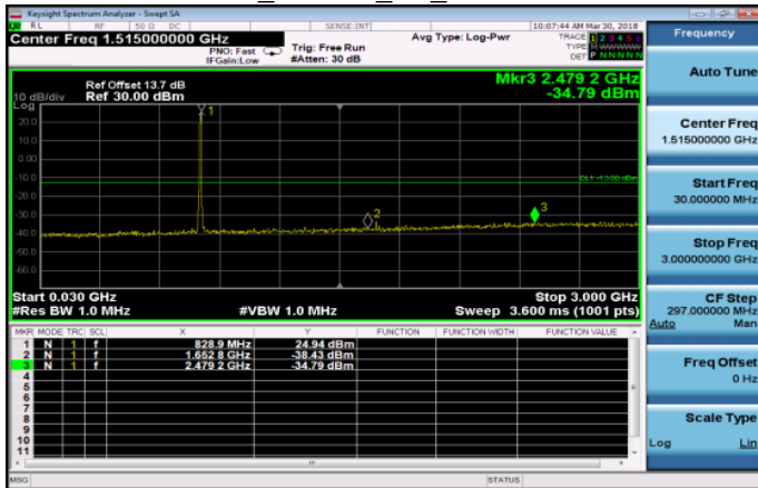
30MHz~3GHz_HSUPA_B5_LowCH4132-826.4
