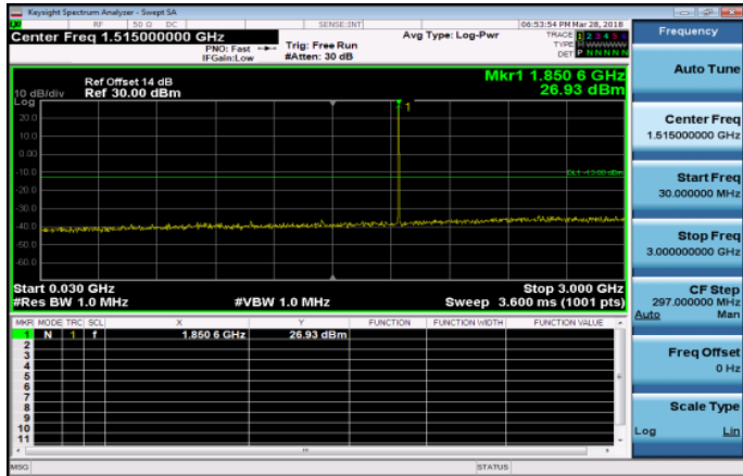
30MHz~3GHz_Band2_1_4MHz_QPSK_1_0_LowCH186 07-1850.7
