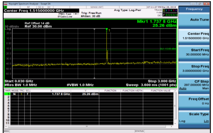
30MHz~3GHz_Band4_20MHz_QPSK_1_0_HighCH203 00-1745
