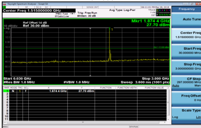
30MHz~3GHz_Band2_15MHz_QPSK_1_0_MidCH1890 0-1880
