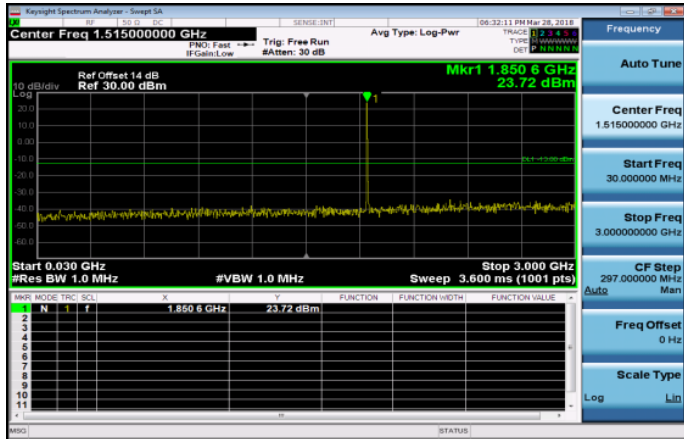
30MHz~3GHz_Band2_5MHz_QPSK_1_0_LowCH18625-1852.5
