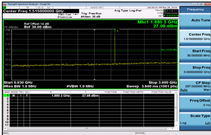
30MHz~3GHz_Band2_1_4MHz_QPSK_1_0_MidCH189 00-1880
