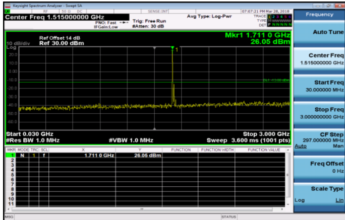
30MHz~3GHz_Band4_20MHz_QPSK_1_0_LowCH2005 0-1720
