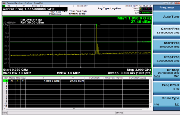
30MHz~3GHz_Band2_20MHz_QPSK_1_0_LowCH1870 0-1860
