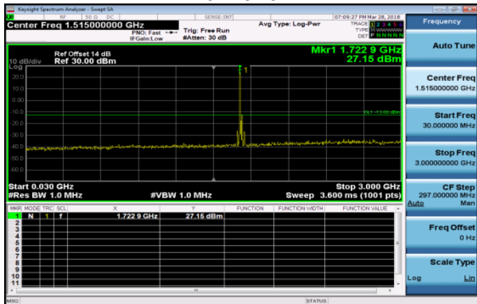
30MHz~3GHz_Band4_20MHz_QPSK_1_0_MidCH2017 5-1732.5
