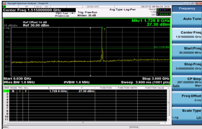
30MHz~3GHz_Band4_10MHz_QPSK_1_0_MidCH2017-5-1732.5
