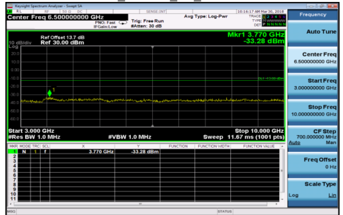
3GHz~10GHz_HSUPA_B5_MidCH4183-836.6
