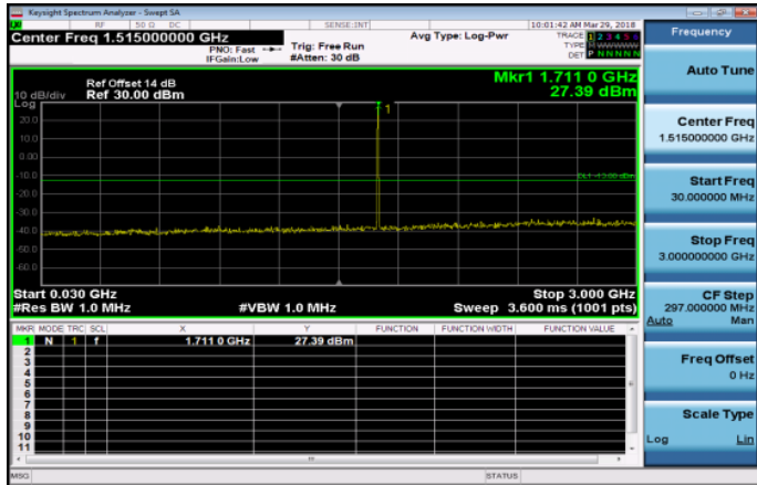
30MHz~3GHz_Band4_3MHz_QPSK_1_0_LowCH1965-1711.5
