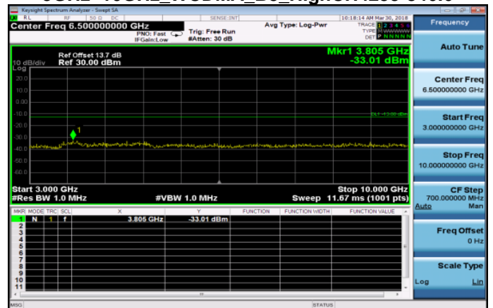
3GHz~10GHz_WCDMA_B5_HighCH4233-846.6
