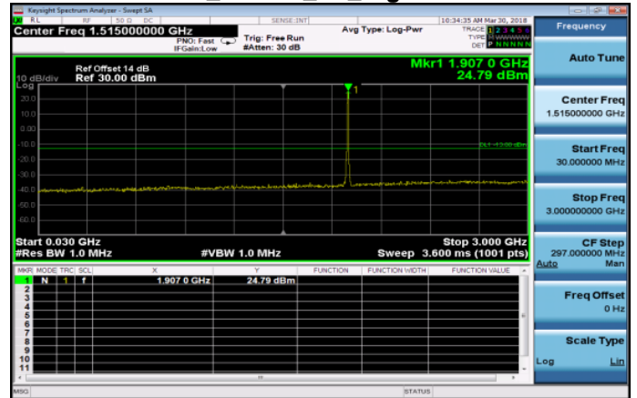
30MHz~3GHz_HSUPA_B2_HighCH9538-1907.6
