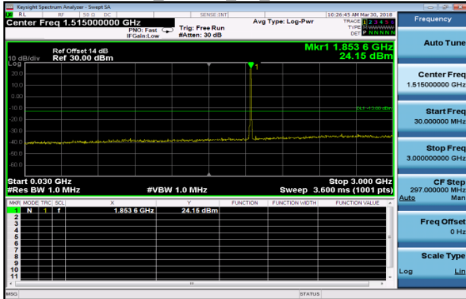
30MHz~3GHz_HSUPA_B2_LowCH9262-1852.4
