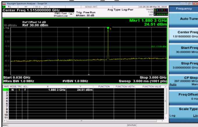
30MHz~3GHz_HSDPA_B2_MidCH9400-1880
