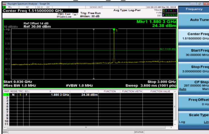
30MHz~3GHz_HSUPA_B2_MidCH9400-1880
