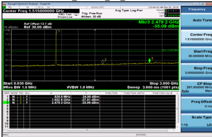
30MHz~3GHz_HSDPA_B5_LowCH4132-826.4
