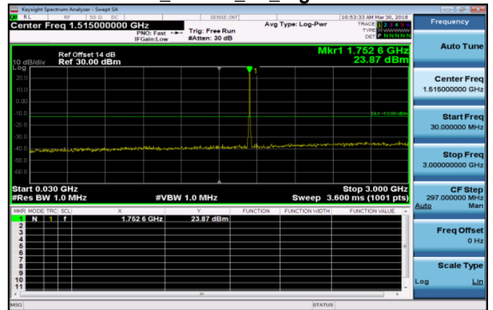
30MHz~3GHz_HSDPA_B4_HighCH1513-1752.6
