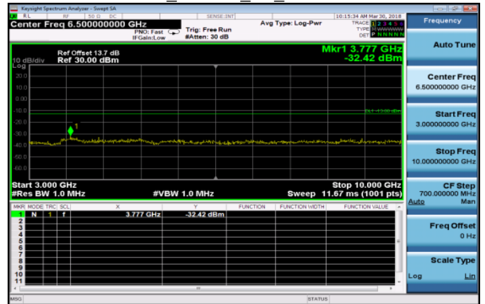
3GHz~10GHz_HSDPA_B5_MidCH4183-836.6
