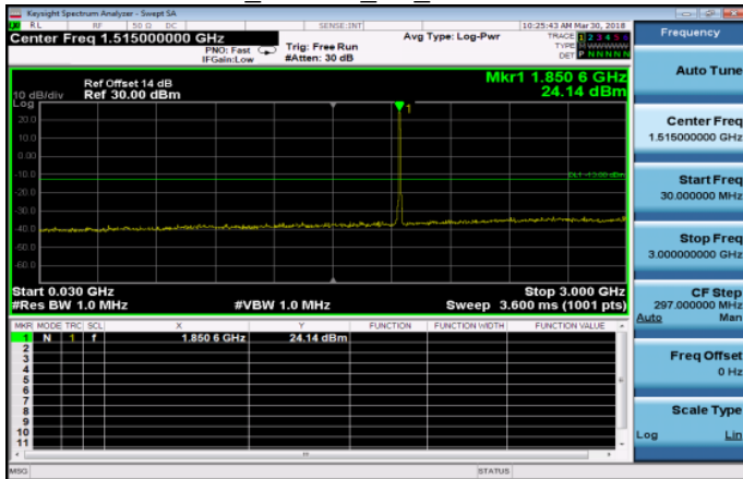
30MHz~3GHz_HSDPA_B2_LowCH9262-1852.4
