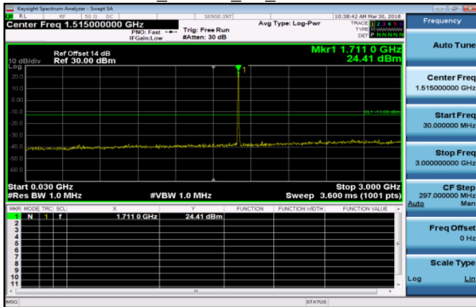
30MHz~3GHz_HSDPA_B4_LowCH1312-1712.4
