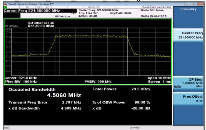
Part 90 Band26 5MHz 16QAM 25 0 HighCH26765-821.5
