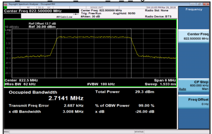
Part 90 Band26 3MHz 16QAM 15 0 HighCH26775-822.5
