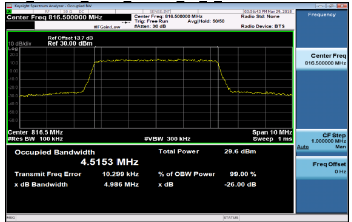
Part 90 Band26 5MHz 16QAM 25 0 LowCH26715-816.5
