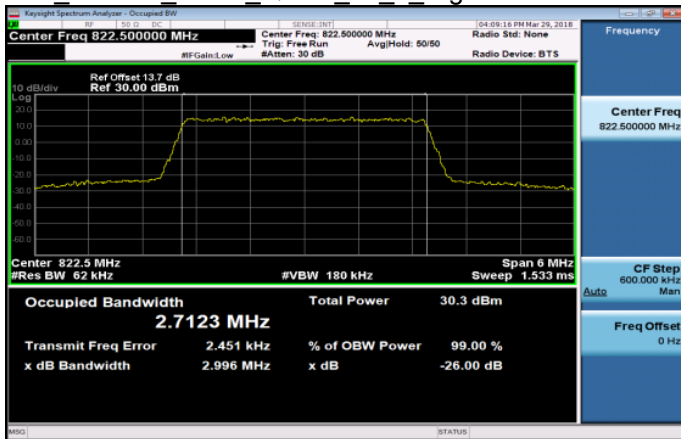
Part 90 Band26 3MHz QPSK 15 0 HighCH26775-822.5
