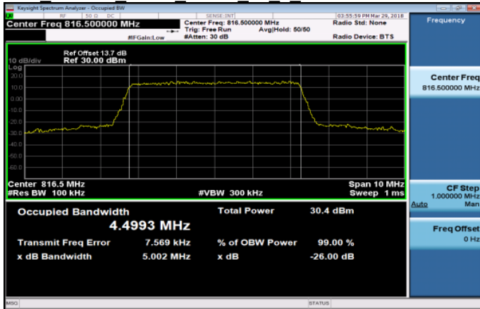
Part 90 Band26 5MHz QPSK 25 0 LowCH26715-816.5
