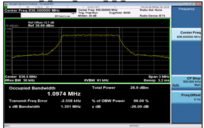
Band26 1 4MHz 16QAM 6 0 MidCH26915-836.5
