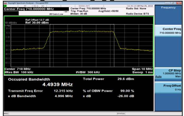
Band17 5MHz 16QAM 25 0 MidCH23790-710
