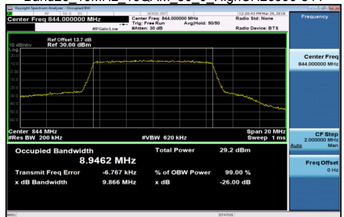
Band26 10MHz 16QAM 50 0 HighCH26990-844
