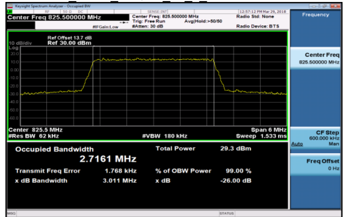
Band26 3MHz 16QAM 15 0 LowCH26805-825.5
