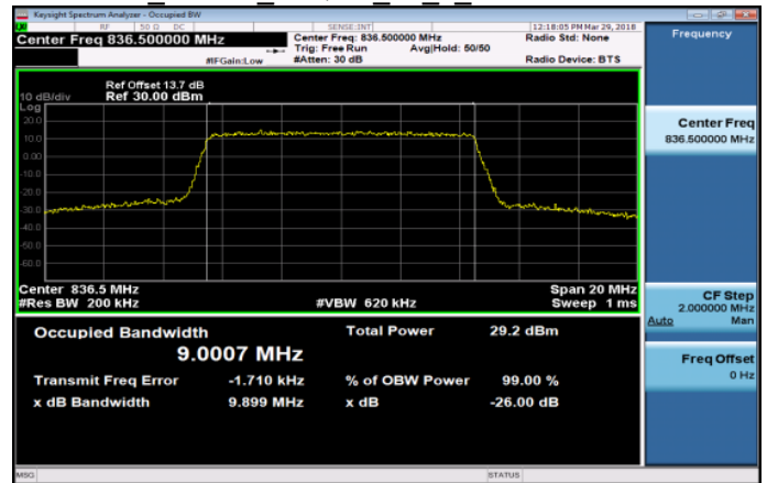
Band26 10MHz 16QAM 50 0 MidCH26915-836.5
