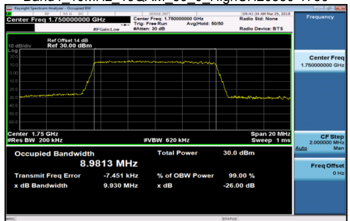
Band4_10MHz_16QAM_50_0_HighCH20350-1750
