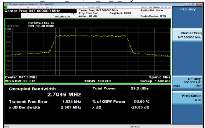
Band26 3MHz 16QAM 15 0 HighCH27025-847.5
