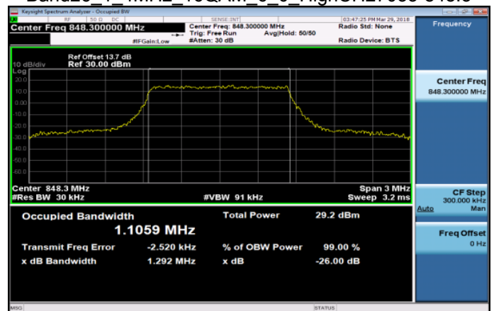
Band26 1 4MHz 16QAM 6 0 HighCH27033-848.3
