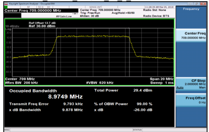
Band17 10MHz 16QAM 50 0 LowCH23780-709
