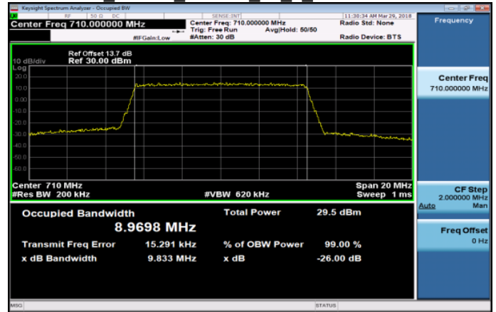
Band17 10MHz 16QAM 50 0 MidCH23790-710
