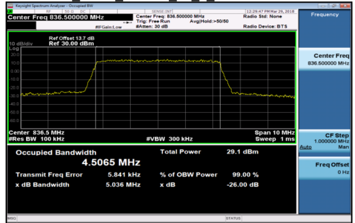
Band26 5MHz 16QAM 25 0 MidCH26915-836.5
