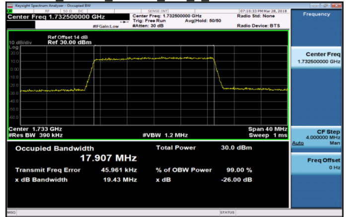
Band4 20MHz 16QAM 100 0 MidCH20175-1732.5
