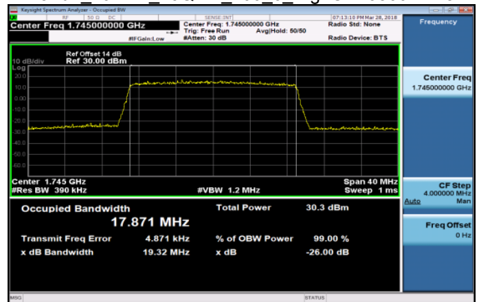
Band4 20MHz 16QAM 100 0 HighCH20300-1745
