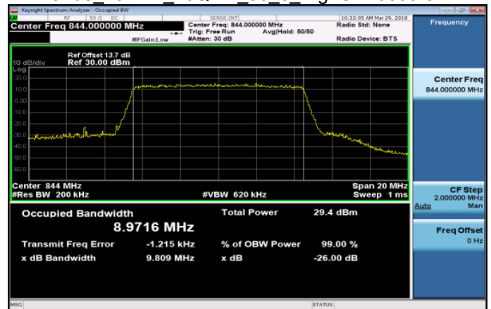
Band5_10MHz_16QAM_50_0_HighCH20600-844
