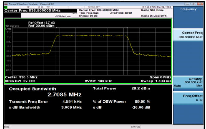
Band26 3MHz 16QAM 15 0 MidCH26915-836.5
