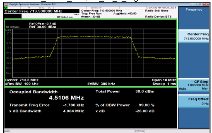
Band17 5MHz 16QAM 25 0 HighCH23825-713.5
