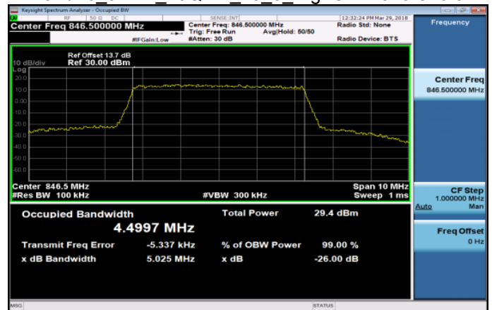
Band26 5MHz 16QAM 25 0 HighCH27015-846.5
