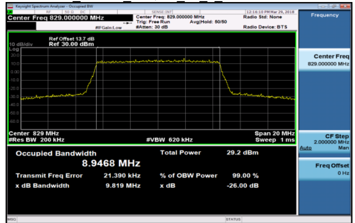
Band26 10MHz 16QAM 50 0 LowCH26840-829
