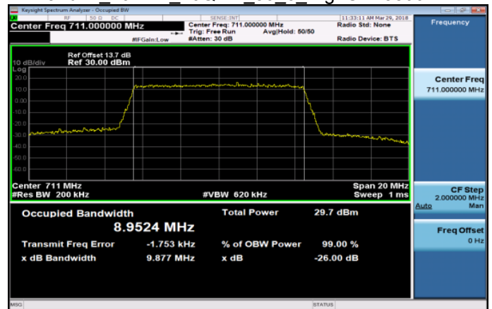
Band17 10MHz 16QAM 50 0 HighCH23800-711
