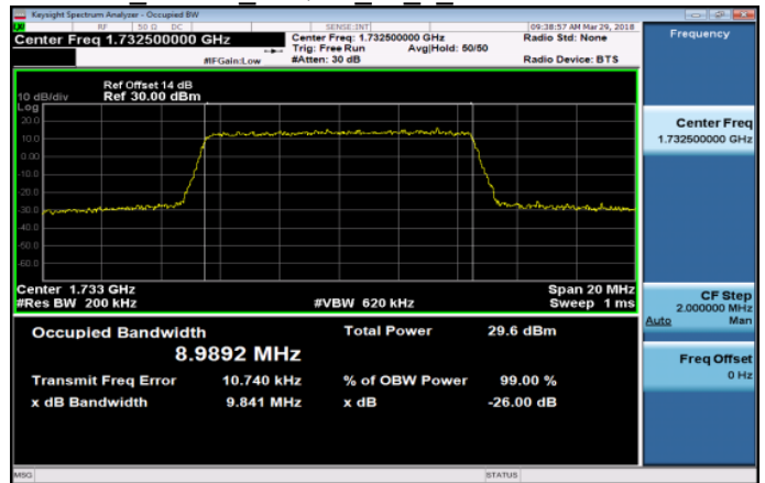
Band4_10MHz_16QAM_50_0_MidCH20175-1732.5
