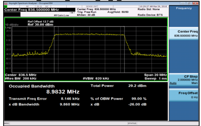
Band5_10MHz_16QAM_50_0_MidCH20525-836.5
