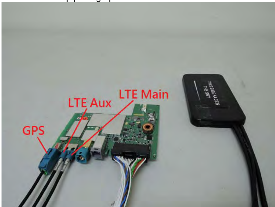
Setup photograph – 4G/3G/2G MIMO Antenna
