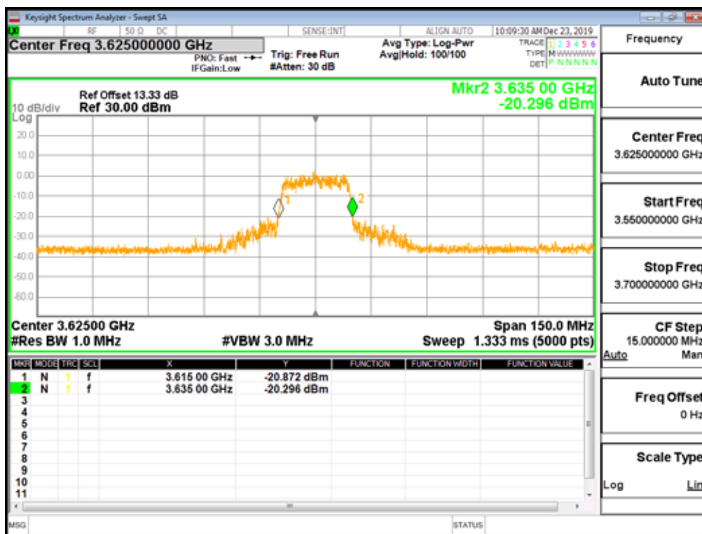
3625_20M_EIRP 20dBm_10s
