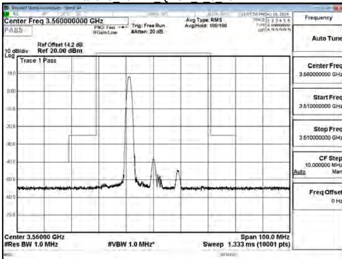
Band48 20MHz QPSK 1 0 Low-2
