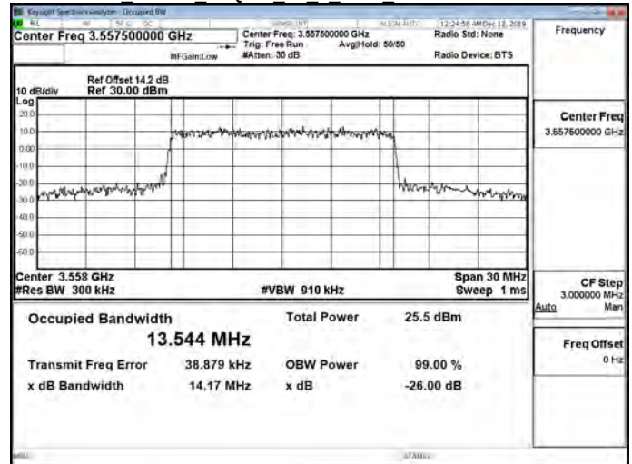
Band48 15MHz 16QAM 75 0 Main LowCH55315-3557.5
