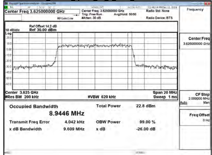
Band48 10MHz QPSK 50 0 Main MidCH55990-3625
