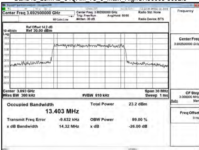
Band48 15MHz 64QAM 75 0 Main HighCH56665-3692.5
