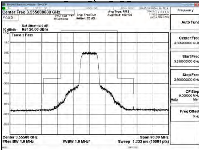
Band48 10MHz QPSK 50 0 Low-2
