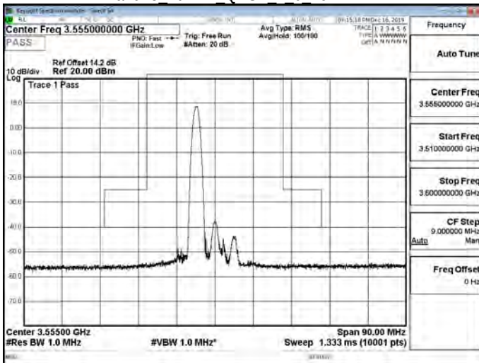
Band48 10MHz QPSK 1 0 Low-2
