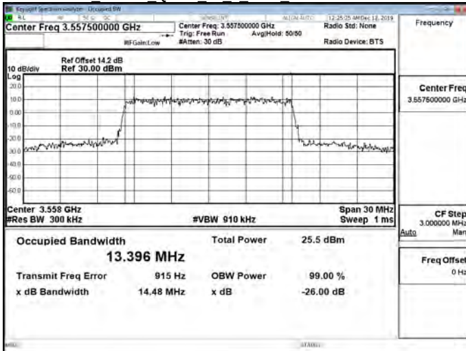
Band48 15MHz QPSK 75 0 Main LowCH55315-3557.5
