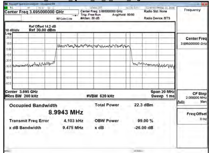
Band48 10MHz QPSK 50 0 Main HighCH56690-3695
