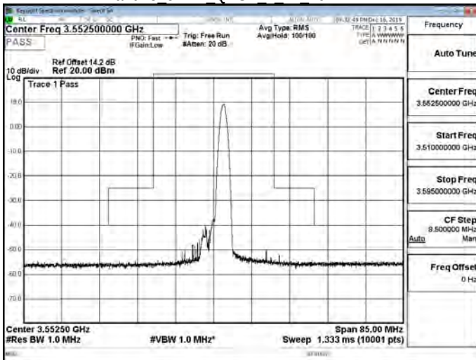
Band48 5MHz QPSK 1 24 Low-2
