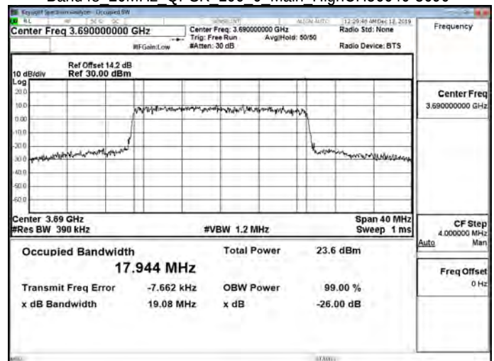
Band48 20MHz QPSK 100 0 Main HighCH56640-3690
