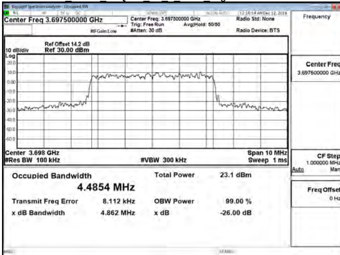
Band48 5MHz 64QAM 25 0 Main HighCH56715-3697.5
