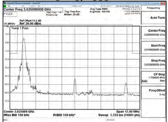
Band48 15MHz QPSK 1 0 Mid-2
