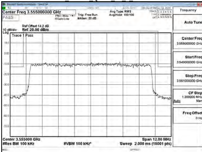
Band48 10MHz QPSK 50 0 Mid-1
