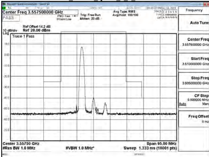
Band48 15MHz QPSK 1 0 Low-1
