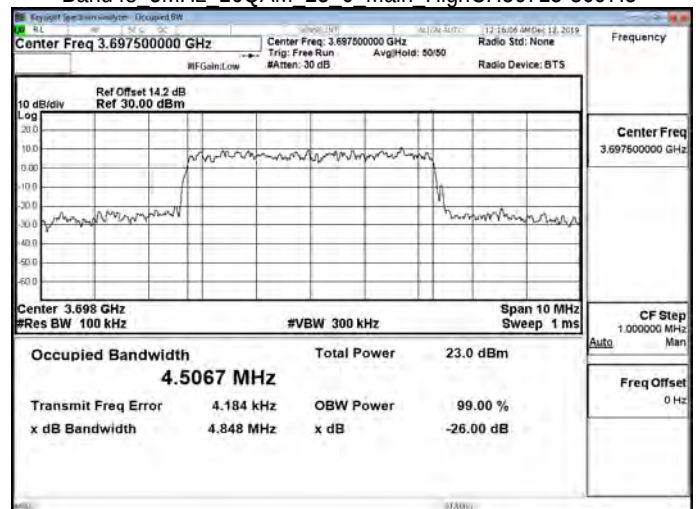
Band48 5MHz 16QAM 25 0 Main HighCH56715-3697.5
