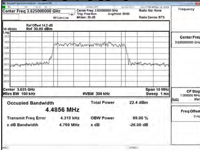
Band48 5MHz 64QAM 25 0 Main MidCH55990-3625
