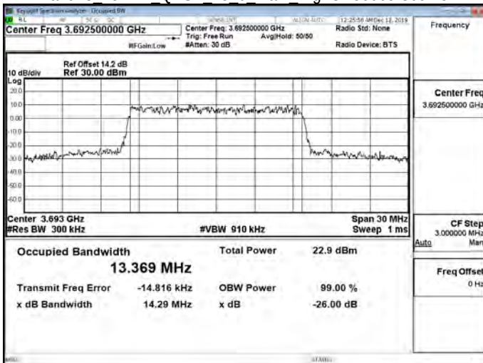
Band48 15MHz QPSK 75 0 Main HighCH56665-3692.5
