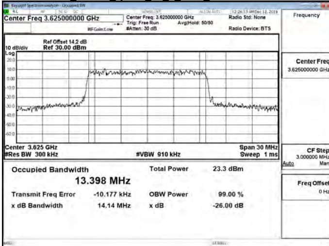
Band48 15MHz QPSK 75 0 Main MidCH55990-3625
